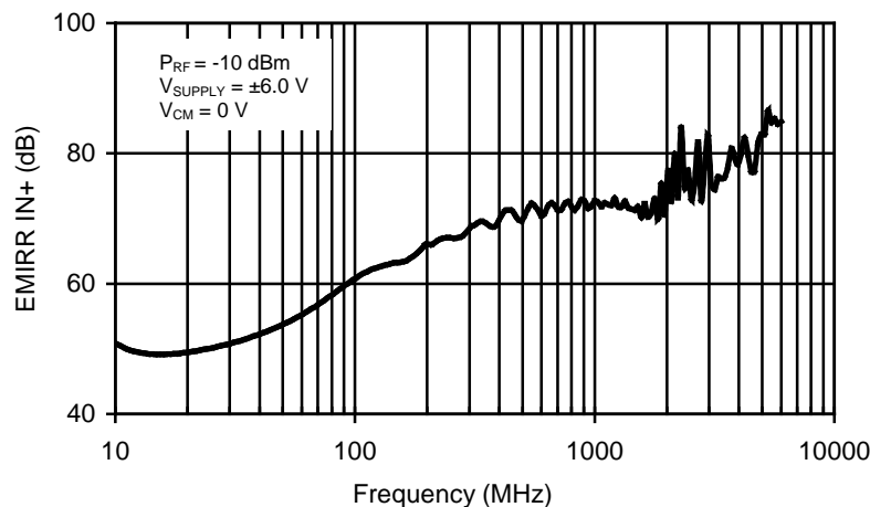
Figure 1. TLC2201 EMIRR IN+ vs Frequency
