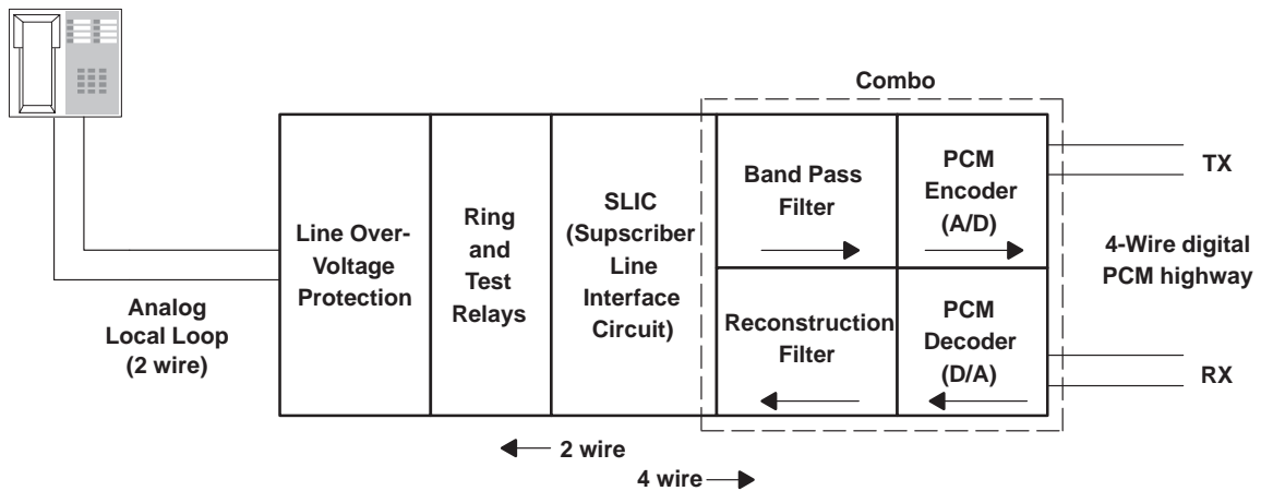
Figure 3. Line Card Block Diagram
