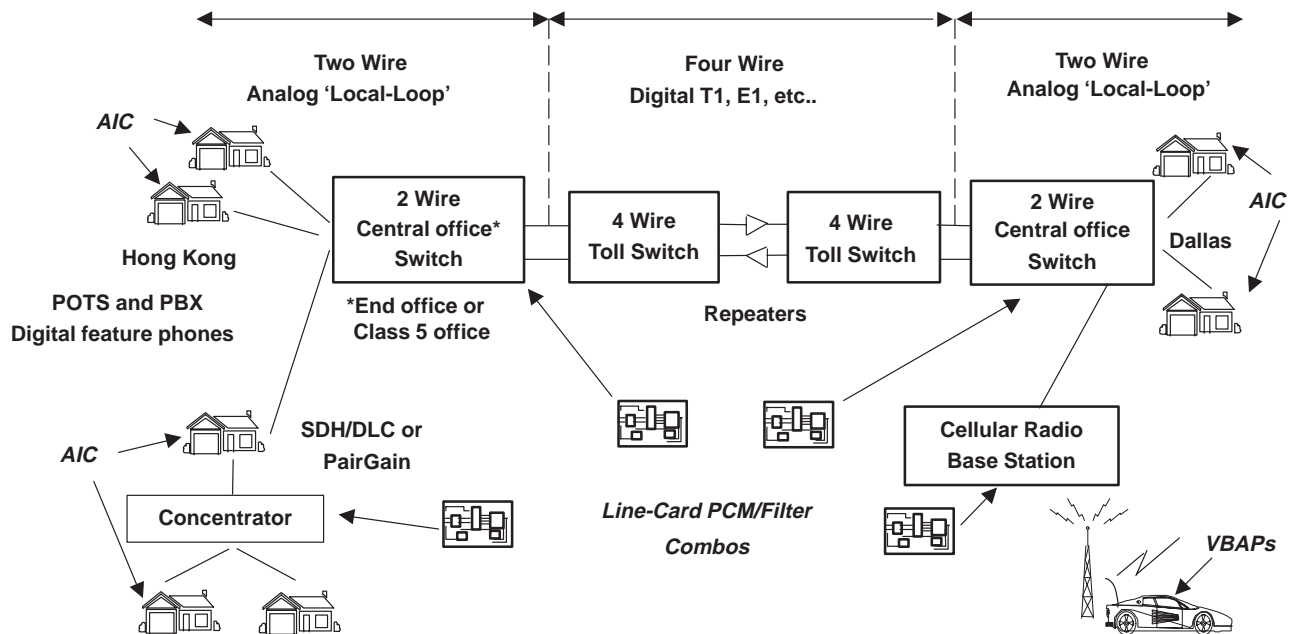
Figure 1. Voice-Band CODEC Applications
