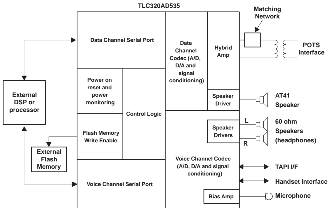
Figure 2. TLC320AD535 Block Diagram
