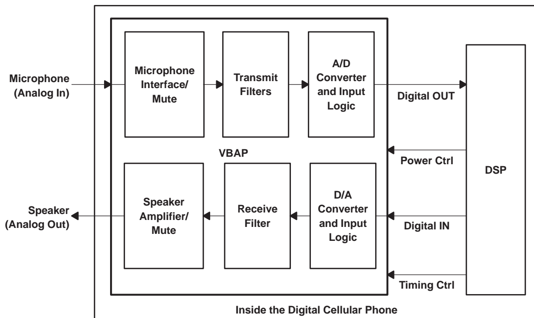
Figure 4. Voice-Band Audio Processor Application
