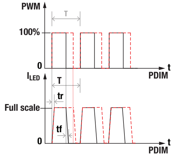
Figure 9. LED illumination with PWM dimming.
