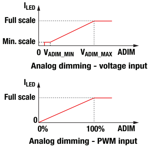
Figure 8. LED illumination with analog dimming.
