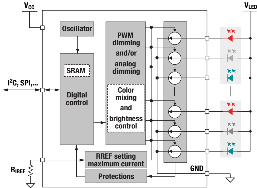
Figure 6. Typical block diagram of an LED animation driver.
