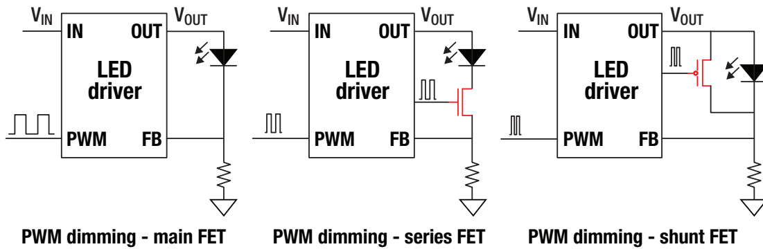
Figure 10. LED illumination PWM dimming methods.
