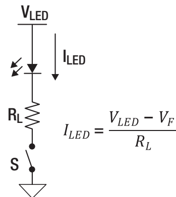
Figure 3. An LED driving circuit with a current-limiting resistor.
