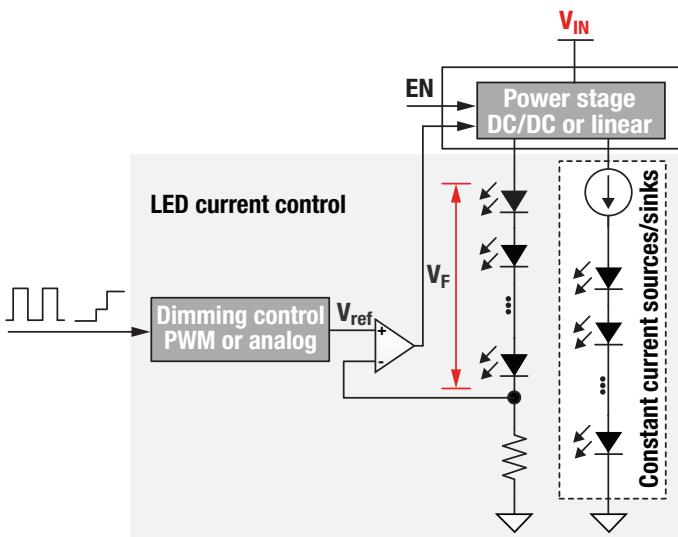
Figure 7. Typical block diagram for LED illumination.
