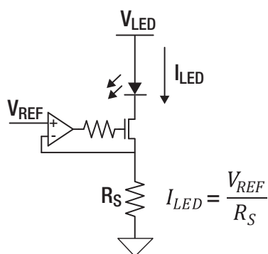
Figure 4. An LED driving circuit with constant current.
