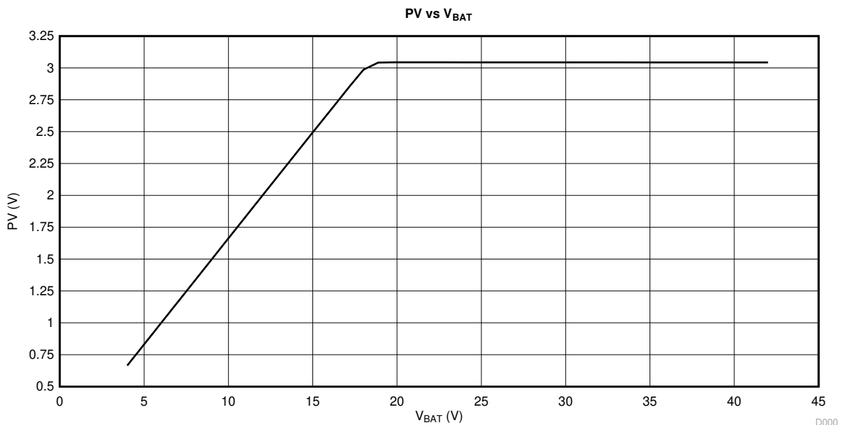
Figure 8-10. V_{BAT} vs PV for 3.3 V
