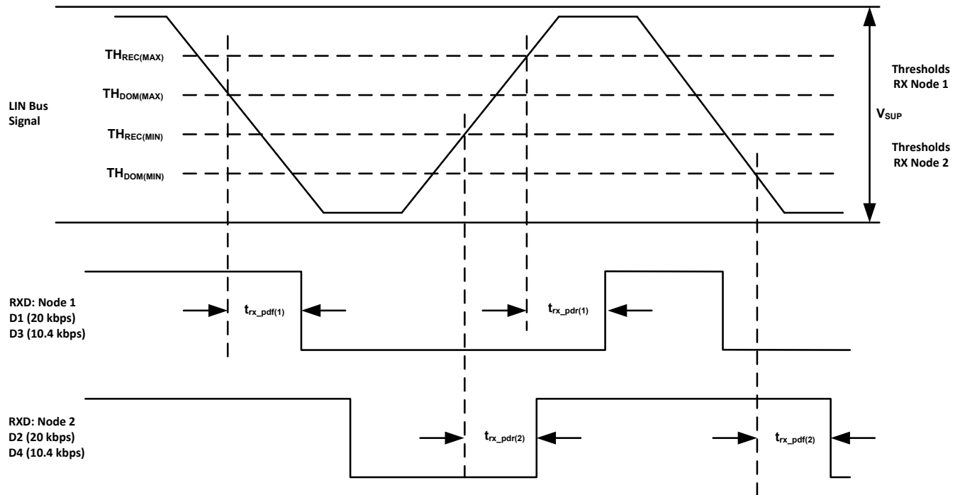
Figure 7-4. Propagation Delay
