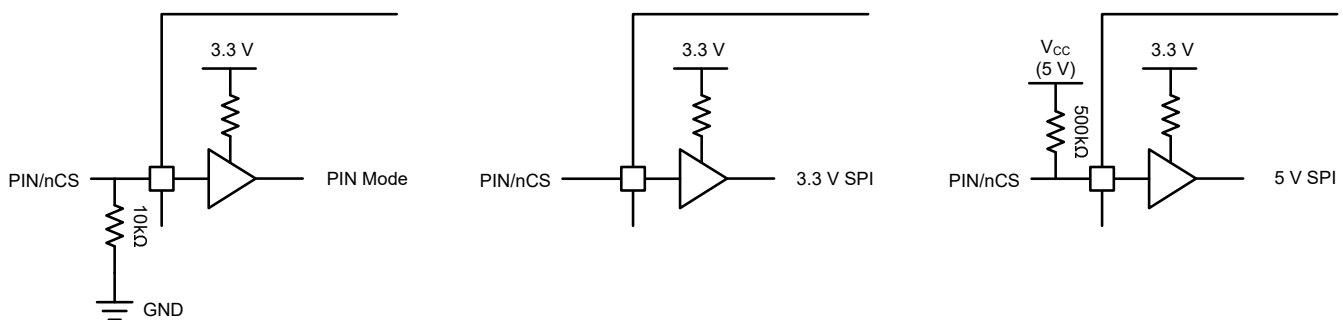
Figure 8-4. PIN/nCS configuration
