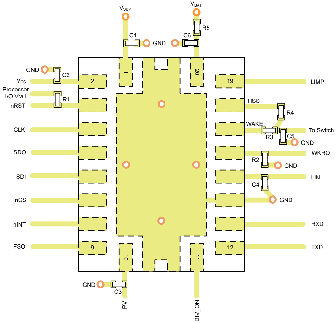
Figure 9-5. Layout Example
