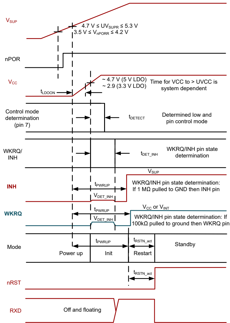
Figure 8-5. Power up timing diagram for pin 7 connected to ground
