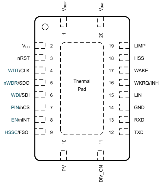
Figure 5-1. RGY Package, 20-Pin QFN (Top View)
