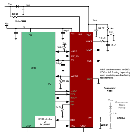
Simplified Schematics, Pin Control
