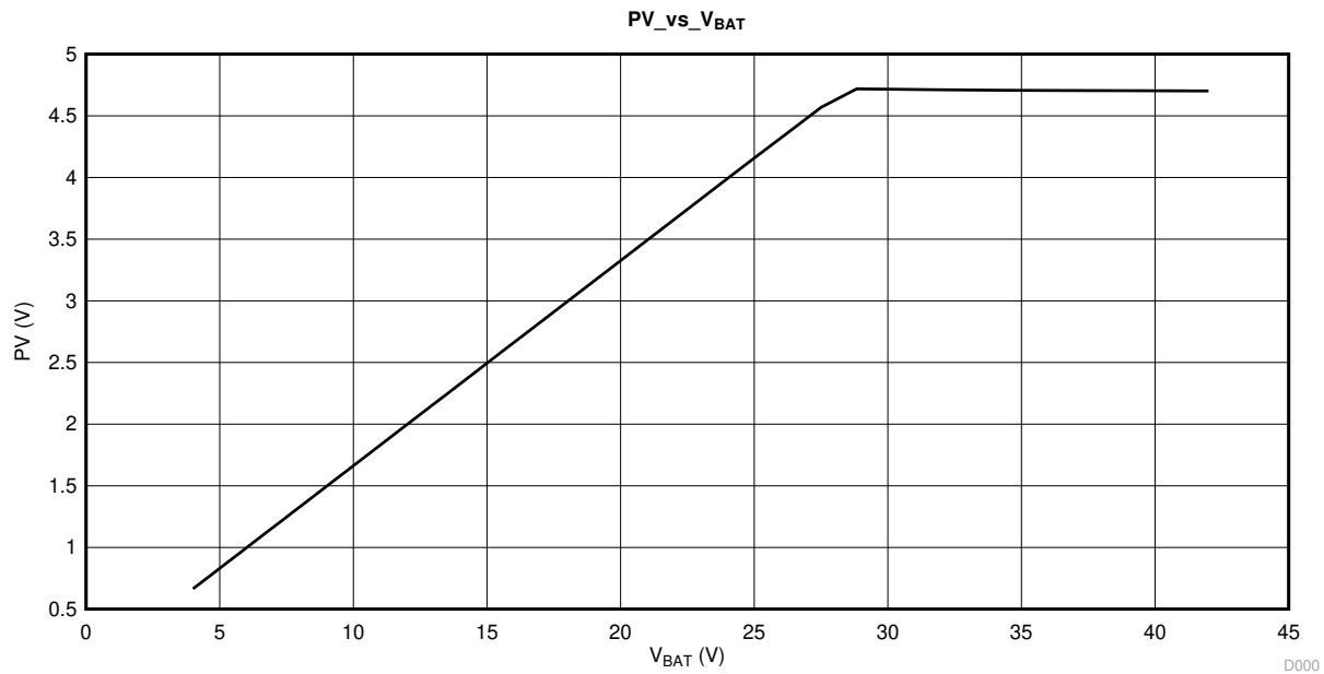
Figure 8-9. V_{BAT} vs PV for 5 V
