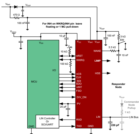
Simplified Schematics, SPI Control
