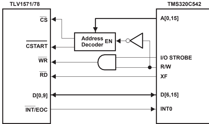
Figure 1. ADC-DSP Interface
