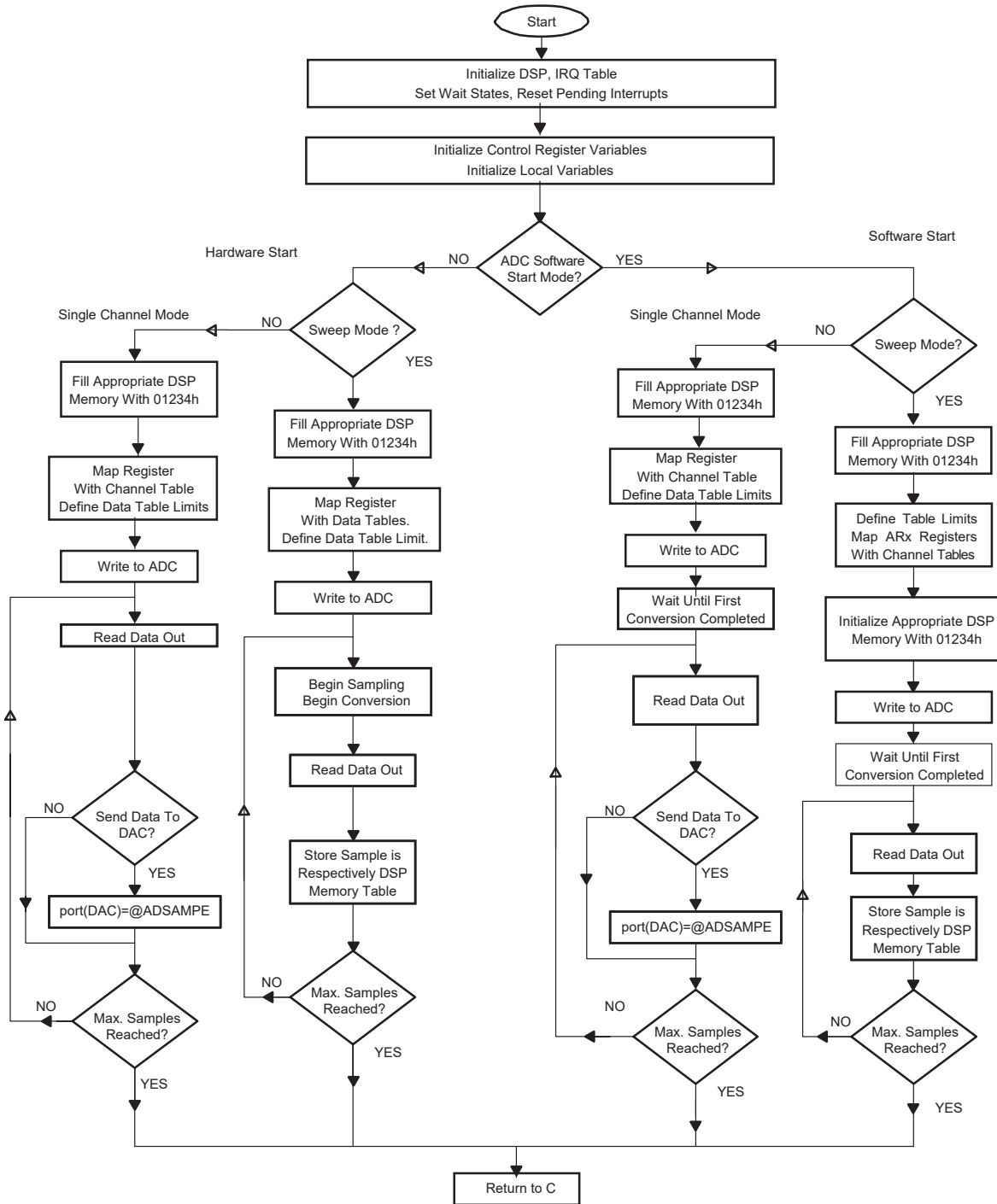
Figure 8. Software Flow Chart
