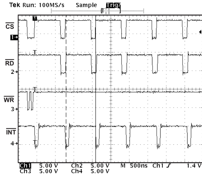
Figure 5. Software Start Configuration Cycle With INT
