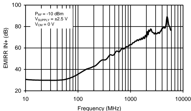
Figure 1. TLV2262 EMIRR IN+ vs Frequency
