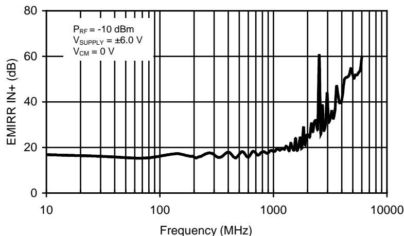
Figure 1. TLV2381 EMIRR IN+ vs Frequency
