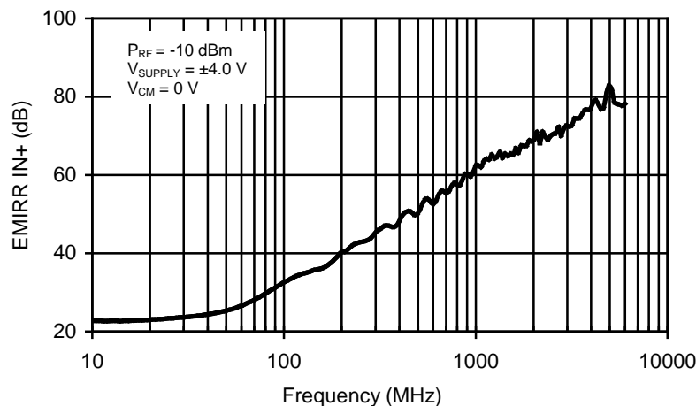
Figure 1. TLV2432 EMIRR IN+ vs Frequency
