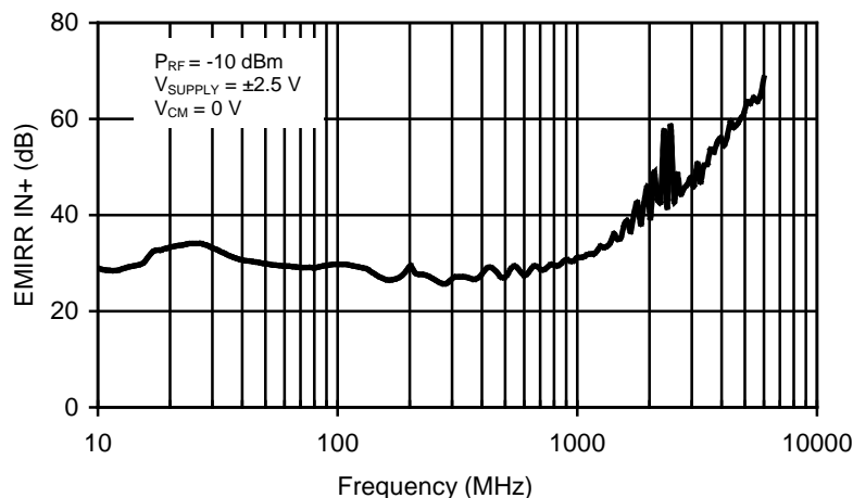
Figure 1. TLV2621 EMIRR IN+ vs Frequency
