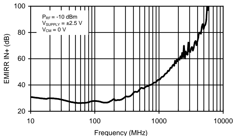
Figure 1. TLV2631 EMIRR IN+ vs Frequency
