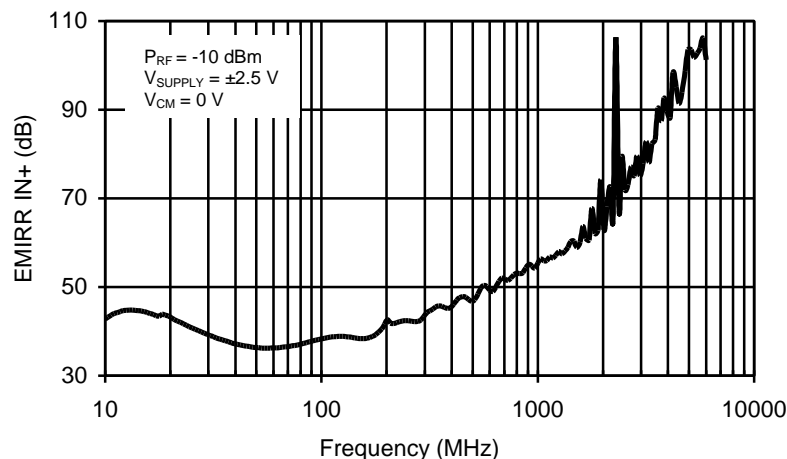
Figure 1. TLV2771 EMIRR IN+ vs Frequency
