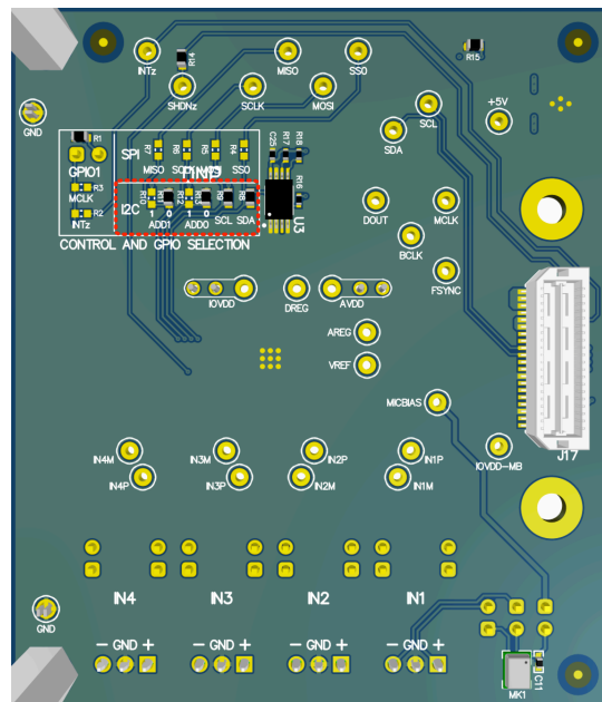
Figure 18. I 2 C Address Configuration for the TLV320ADx140 EVM
