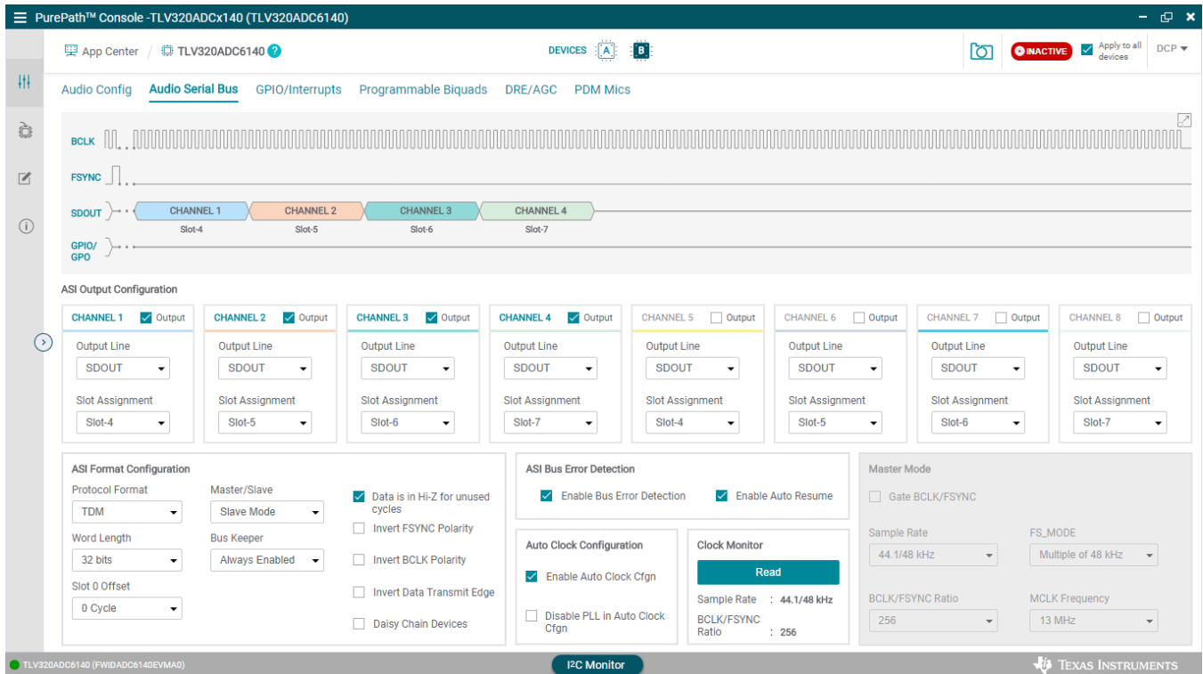
Figure 22. PurePath Console Device B Channel to Slot Mapping
