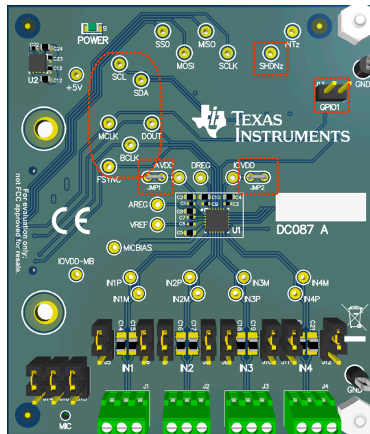
Figure 17. Location of TLV320ADCx140 EVM I 2 C and TDM signals
