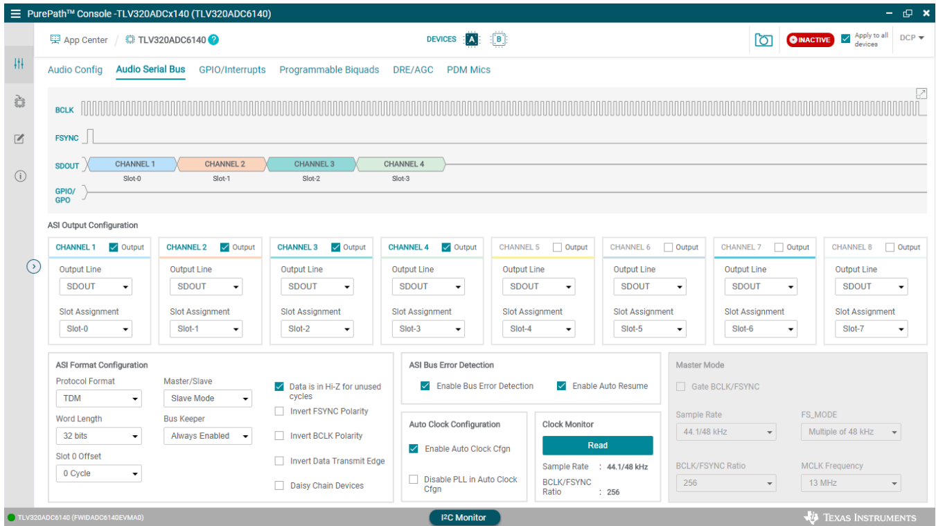
Figure 21. PurePath Console Device A Channel to Slot Mapping
