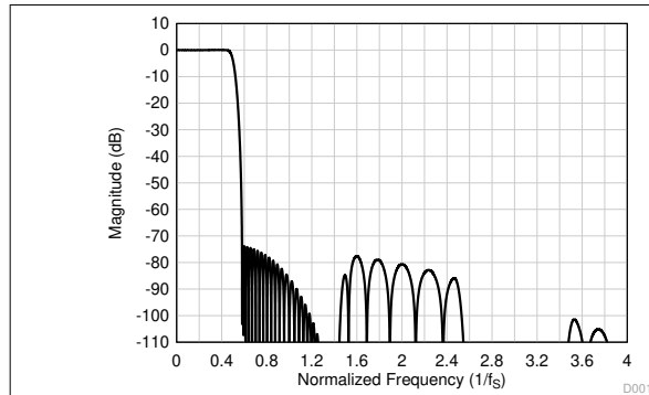
Figure 8-25. Linear Phase Decimation Filter Magnitude Response
