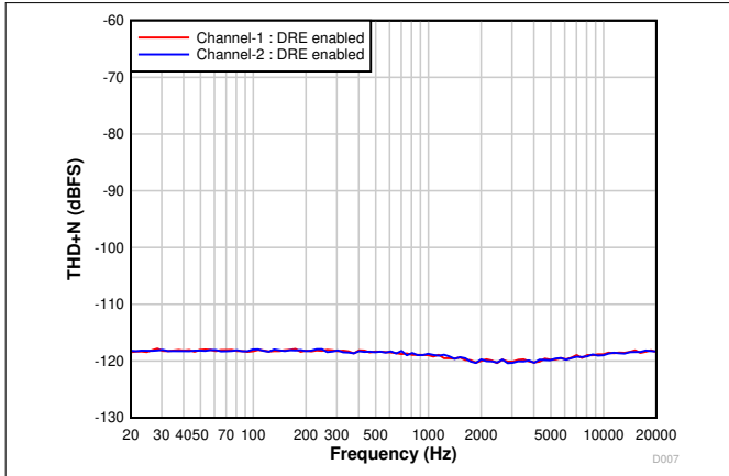
Figure 7-10. THD+N vs Input Frequency With a -60-dBr Input
