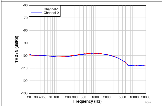
Figure 7-10. THD+N vs Input Frequency With a -60-dBr Input
