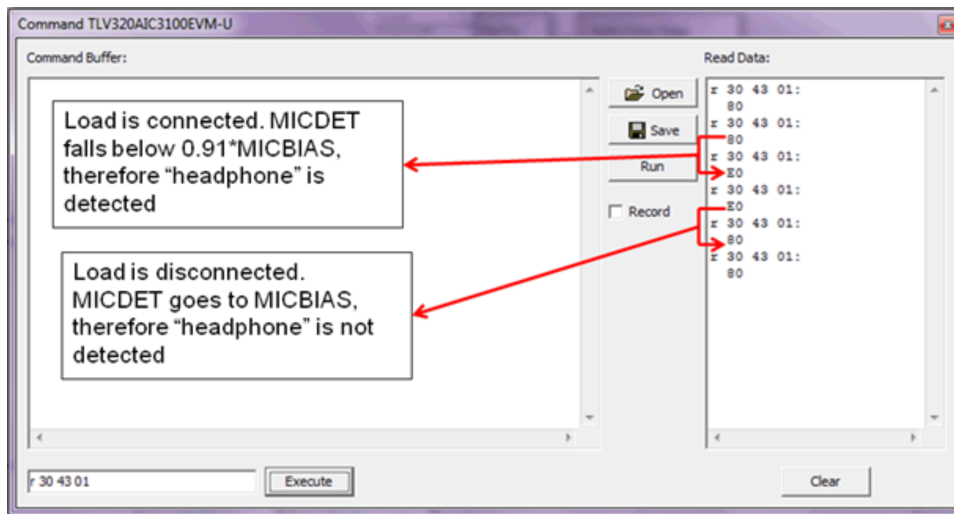
Figure 3. Register Values From the Command Prompt
