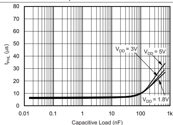
Figure 8. Propagation Delay ( t_{PHL} ) vs Capacitive Load
