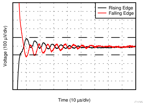
Figure 6-26. Settling Time
