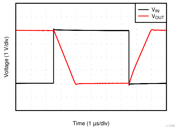
Figure 6-25. Large-Signal Step Response (4-V Step)
