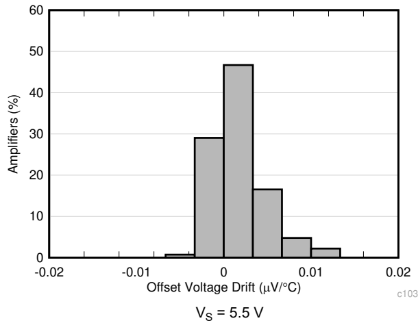
Figure 6-1. Offset Voltage Drift Distribution
