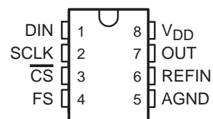
D, DGK, OR P PACKAGE (TOP VIEW)
