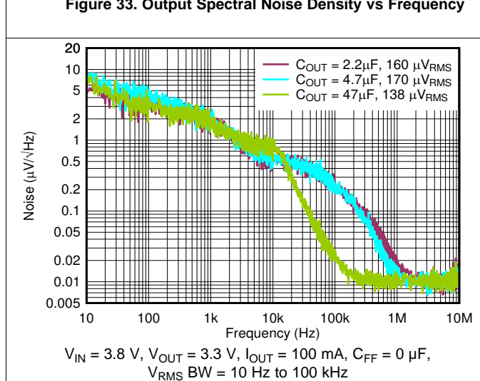
Figure 35. Output Spectral Noise Density vs Frequency and C_{OUT}
