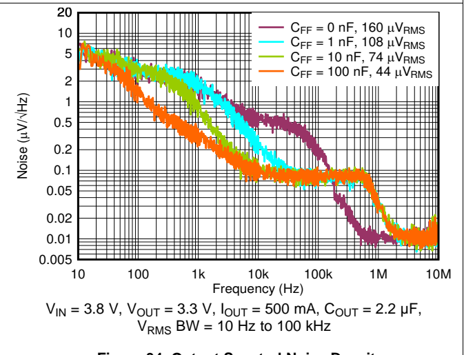
Figure 34. Output Spectral Noise Density vs Frequency and C_{FF}
