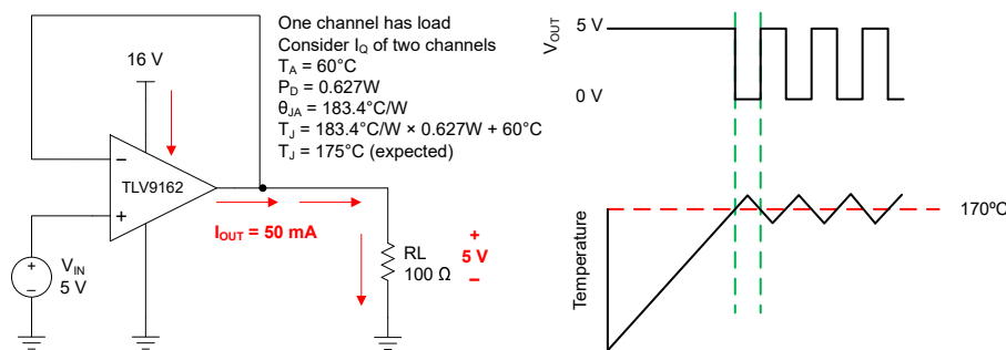
Figure 7-4. Thermal Protection
