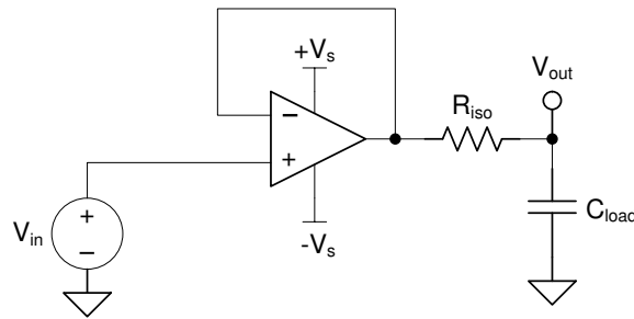
Figure 7-7. Extending Capacitive Load Drive With the TLV9161
