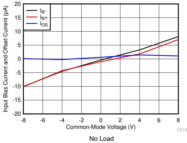
Figure 6-13. Input Bias Current and Offset Current vs Common-Mode Voltage
