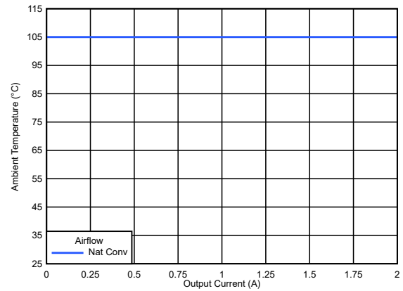
The device is soldered to a 64-mm × 83-mm, 4-layer PCB. Figure 7-10. Safe Operating Area (All V_{OUT} )
