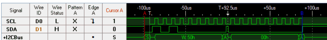
Figure 9. I2C Transaction for I2C_MASTER_CMD_BURST_SEND_START
