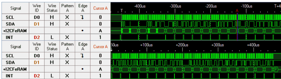
Figure 17. Receive With CPU and Non FIFO
