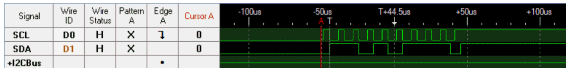
Figure 15. I2C Transaction for I2C_MASTER_CMD_BURST_RECEIVE_FINISH
