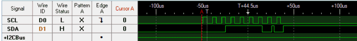
Figure 14. I2C Transaction for I2C_MASTER_CMD_BURST_RECEIVE_CONT
