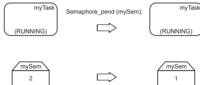
Figure 13. Task Continues to Run After Semaphore_Pend()
