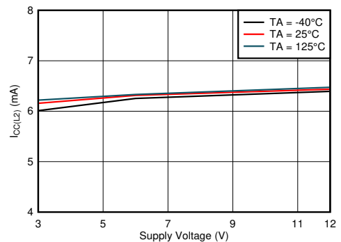
Figure 7-28. I_{CC(L2)} vs V_{CC}
