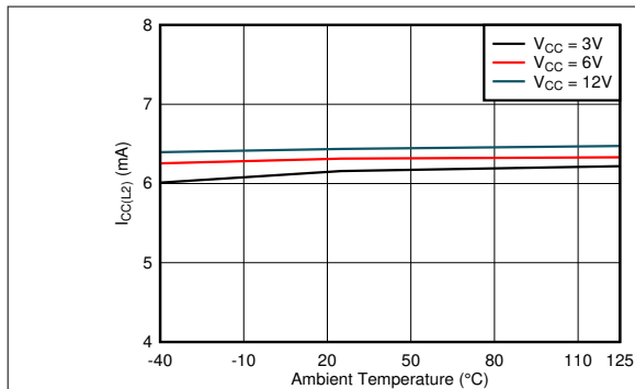
Figure 7-27. I_{CC(L2)} vs Temperature
