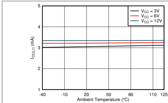
Figure 7-25. I_{CC(L1)} vs Temperature
