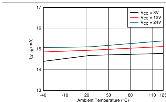
Figure 7-29. I_{CC(H)} vs Temperature
