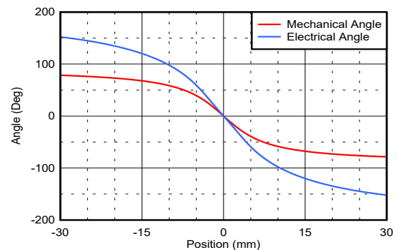
Figure 7. Measured Angle vs. Position
