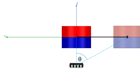
Figure 5. Slide-By Mechanical Angle
