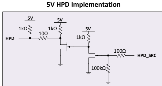
Figure 60. TMDS171 in Sink Side Application, 5 V HPD Implementation
