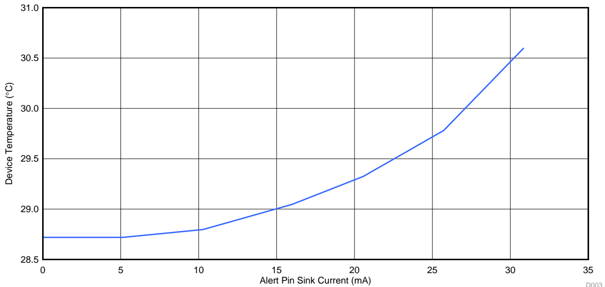
Figure 10. TMP107 Self Heating Effect vs Alert Pin Sink Current. V+ = 3.3 V
