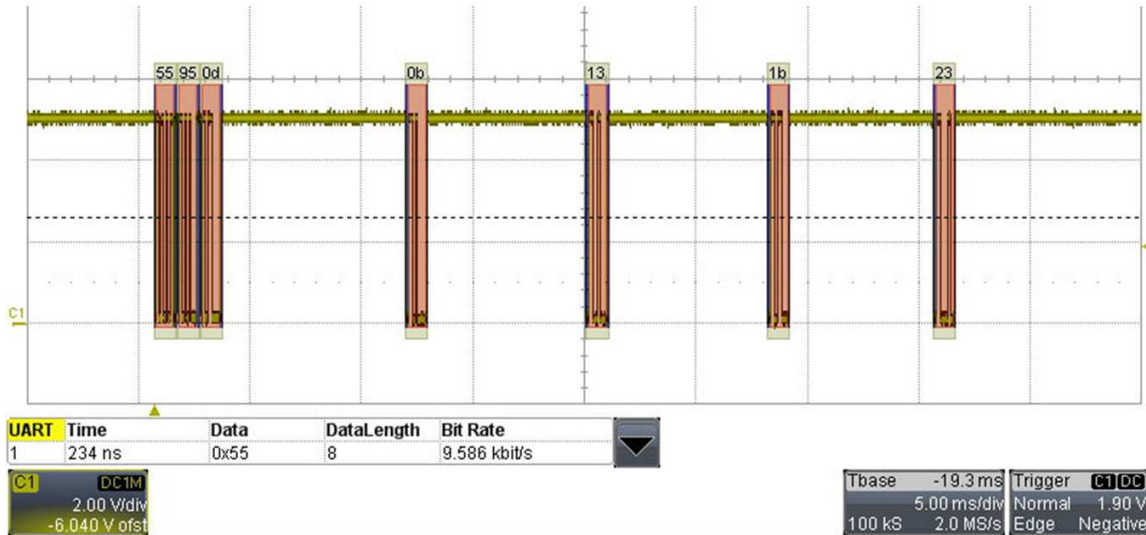
Figure 11. Oscilloscope of 4 Parts Chain Initialization Signal
