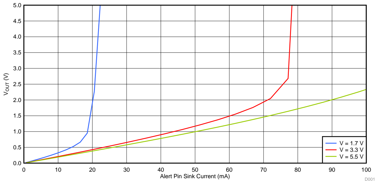
Figure 8. Alert Pin Output Voltage vs Sink Current: Temperature = 25°C
