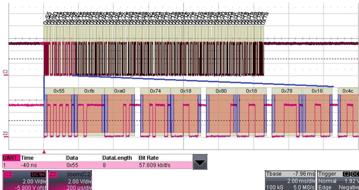
Figure 3. Oscilloscope of 32 Device Chain Global Temperature Data Read Event
