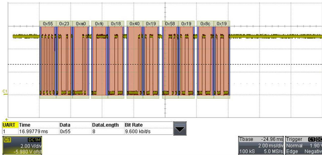
Figure 1. Oscilloscope of Global Read Command in Continuous Conversion Mode
