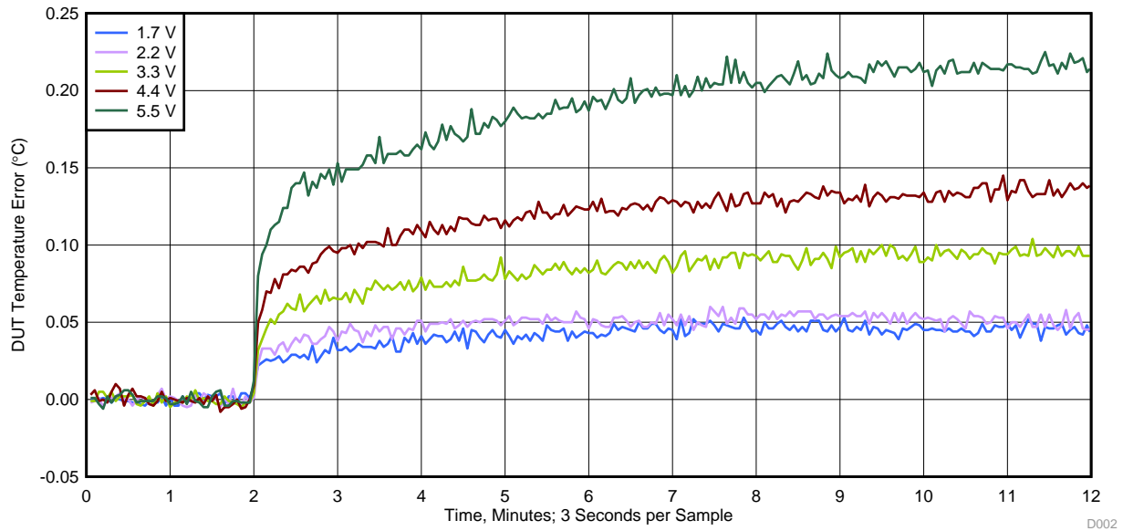
Figure 9. TMP107 Self-Heating Effect vs Supply Voltages: Temperature = 25°C
