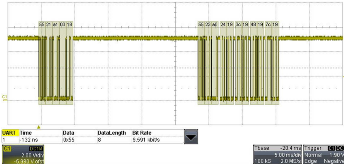
Figure 2. Oscilloscope of Temperature Data Collection in One Shot Mode for 4 Parts Chain
