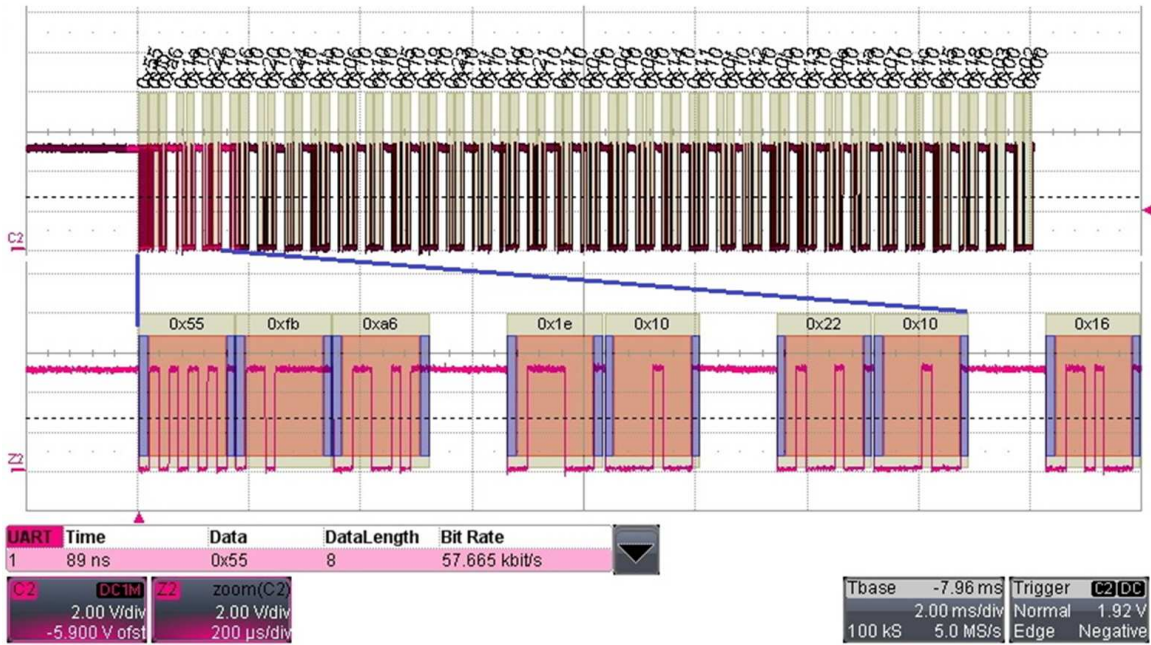
Figure 4. Oscilloscope of 32 Device Chain Global EEPROM Cell-1 Data Read Event
