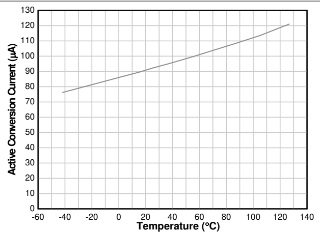
Figure 6-9. Active Conversion Current vs Temperature
