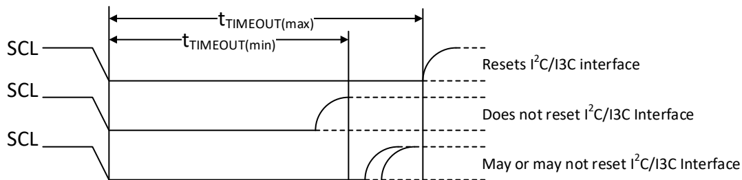
Figure 7-4. I 2 C or I 3 C Basic Bus Reset
