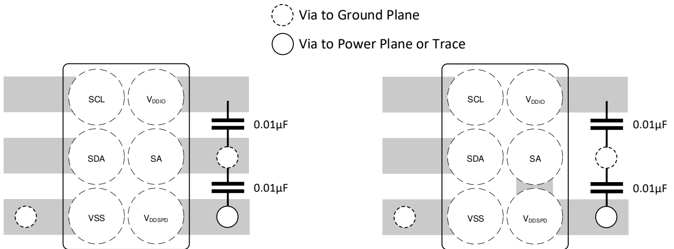
Figure 10-1. Layout Example
