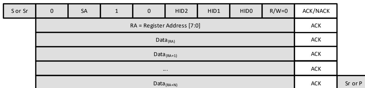
Figure 7-6. I 2 C Write Operation
