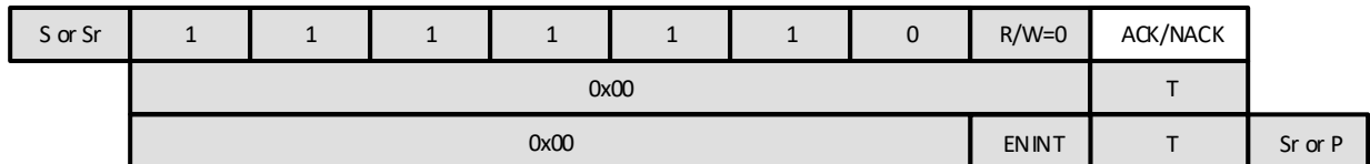
Figure 7-25. ENEC CCC Broadcast
