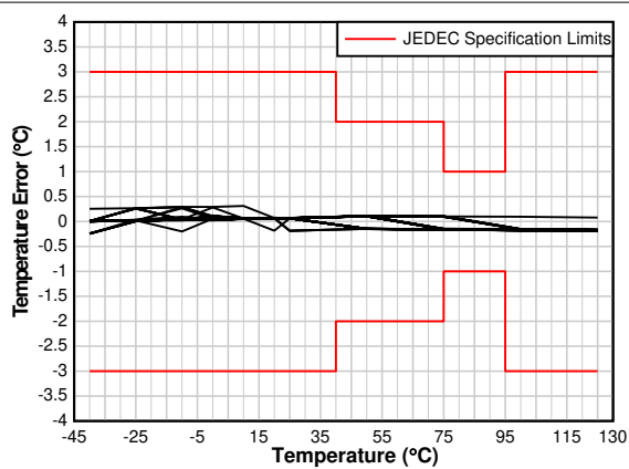
Figure 6-8. Temperature Error vs Temperature
