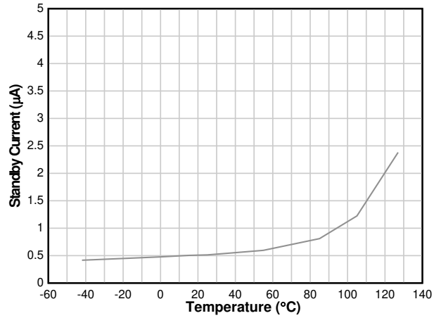
Figure 6-11. Standby Current vs Temperature
