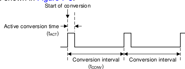
Figure 7-5. Continuous Conversion Timing Diagram
