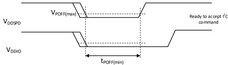
Figure 7-3. Power-Down and Reset Sequence
