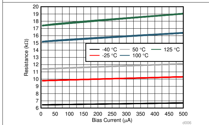
Figure 5. Supply Dependence Resistance vs. Bias Current
