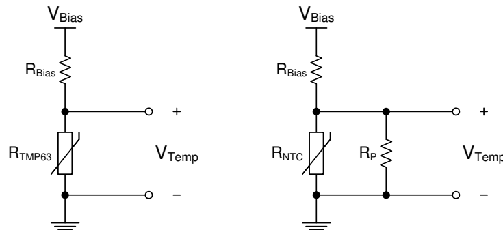
Figure 8-7. TMP63-Q1 vs. NTC With Linearization Resistor ( R_{\text{P}} ) Voltage Divider Circuits
