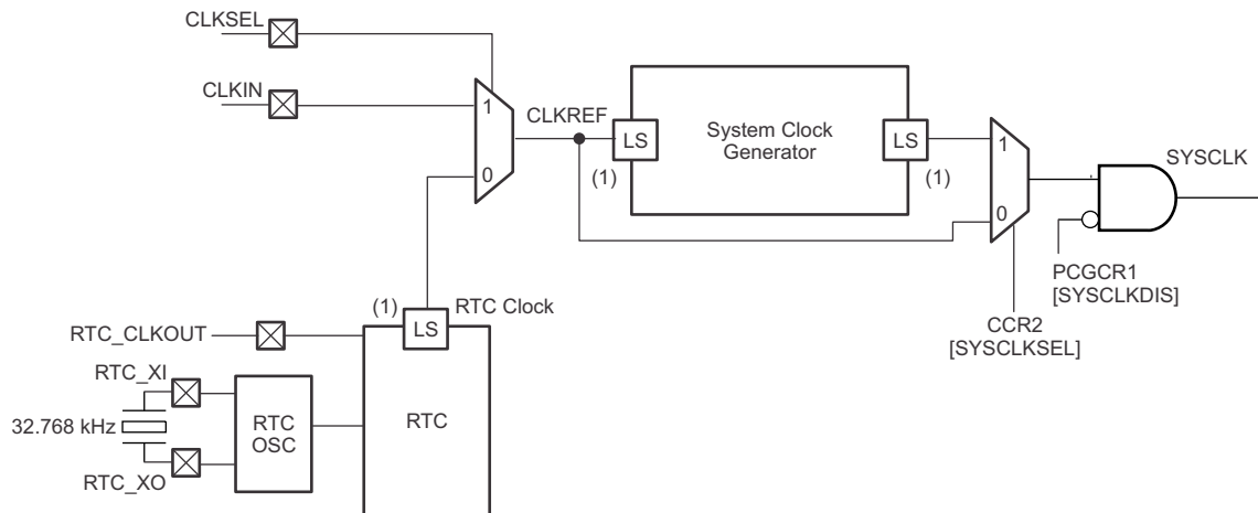
Figure 1. System Clock Generation - C55x5
