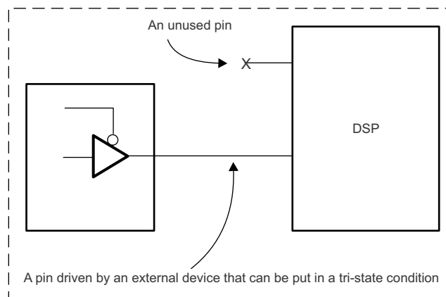
Figure 7. Unused Pins
