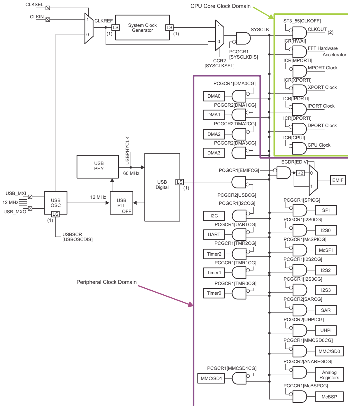
Figure 4. C5517 Clock Diagram
