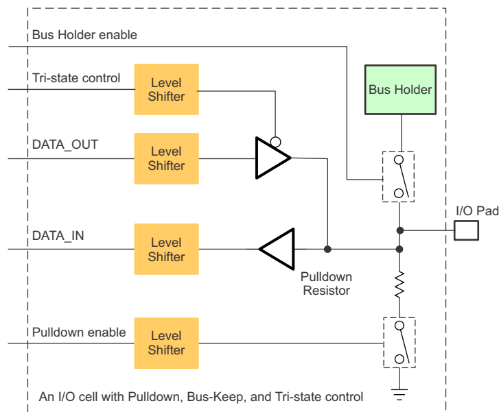
Figure 8. Typical I/O Cell
