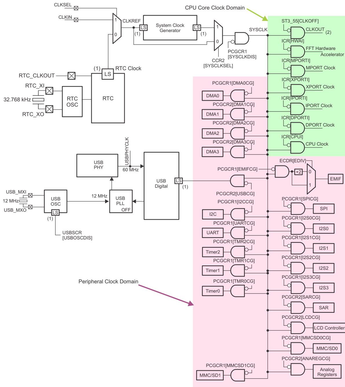
Figure 3. C55x5 Clock Diagram
