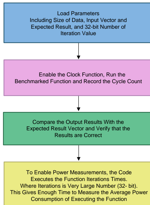
Figure 1. Algorithm Flow
