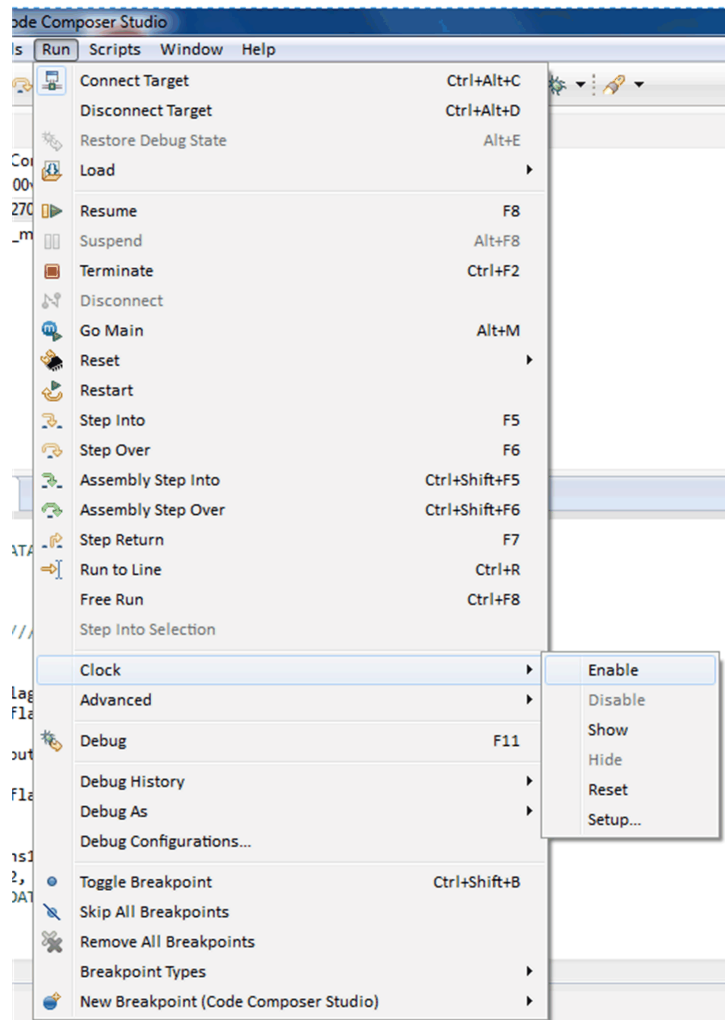
Figure 18. Clock Enable
