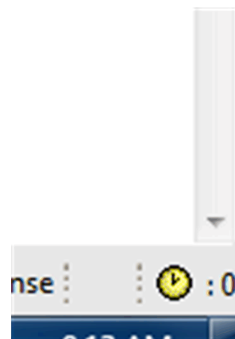
Figure 19. Clock Icon
