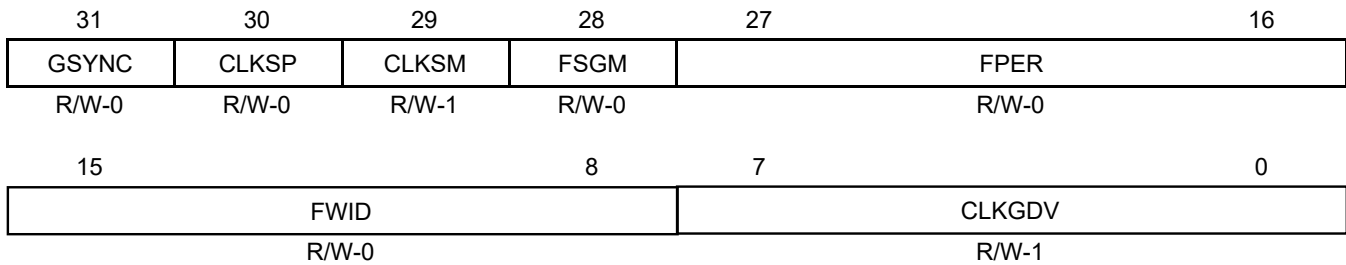
Figure 4. Sample Rate Generator Register (SRGR for SPI Master)
