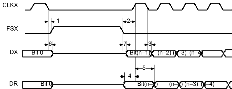
Figure 8. C6000 Timing, CLKSTP = 11b, CLKXP = 0
