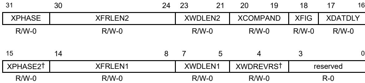
Figure 3. Transmit Control Register (XCR for SPI Master)
