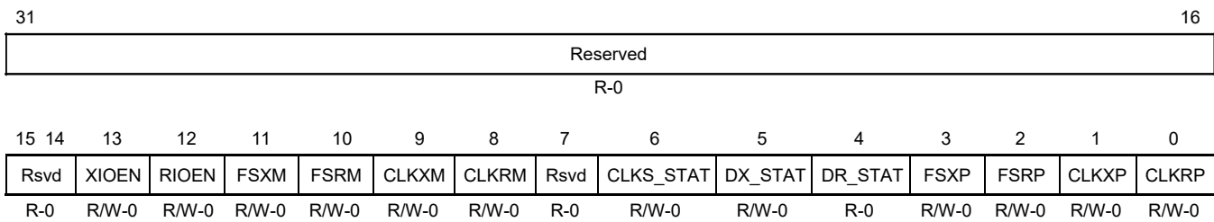
Figure 5. Pin Control Register (PCR for SPI Master)
