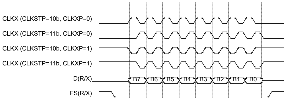
Figure 7. Clock Stop Mode Options
