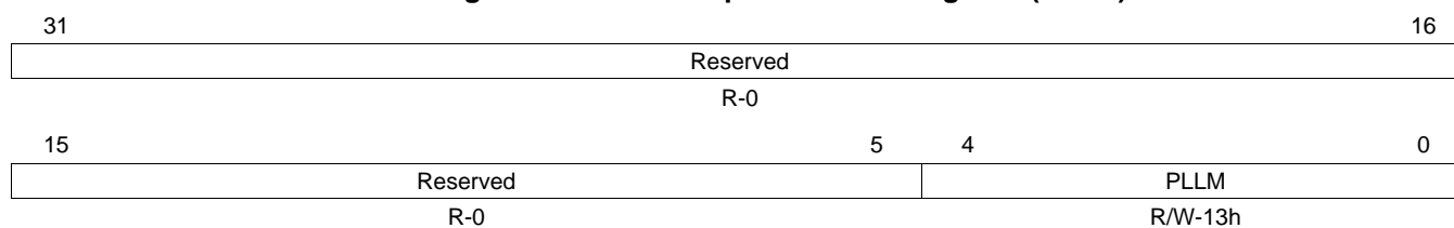
Figure 8-6. PLL Multiplier Control Register (PLLM)
