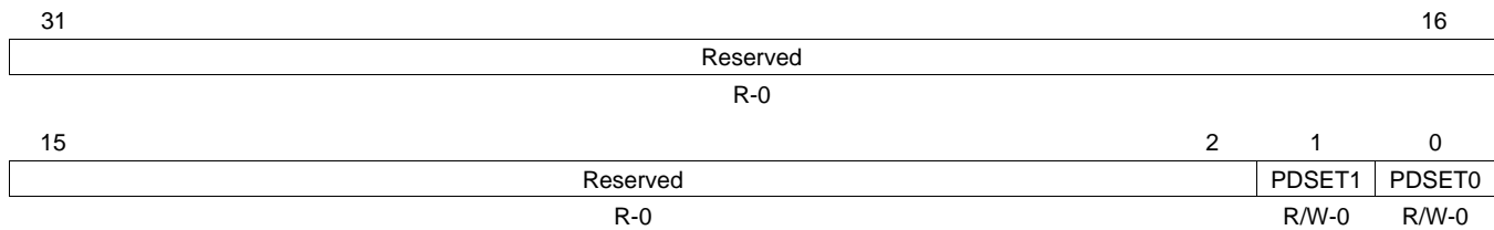
Figure 24-34. I2C Pin Data Set Register (ICPDSET)
