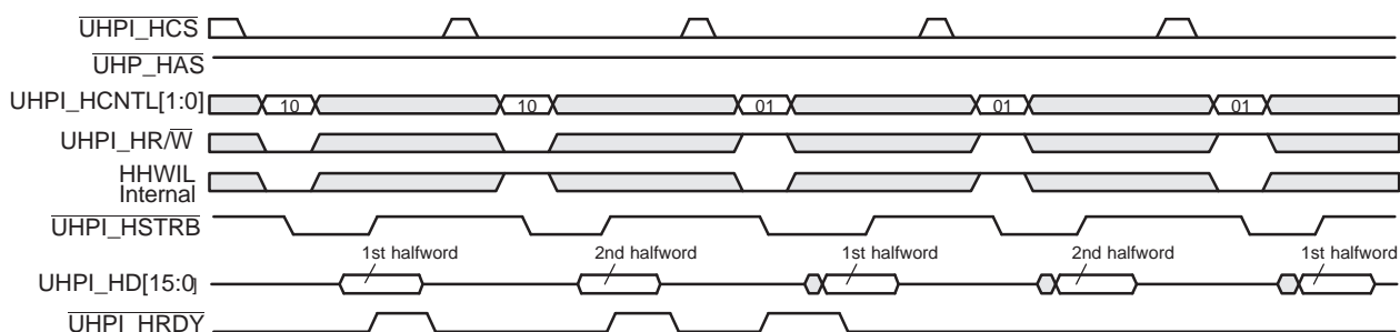
Figure 23-9. \overline{UHPI\_HRDY} Behavior During a Data Read Operation in the Multiplexed Mode (Case 2: HPIA Write Cycle Followed by Autoincrement HPID Read Cycles)
