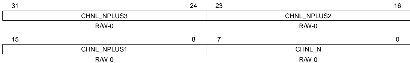
Figure 12-30. Channel Map Registers (CMRn)
