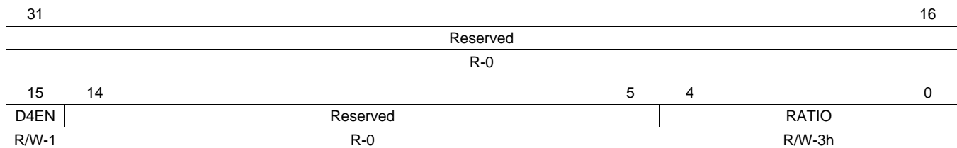
Figure 8-11. PLL Controller Divider 4 Register (PLLDIV4)
