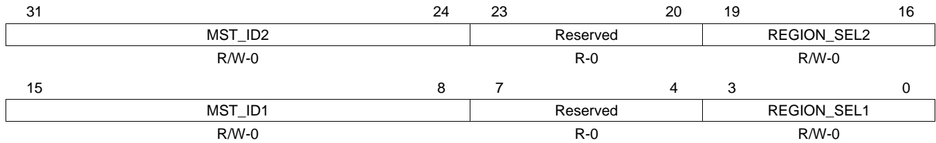
Figure 21-23. Performance Counter Master Region Select Register (PCMRS)
