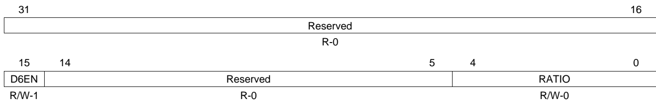
Figure 8-13. PLL Controller Divider 6 Register (PLLDIV6)
