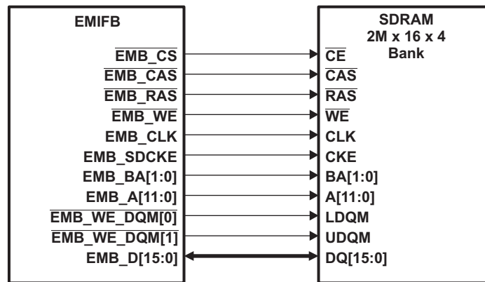
Figure 21-3. EMIFB to 2M × 16 × 4 bank SDRAM Interface
