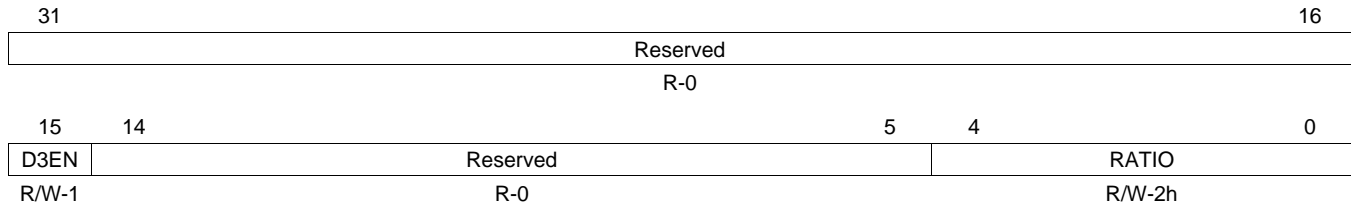
Figure 8-10. PLL Controller Divider 3 Register (PLLDIV3)
