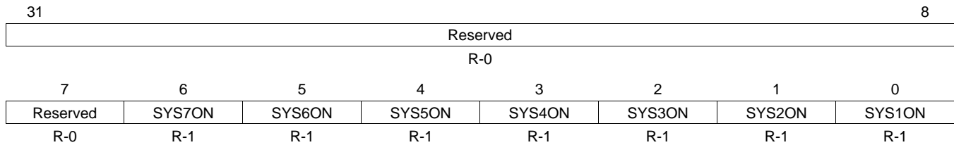
Figure 8-23. SYSCLK Status Register (SYSTAT)
