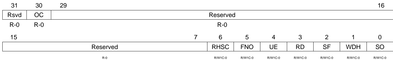
Figure 32-5. HC Interrupt and Status Register (HCINTERRUPTSTATUS)
