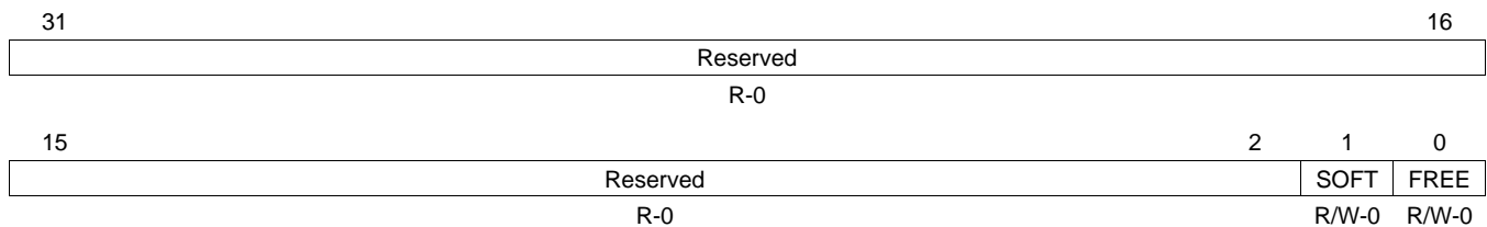
Figure 23-18. Power and Emulation Management Register (PWREMU_MGMT)
