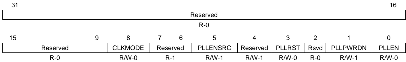
Figure 8-4. PLL Control Register (PLLCTL)
