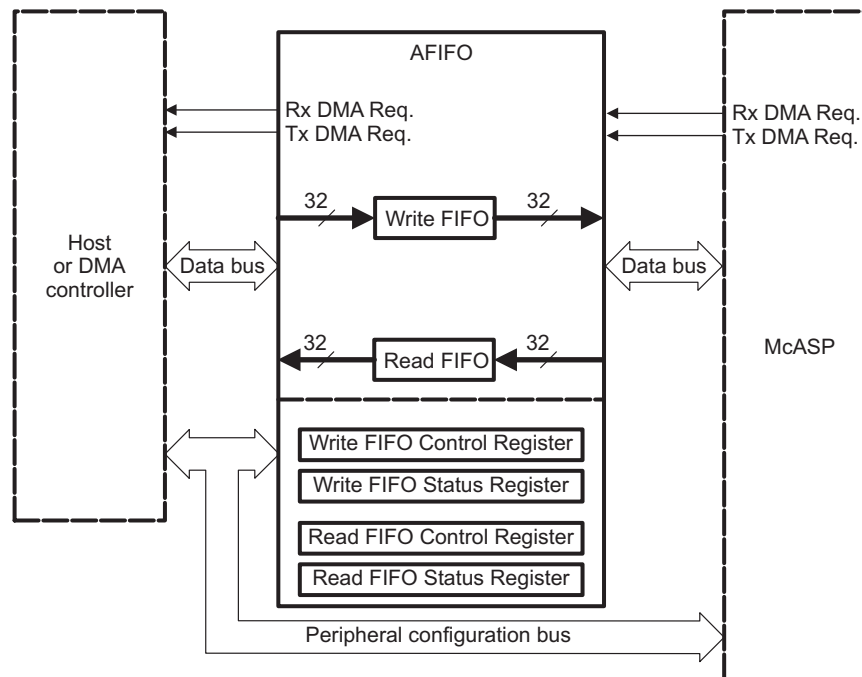
Figure 26-28. McASP Audio FIFO (AFIFO) Block Diagram
