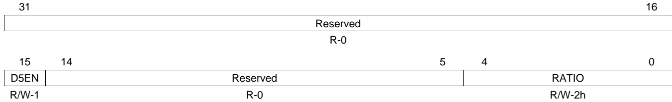
Figure 8-12. PLL Controller Divider 5 Register (PLLDIV5)
