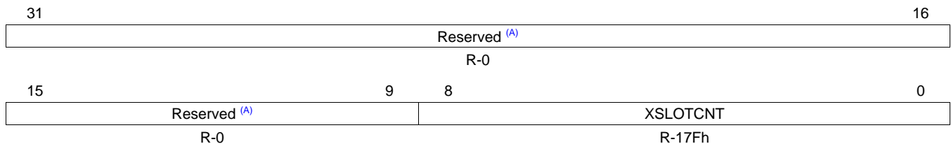
Figure 26-67. Current Transmit TDM Time Slot Register (XSLOT)
