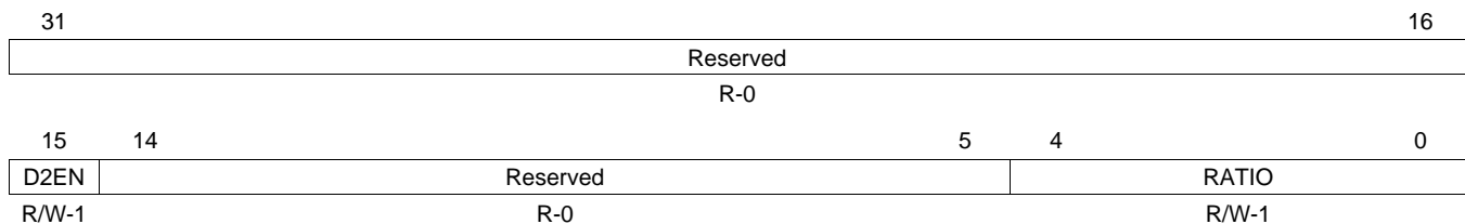
Figure 8-9. PLL Controller Divider 2 Register (PLLDIV2)
