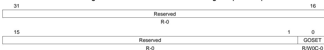
Figure 8-17. PLL Controller Command Register (PLLCMD)
