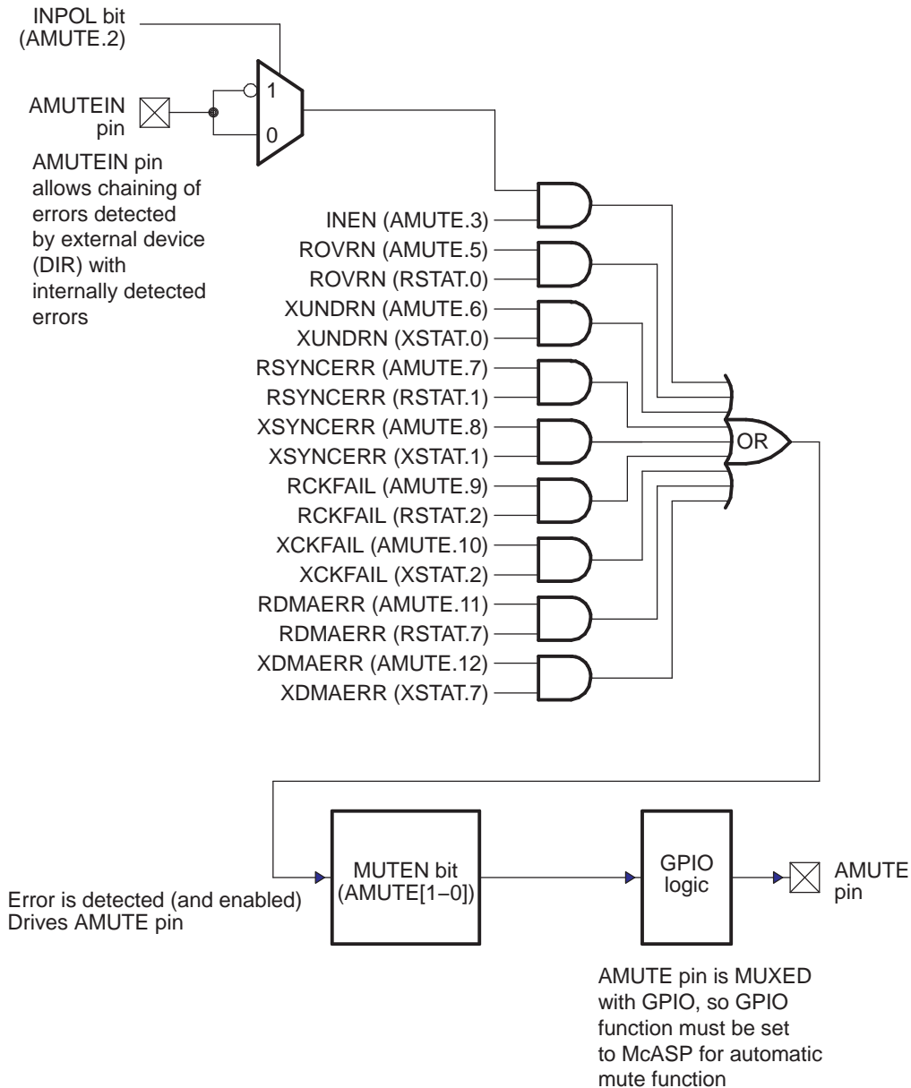
Figure 26-31. Audio Mute (AMUTE) Block Diagram
