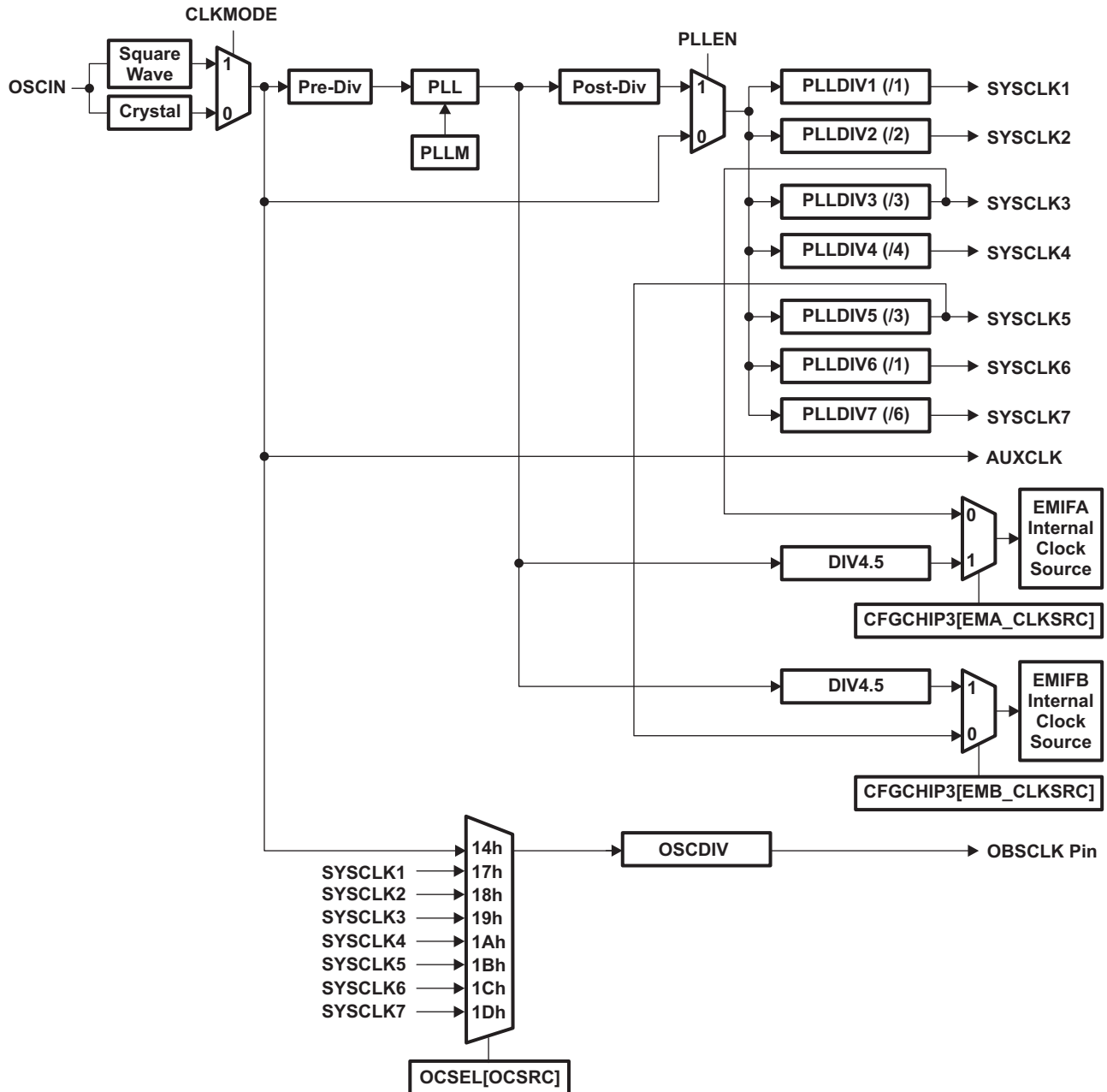
Figure 8-1. PLL0 Structure
