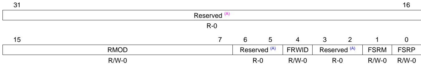
Figure 26-49. Receive Frame Sync Control Register (AFSRCTL)
