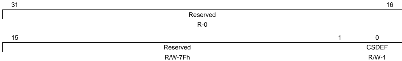
Figure 29-38. SPI Default Chip Select Register (SPIDEF)
