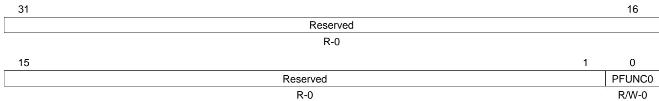
Figure 24-30. I2C Pin Function Register (ICPFUNC)
