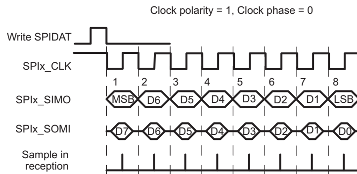
Figure 29-10. Clock Mode with POLARITY = 1 and PHASE = 0
