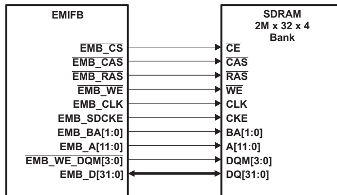
Figure 21-4. EMIFB to 2M × 32 × 4 bank SDRAM Interface
