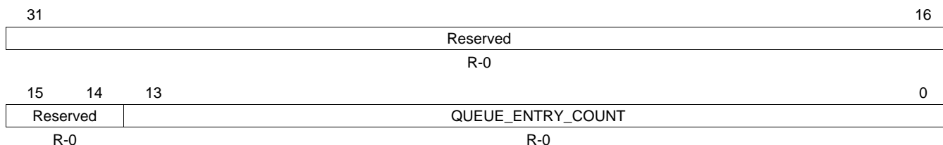
Figure 33-115. Queue Manager Queue N Status Register A (QSTATA[ M ])
