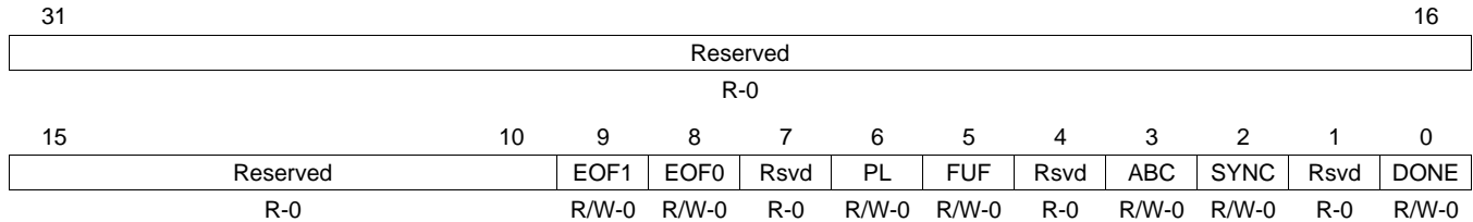
Figure 25-17. LCD Status Register (LCD_STAT)
