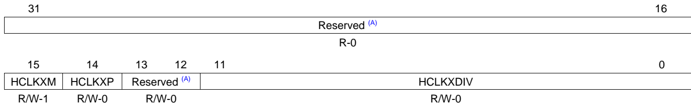
Figure 26-63. Transmit High-Frequency Clock Control Register (AHCLKXCTL)
