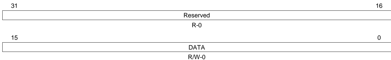
Figure 25-21. LCD LIDD CS n Data Read/Write Register (LIDD_CS n _DATA)
