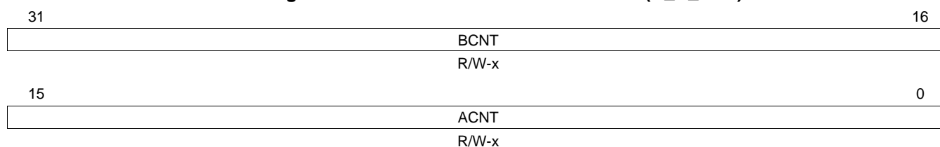
Figure 18-37. A Count/B Count Parameter (A_B_CNT)
