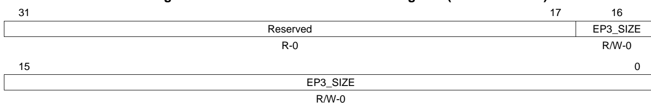
Figure 33-45. Generic RNDIS EP3 Size Register (GENRNDISSZ3)
