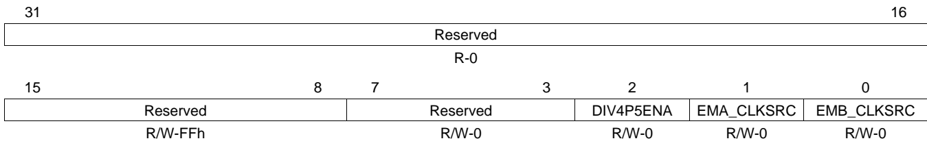
Figure 11-45. Chip Configuration 3 Register (CFGCHIP3)
