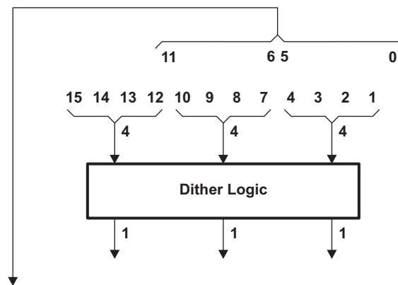
Figure 25-29. 16-BPP STN Mode
