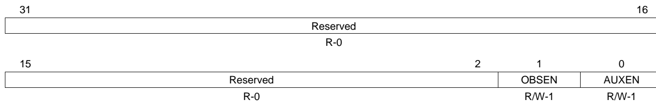
Figure 8-21. Clock Enable Control Register (CKEN)
