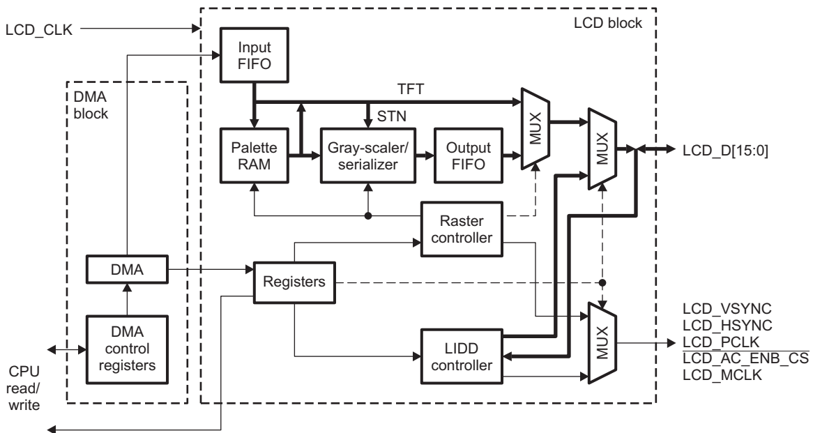
Figure 25-1. LCD Controller
