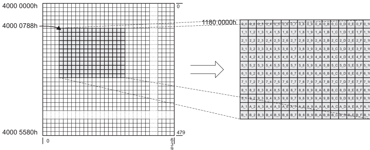
Figure 18-18. Subframe Extraction Example PaPARAM Configuration
