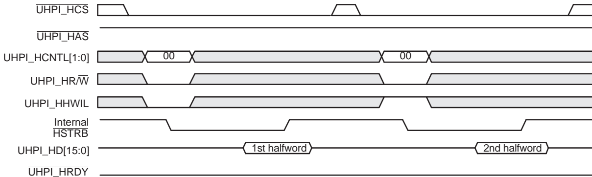
Figure 23-10. UHPI_HRDY Behavior During an HPIC Write Cycle in the Multiplexed Mode
