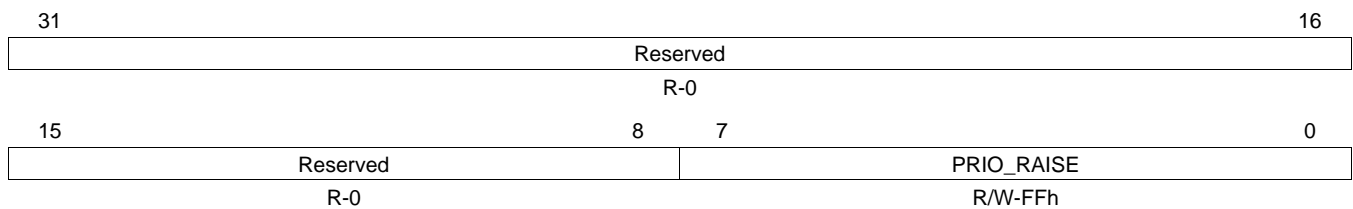
Figure 21-19. Peripheral Bus Burst Priority Register (BPRIO)
