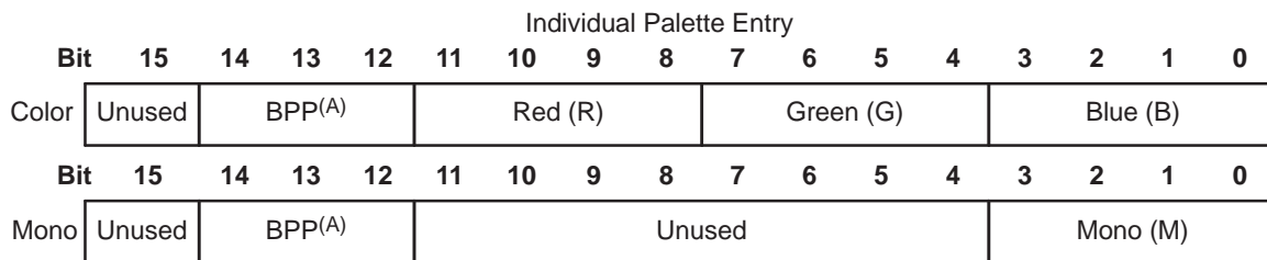
Figure 25-6. 256-Entry Palette/Buffer Format (8 BPP)
