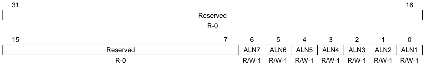
Figure 8-19. PLL Controller Clock Align Control Register (ALNCTL)
