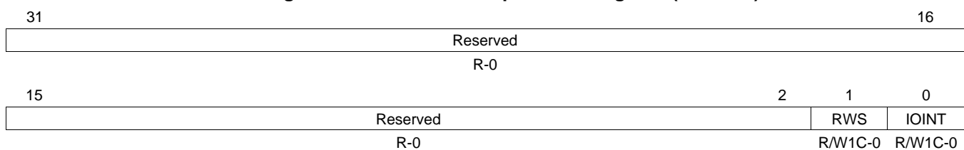
Figure 27-41. SDIO Interrupt Status Register (SDIOIST)
