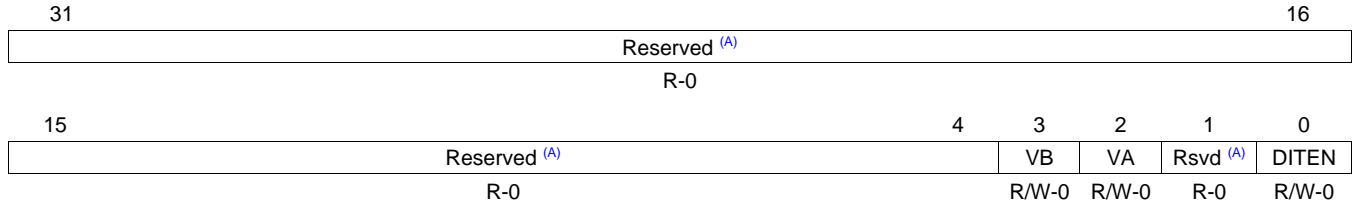
Figure 26-45. Digital Mode Control Register (DITCTL)
