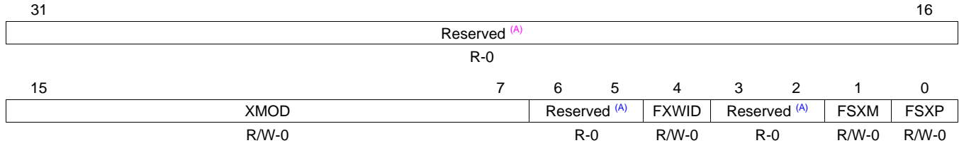
Figure 26-61. Transmit Frame Sync Control Register (AFSXCTL)
