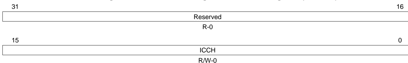
Figure 24-17. I2C Clock High-Time Divider Register (ICCLKH)
