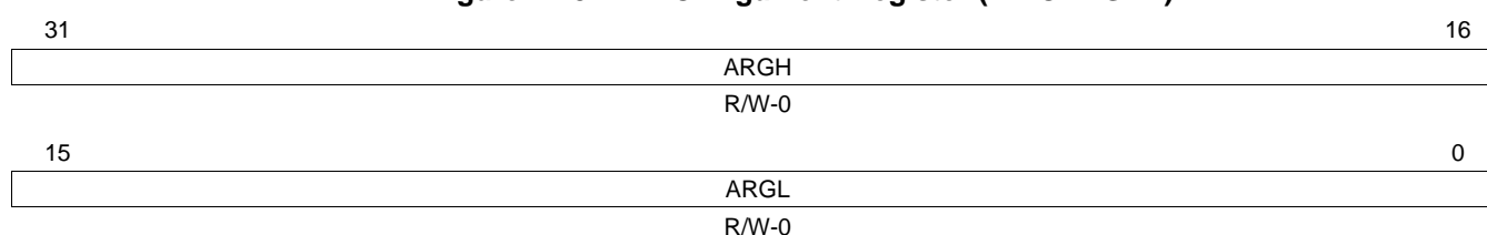
Figure 27-31. MMC Argument Register (MMCARGHL)
