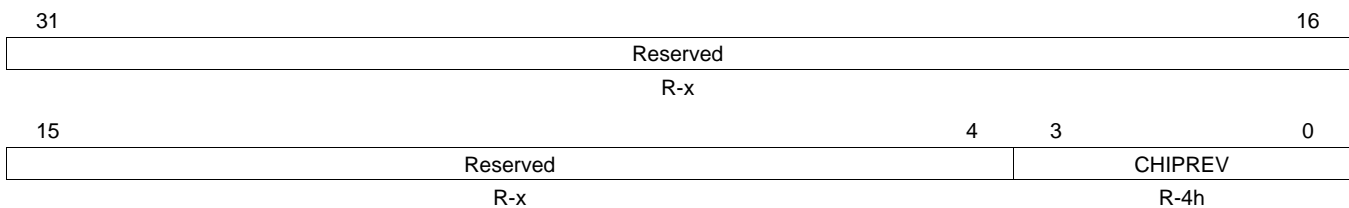
Figure 11-4. Silicon Revision Identification Register (CHIPREVID)
