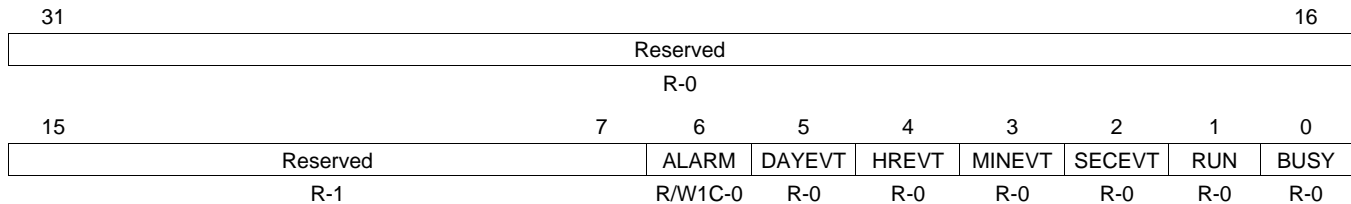
Figure 28-18. Status Register (STATUS)
