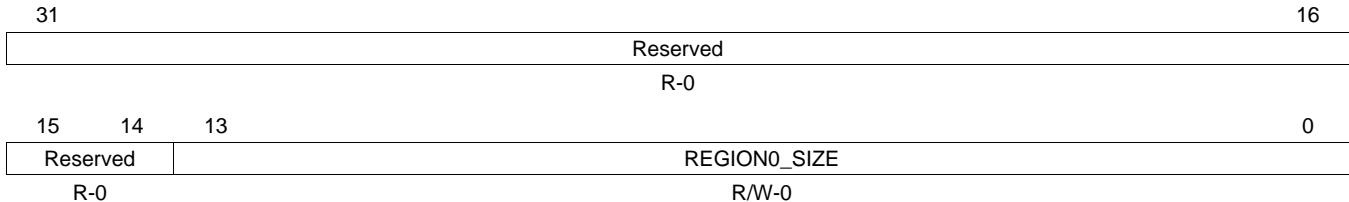
Figure 33-108. Queue Manager Linking RAM Region 0 Size Register (LRAM0SIZE)
