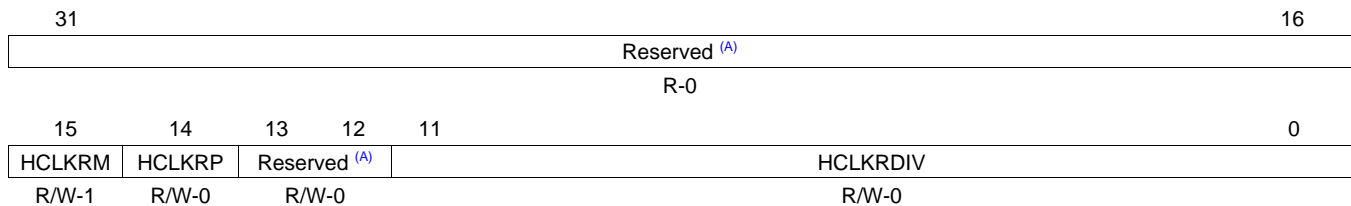
Figure 26-51. Receive High-Frequency Clock Control Register (AHCLKRCTL)
