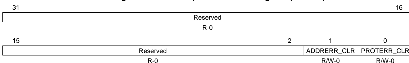
Figure 11-12. Interrupt Enable Clear Register (IENCLR)
