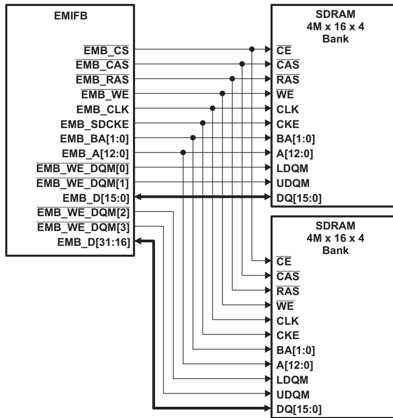
Figure 21-5. EMIFB to Dual 4M x 16 x 4 bank SDRAM Interface
