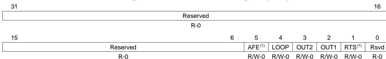
Figure 31-15. Modem Control Register (MCR)
