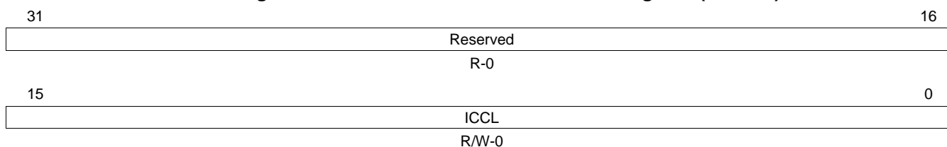
Figure 24-16. I2C Clock Low-Time Divider Register (ICCLKL)
