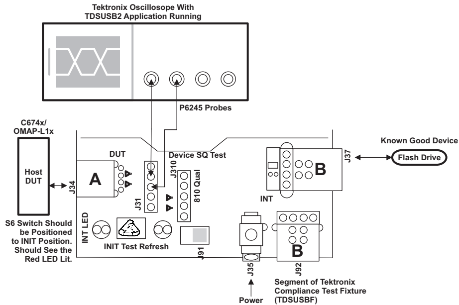
Figure 14. Equipment Setup for Downstream Host Chirp and Suspend and Resume Timings
