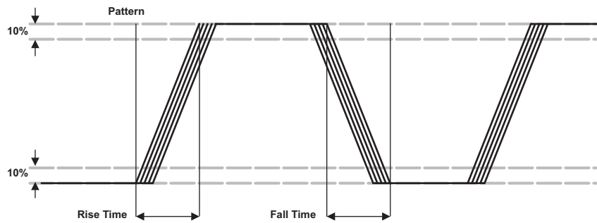
Figure 5. Rise and Fall Time Patterns
