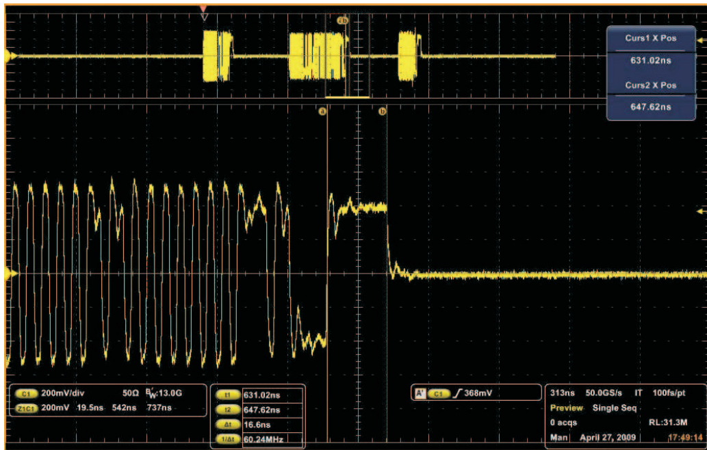
Figure 12. EOP Field of Non-SOP Packet of the Data Packet of the Status Stage of the GET DESCRIPTOR Command
