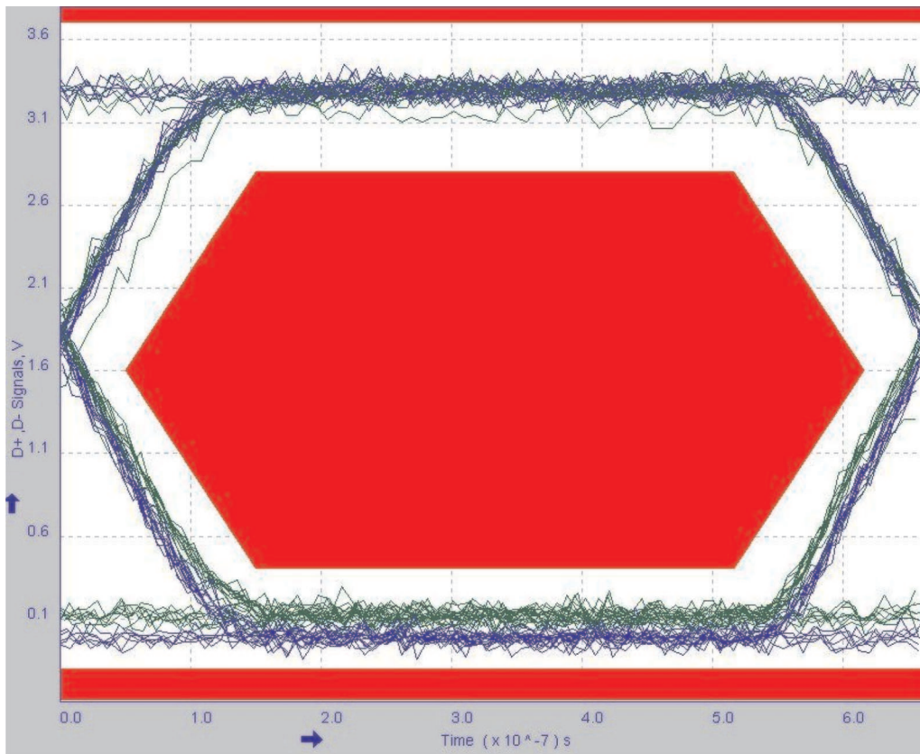
Figure 26. Low-Speed Eye Diagram
