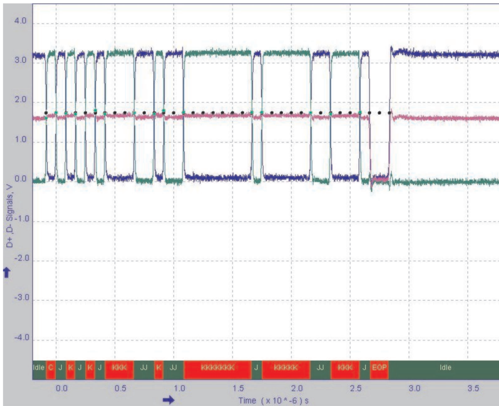
Figure 22. Waveform Plot
