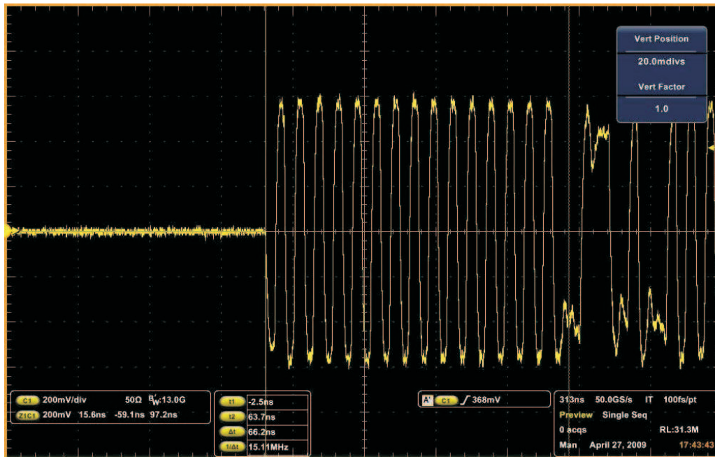
Figure 9. Status Stage of a GET DEVICE DESCRIPTOR Transaction SYNC Field of the Token Packet
