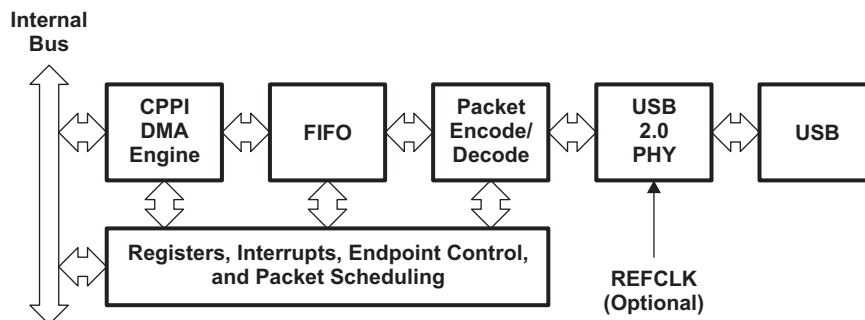
Figure 1. USB Functional Block Diagram
