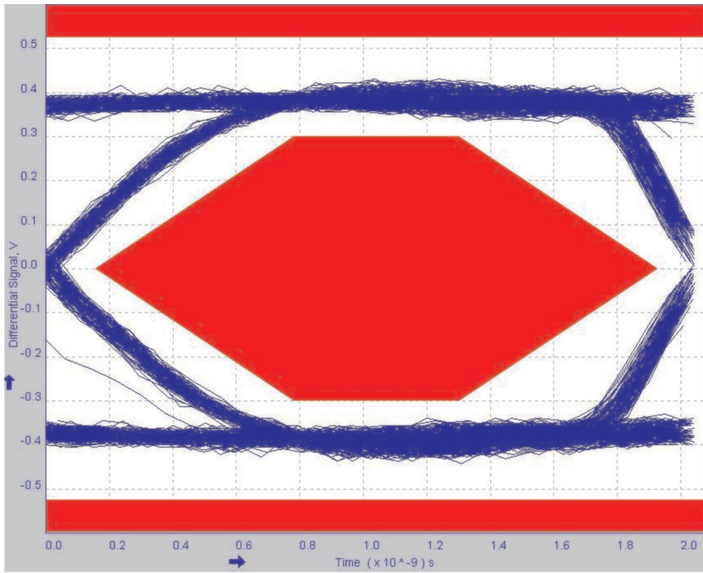
Figure 3. Downstream Eye Diagram
