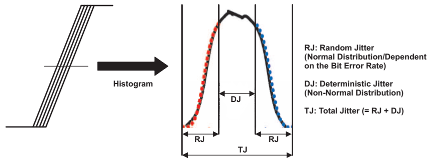
Figure 7. Random Jitter/Deterministic Jitter/Total Jitter
