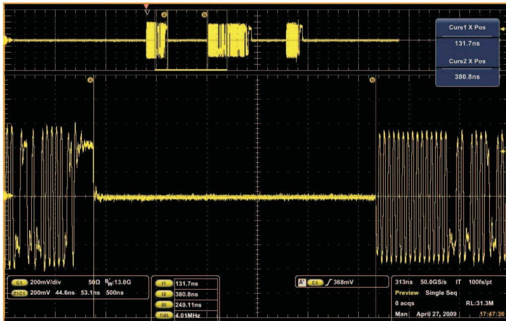
Figure 11. Inter-Packet-Gap Between the Token Packet and the Data Packet of the Status Stage of the GET DESCRIPTOR Transaction
