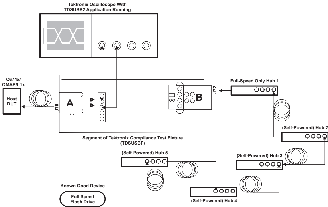
Figure 21. Equipment Setup for Full-Speed Downstream Host Signal Quality Testing
