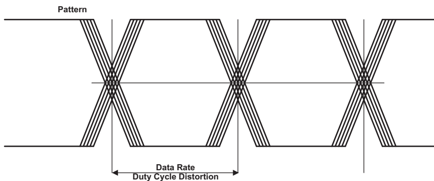
Figure 6. Duty Cycle Distortion (DCD)
