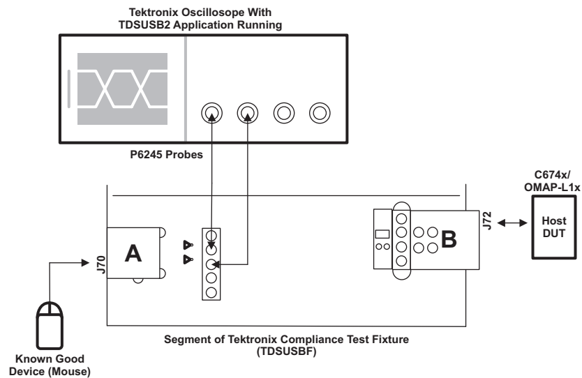
Figure 24. Equipment Setup for Low-Speed Downstream Host Signal Quality Testing
