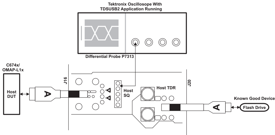
Figure 2. Equipment Setup for High-Speed Downstream Host Signal Quality Testing
