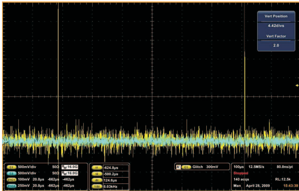
Figure 17. Time Between First SOF and Last Chirp-(J or K)
