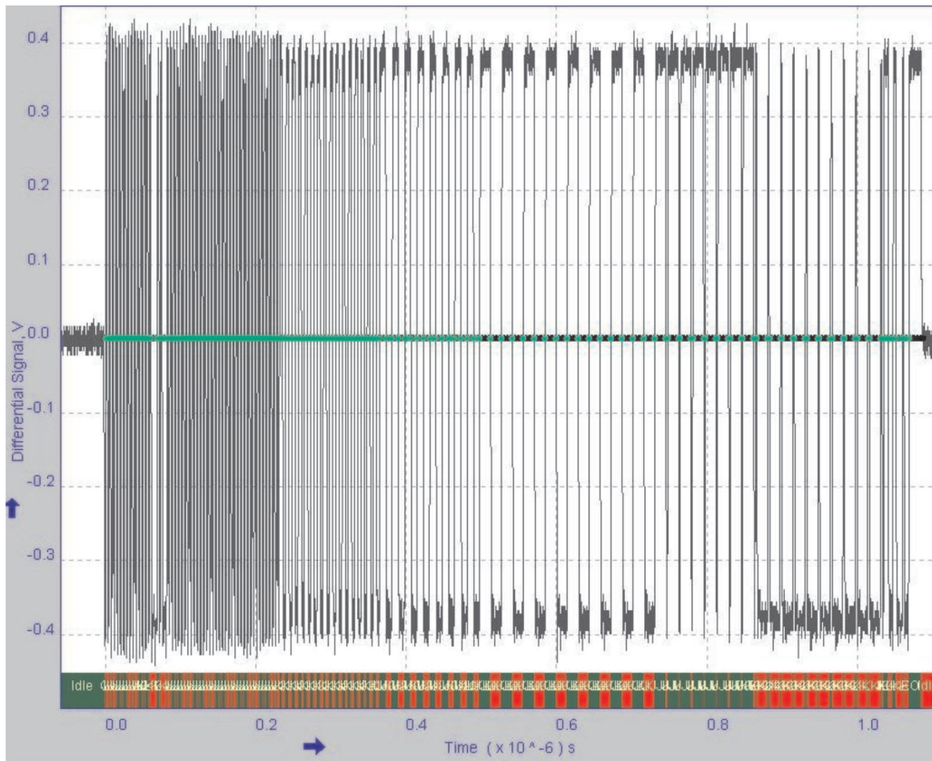
Figure 4. Downstream Waveform Plot
