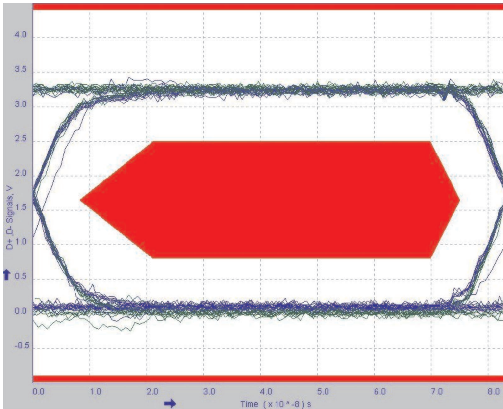
Figure 23. Full-Speed Eye Diagram
