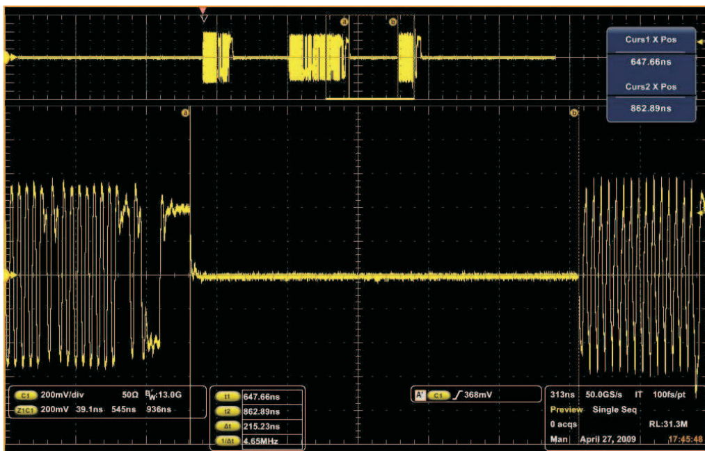
Figure 10. Inter-Packet-Gap Between the Data Packet of Device and Acknowledge Packet of the Embedded Host on the Data Stage of the GET DESCRIPTOR Command
