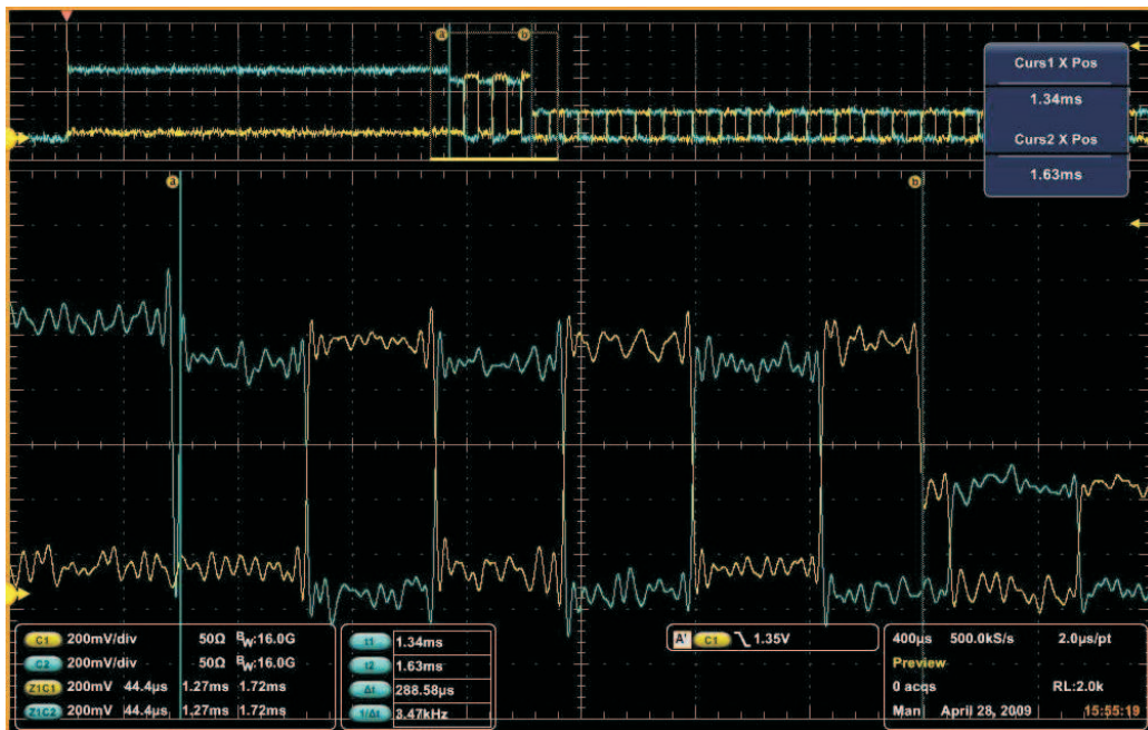
Figure 16. Chirp-K and Chirp-J Duration
