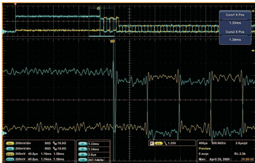
Figure 15. Downstream Chirp Response Time
