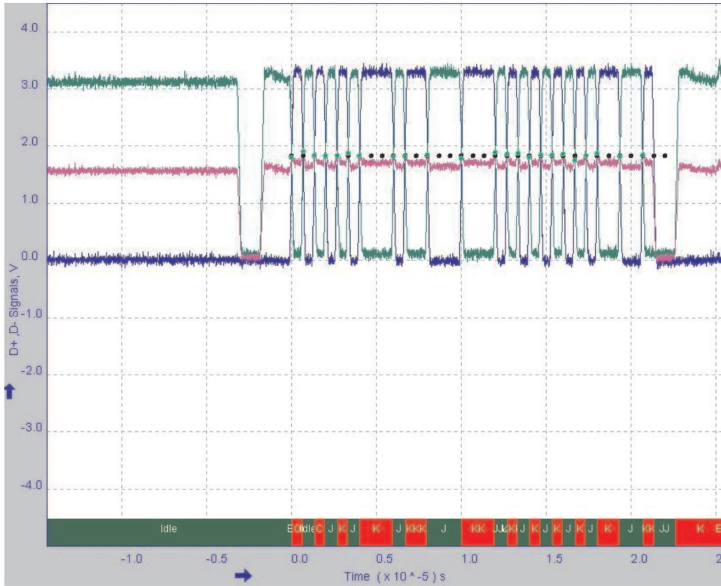
Figure 25. Low-Speed Waveform Plot
