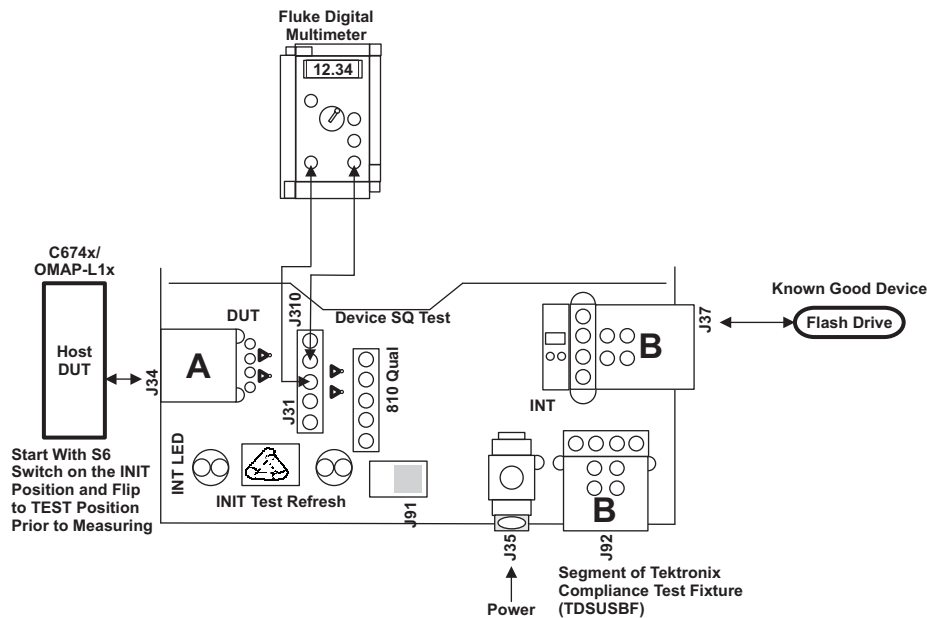
Figure 20. Equipment Setup for Downstream Test J/K, SEO_NAK
