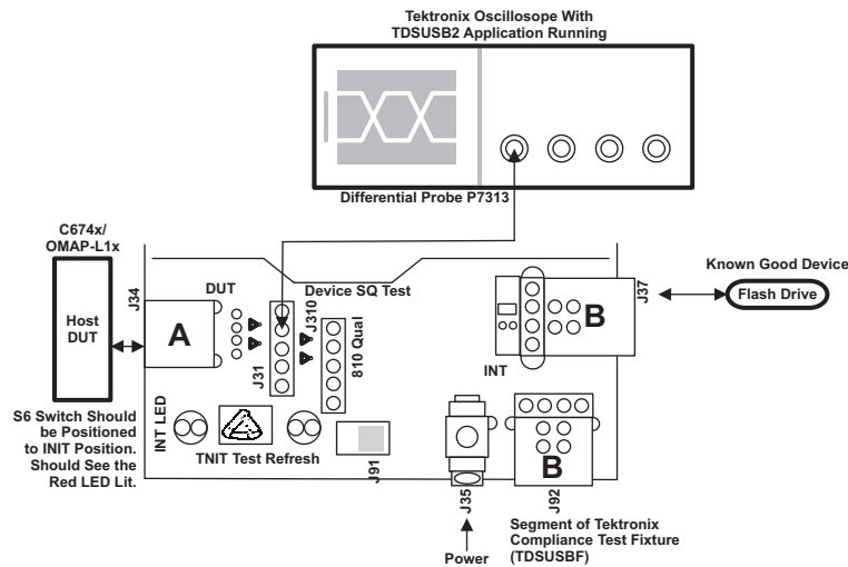
Figure 8. Equipment Setup for Downstream Host Packet Parameters Tests
