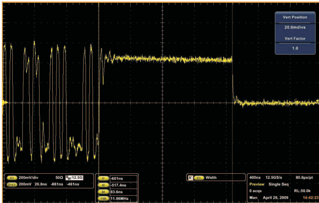
Figure 13. EOP Field of an SOP Packet
