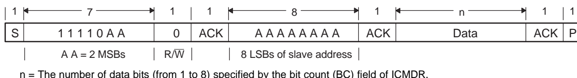
Figure 9. I2C Peripheral 10-Bit Addressing Format With Master-Transmitter Writing to Slave-Receiver (FDF = 0, XA = 1 in ICMDR)
