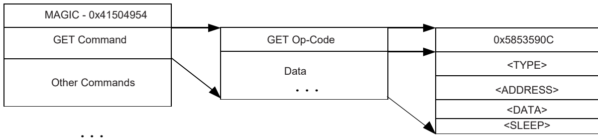
Figure 8. Structure of GET Command
