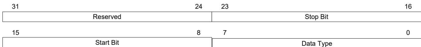
Figure 7. Valid SET Command Data Types
