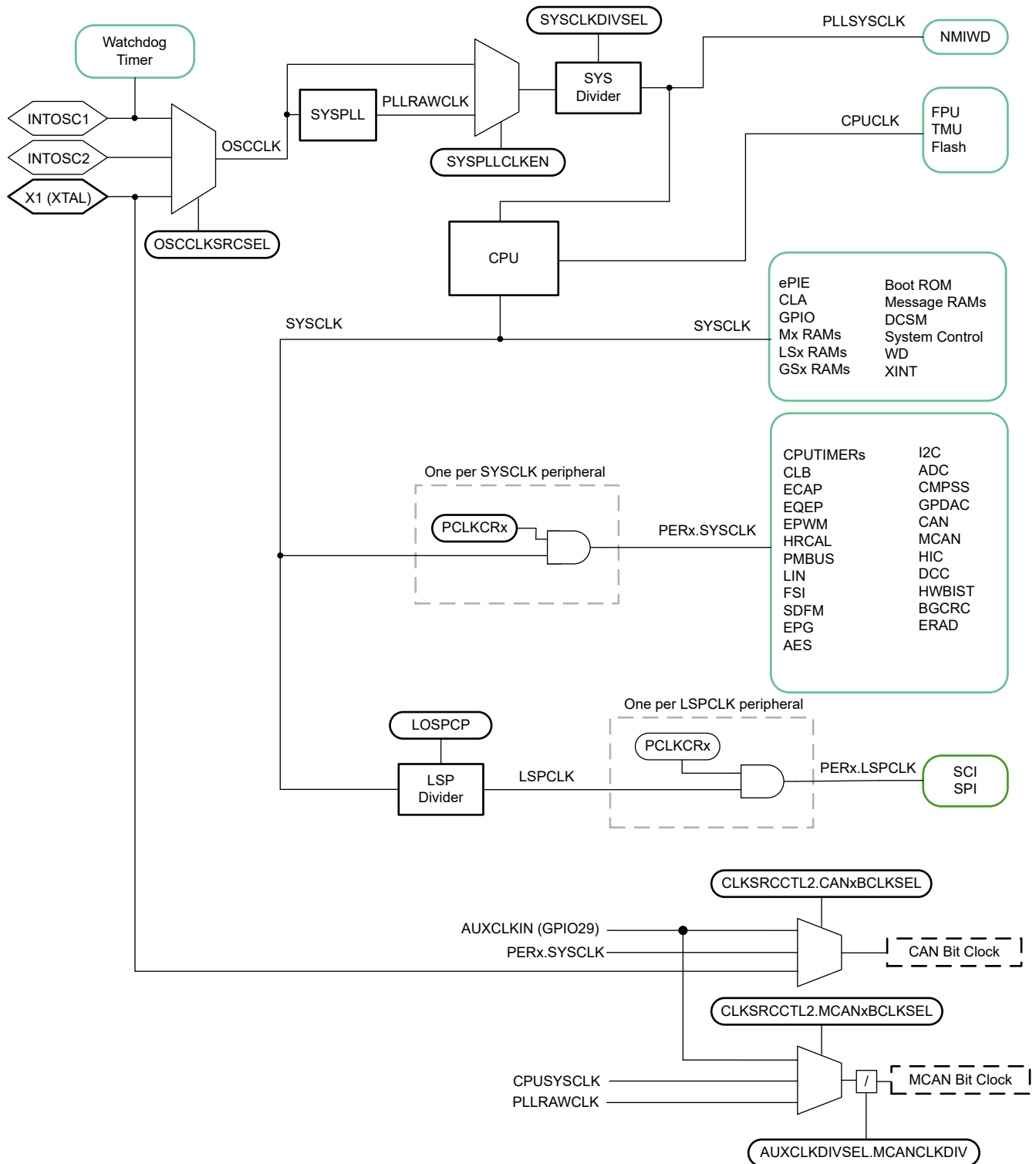
Figure 6-9. Clocking System
