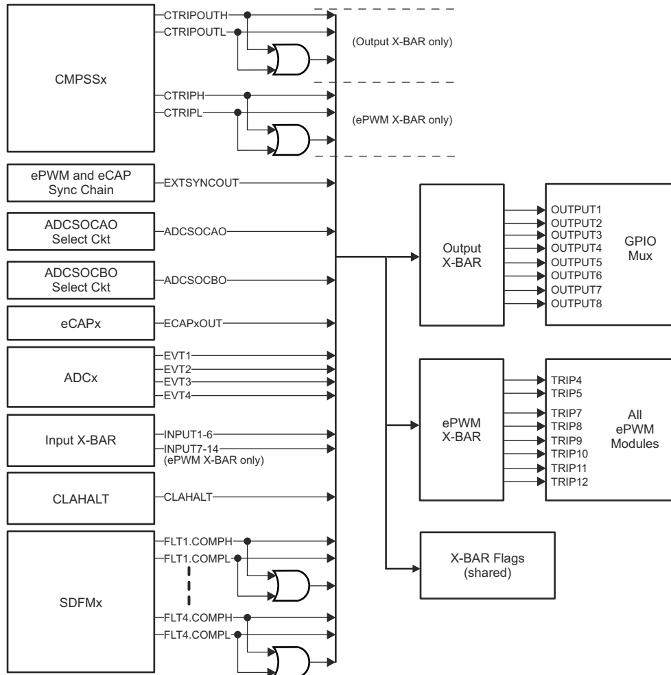
Figure 18-58. ePWM X-BAR
