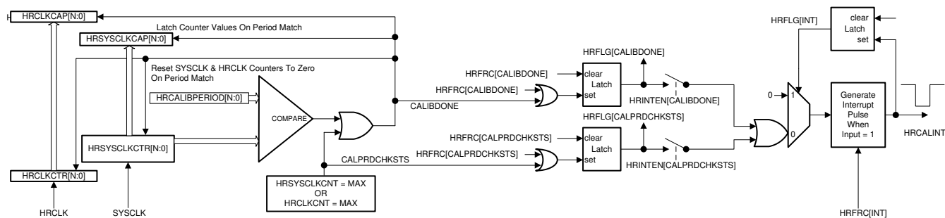
Figure 20-2. HRCAP Calibration
