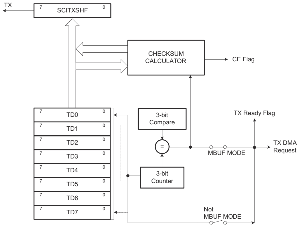
Figure 27-9. Transmit Buffers
