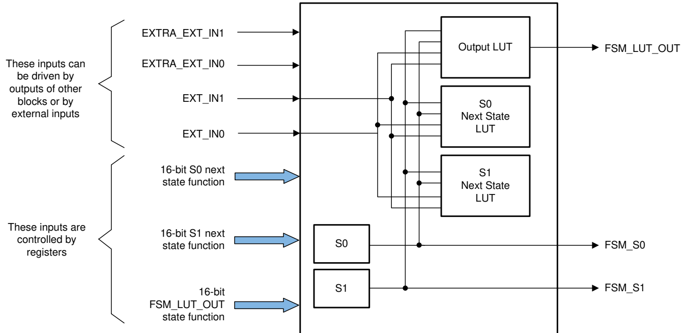
Figure 29-11. FSM Block
