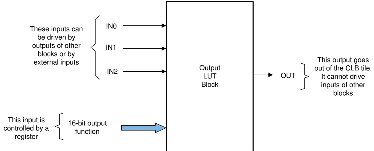
Figure 29-14. Output LUT Block
