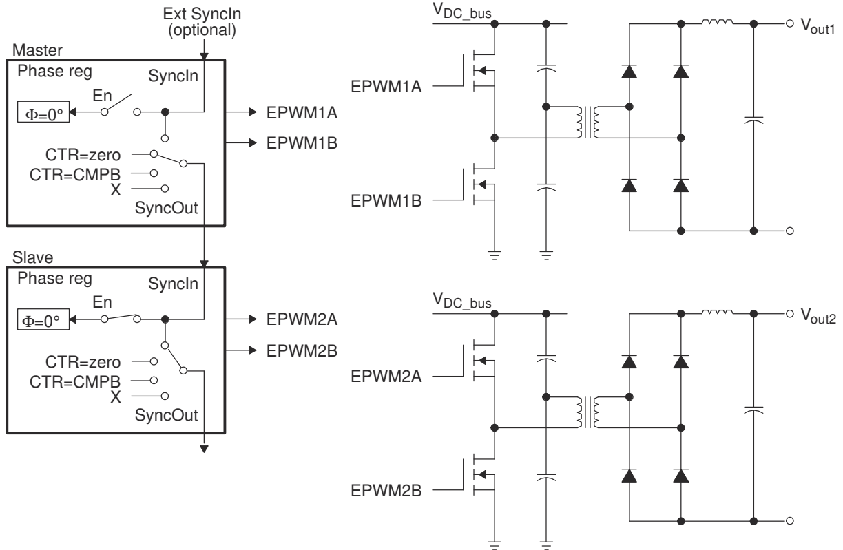
Figure 18-66. Control of Two Half-H Bridge Stages ( F_{PWM2} = N \times F_{PWM1} )
