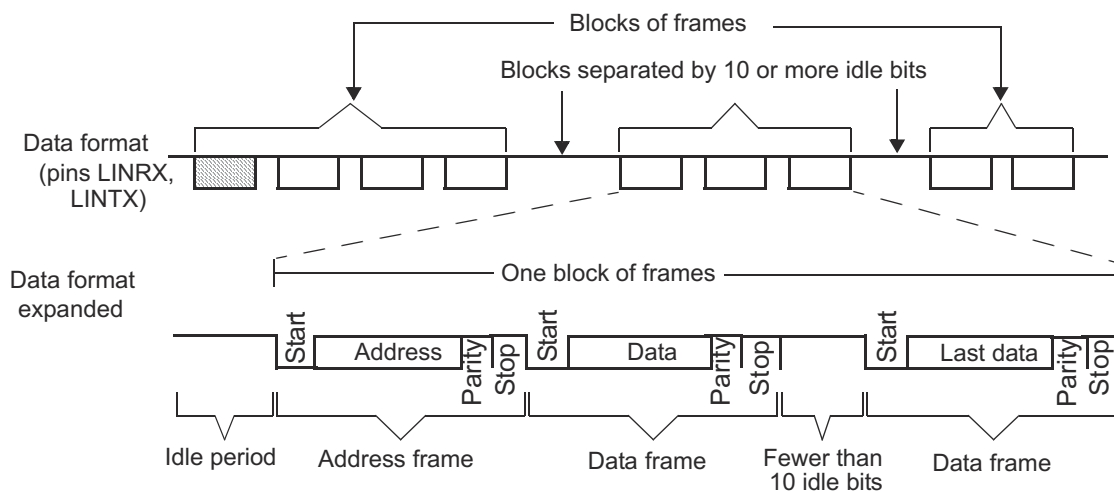
Figure 27-6. Idle-Line Multiprocessor Communication Format
