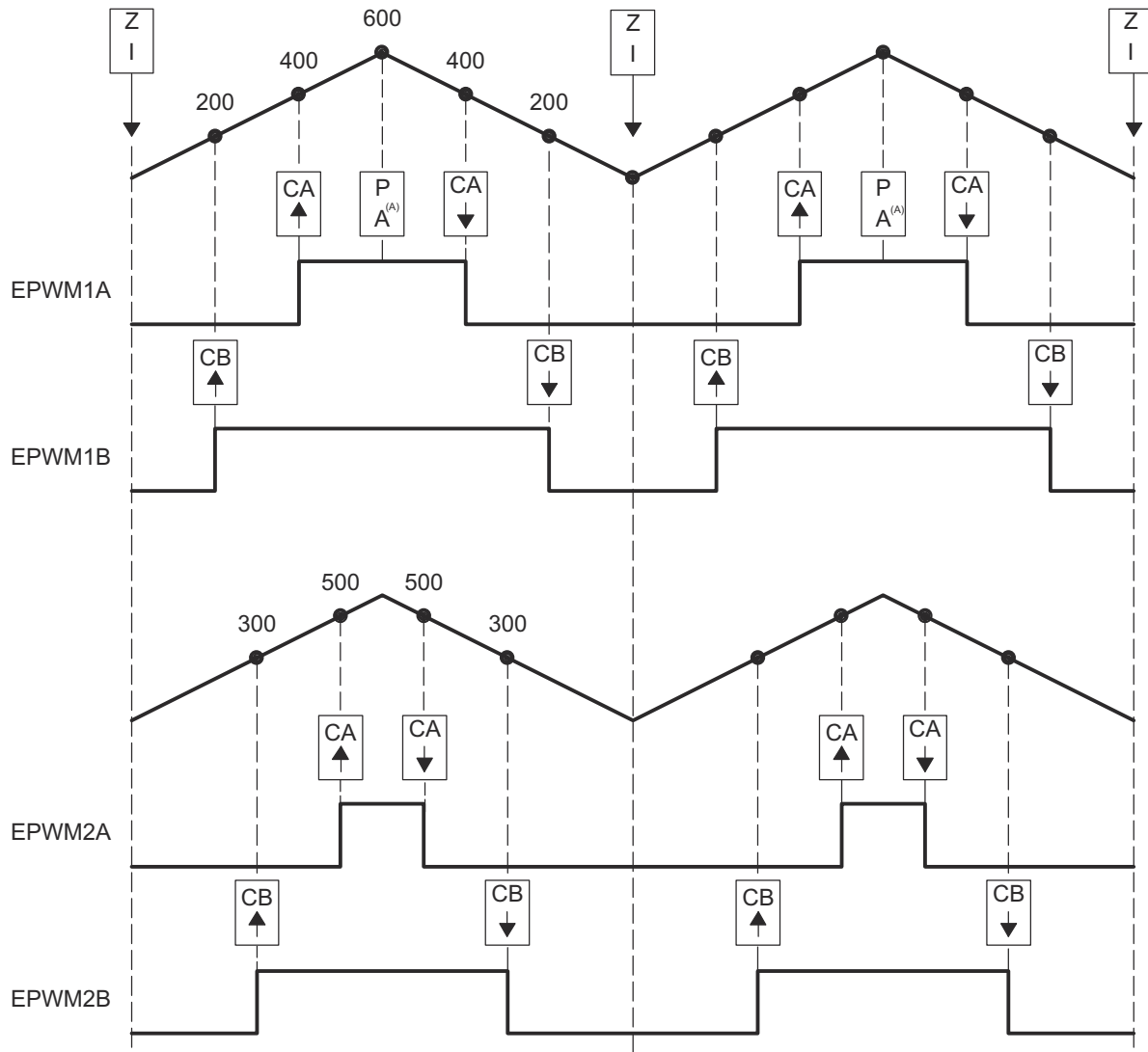
Figure 18-65. Buck Waveforms for Figure 18-64 (Note: F_{PWM2} = F_{PWM1} )
