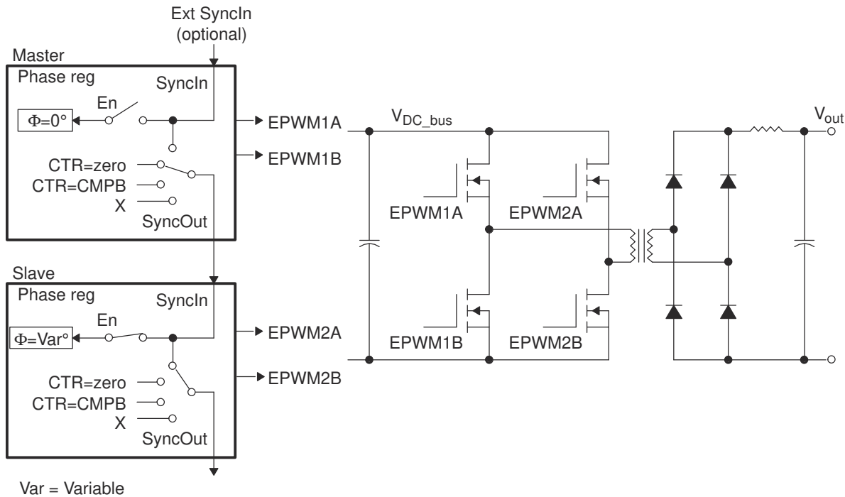
Figure 18-74. Controlling a Full-H Bridge Stage ( F_{PWM2} = F_{PWM1} )
