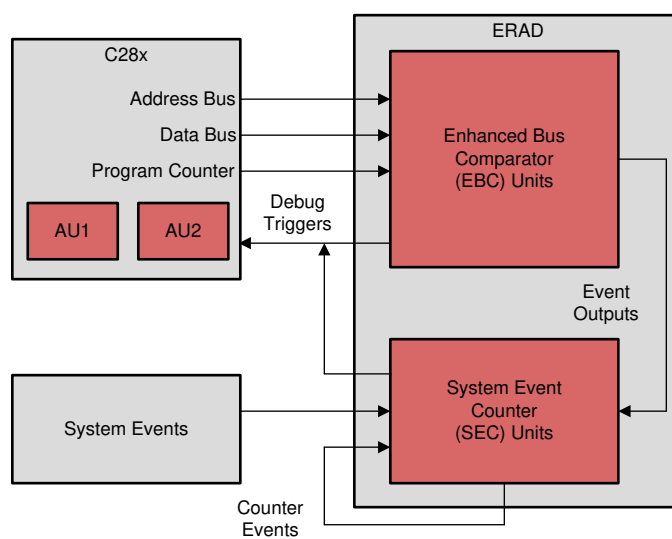
Figure 11-1. ERAD Overview
