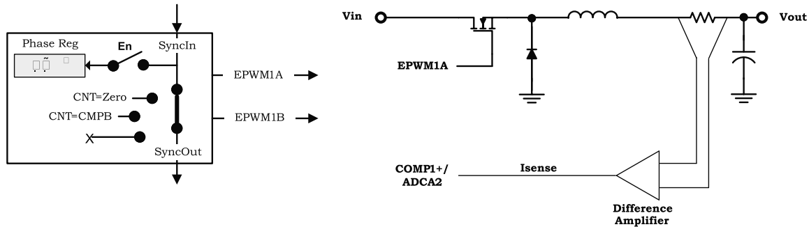
Figure 18-76. Peak Current Mode Control of a Buck Converter
