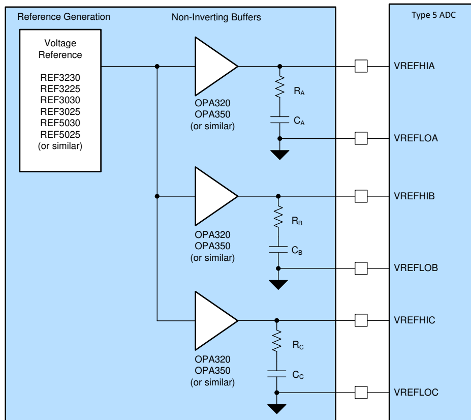
Figure 13-19. ADC Reference System
