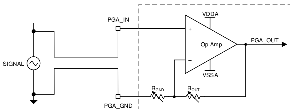
Figure 14-6. PGA Amplifier Example
