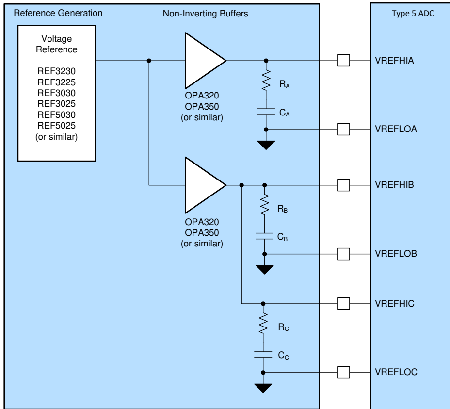
Figure 13-20. ADC Shared Reference System
