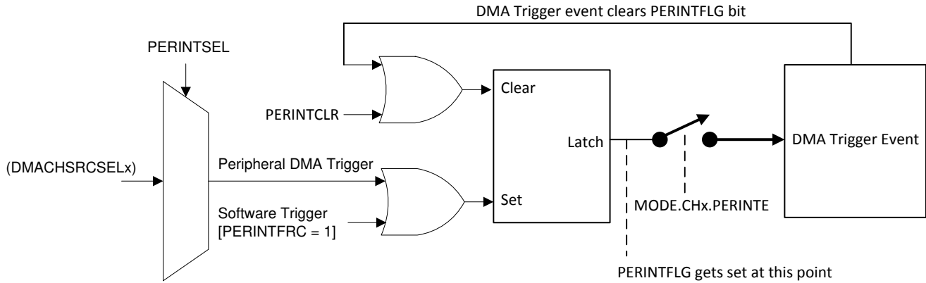
Figure 10-3. Peripheral Interrupt Trigger Input Diagram
