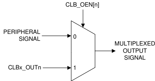
Figure 29-7. Peripheral Signal Multiplexer
