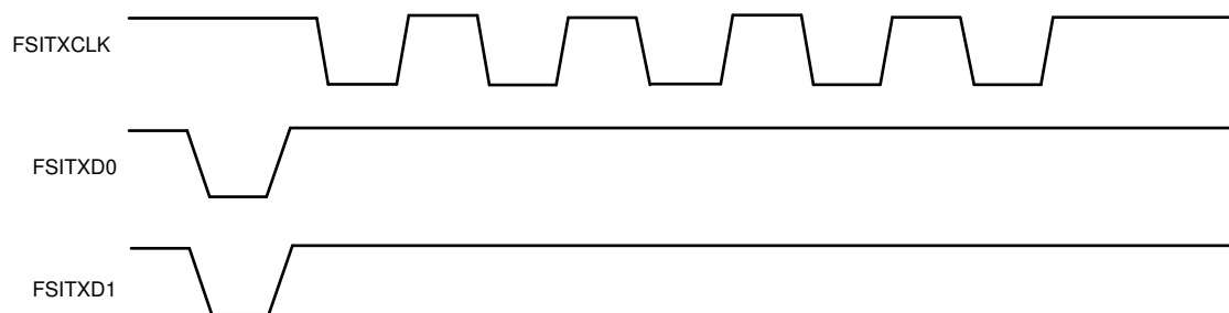
Figure 28-9. Flush Sequence Signals
