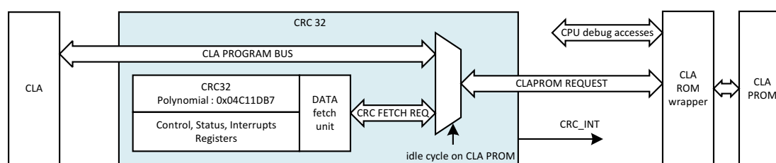
Figure 7-1. CLAPROMCRC Functional Diagram
