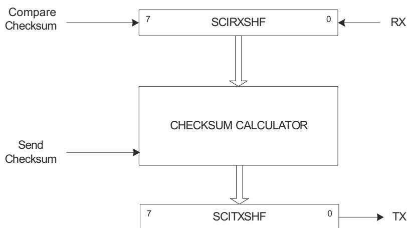
Figure 27-20. Checksum Compare and Send for Extended Frames
