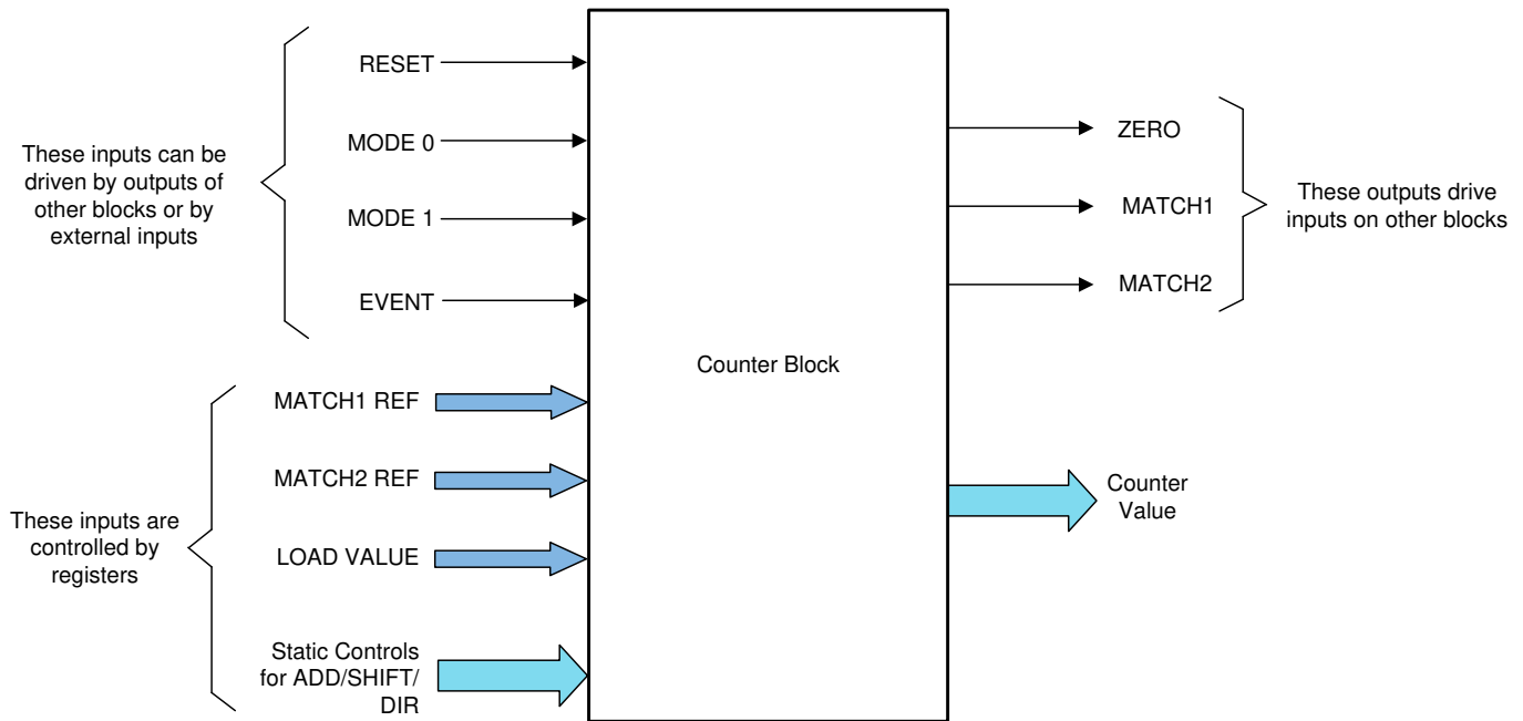
Figure 29-9. Counter Block
