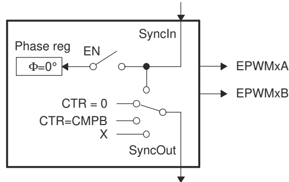
Figure 18-60. Simplified ePWM Module
