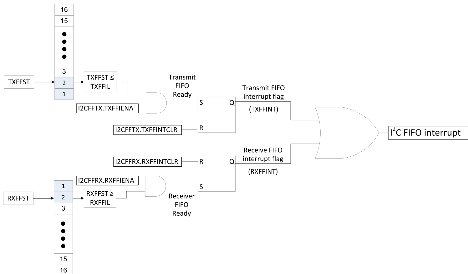
Figure 24-17. I2C_FIFO_interrupt
