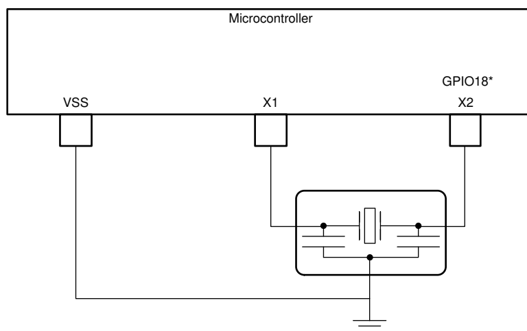
Figure 3-8. External Resonator
