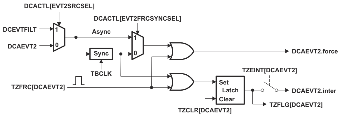
Figure 18-52. DCAEV2 Event Triggering
