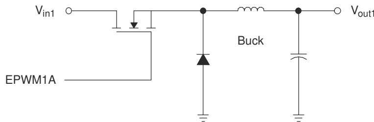
Figure 18-91. Simple Buck Controlled Converter Using a Single PWM
