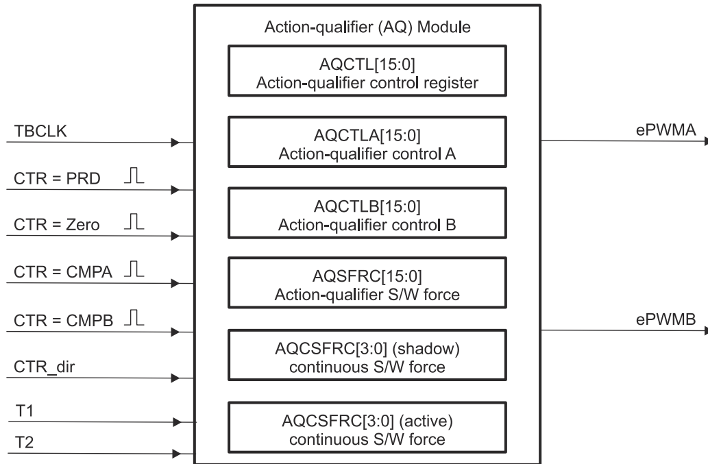
Figure 18-21. Action-Qualifier Submodule Inputs and Outputs
