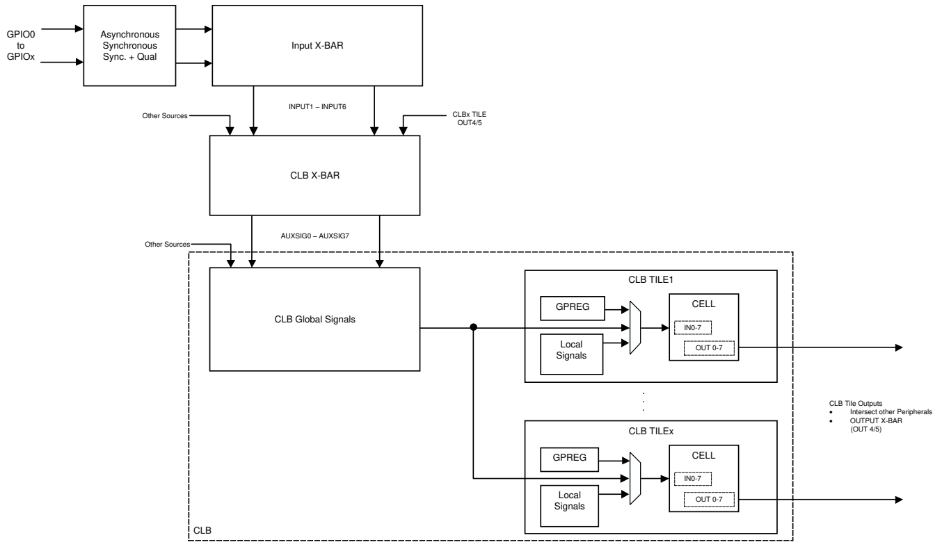
Figure 29-5. GPIO to CLB Tile Connections
