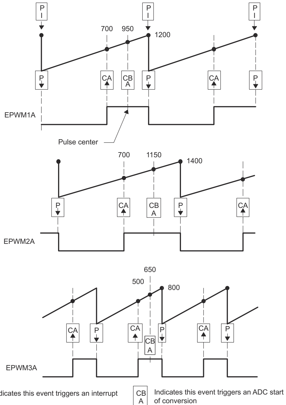
Figure 18-63. Buck Waveforms for Figure 18-62 (Note: Only three bucks shown here)
