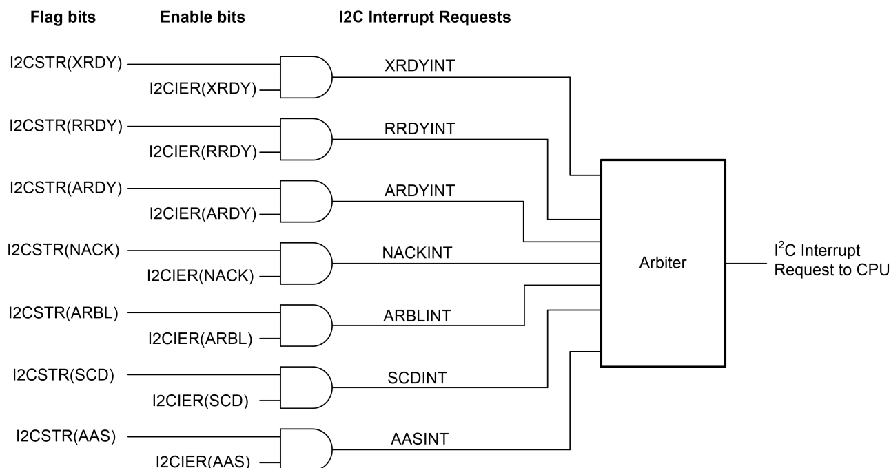
Figure 24-15. Enable Paths of the I2C Interrupt Requests
