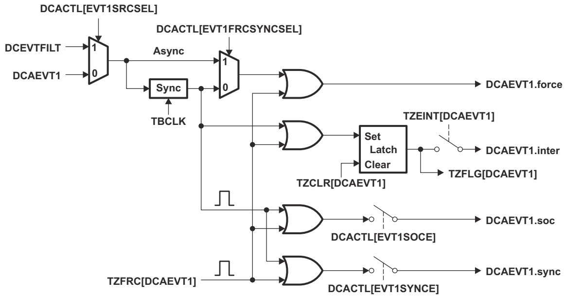
Figure 18-51. DCAEV1 Event Triggering
