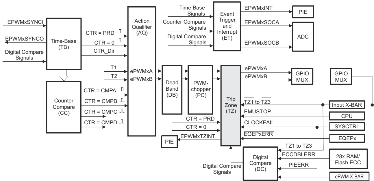
Figure 18-41. Trip-Zone Submodule
