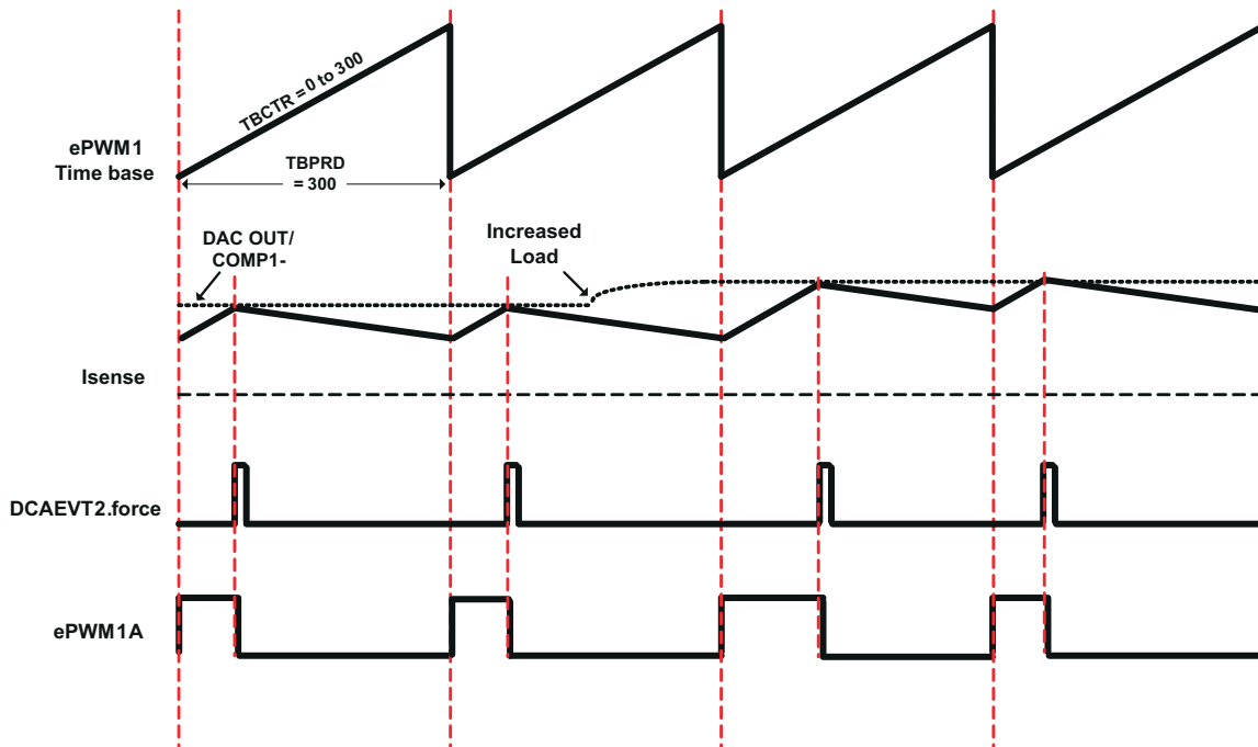
Figure 18-77. Peak Current Mode Control Waveforms for Figure 18-76
