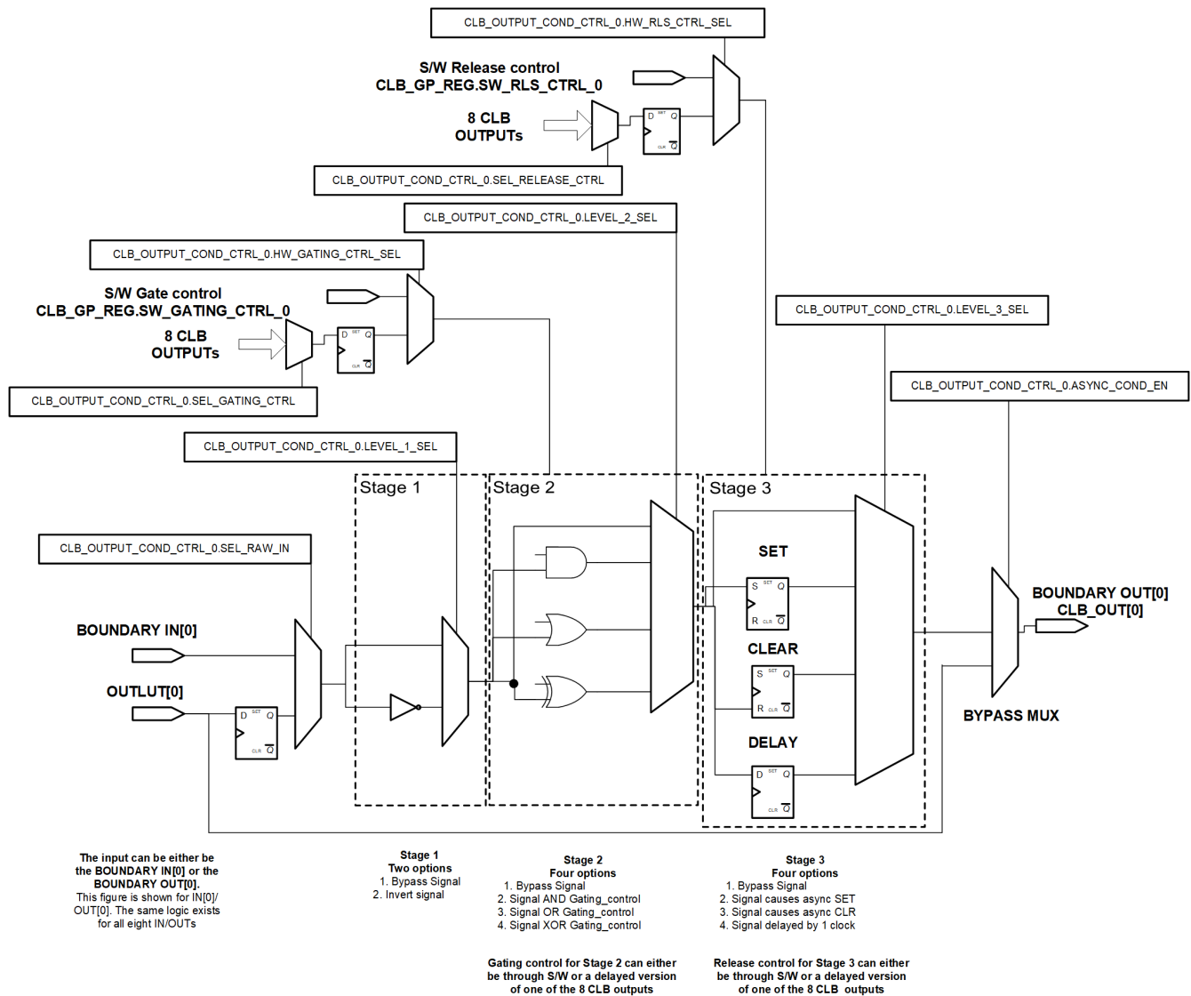
Figure 29-15. AOC Block
