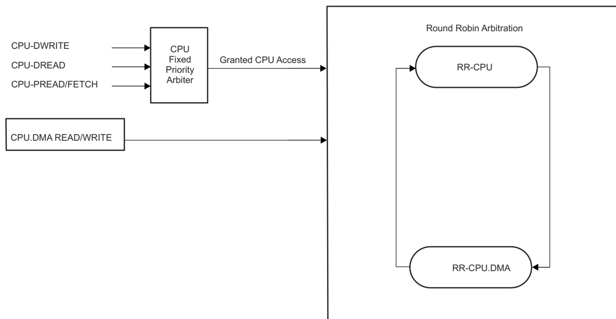
Figure 3-13. Arbitration Scheme on Global Shared Memories
