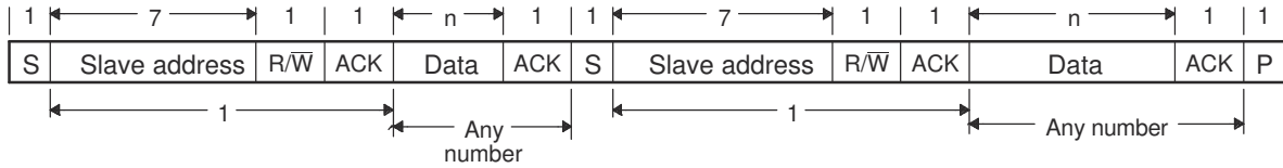
Figure 24-11. Repeated START Condition (in This Case, 7-Bit Addressing Format)
