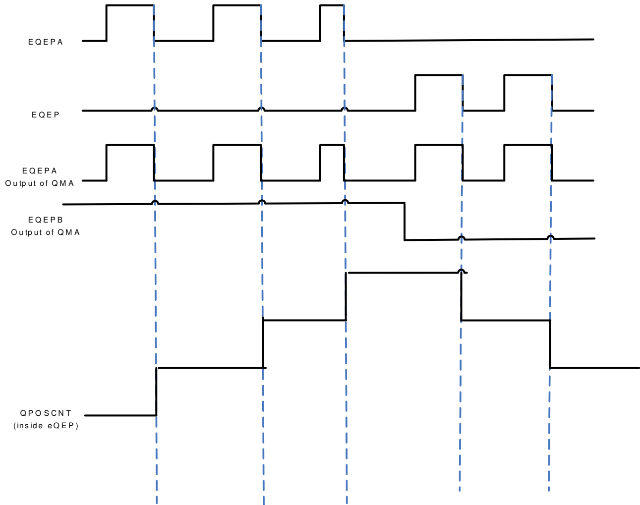
Figure 21-22. QMA Mode-2
