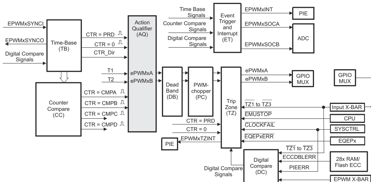
Figure 18-20. Action-Qualifier Submodule
