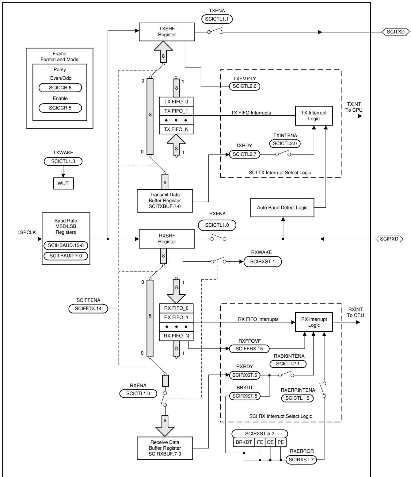
Figure 23-2. Serial Communications Interface (SCI) Module Block Diagram
