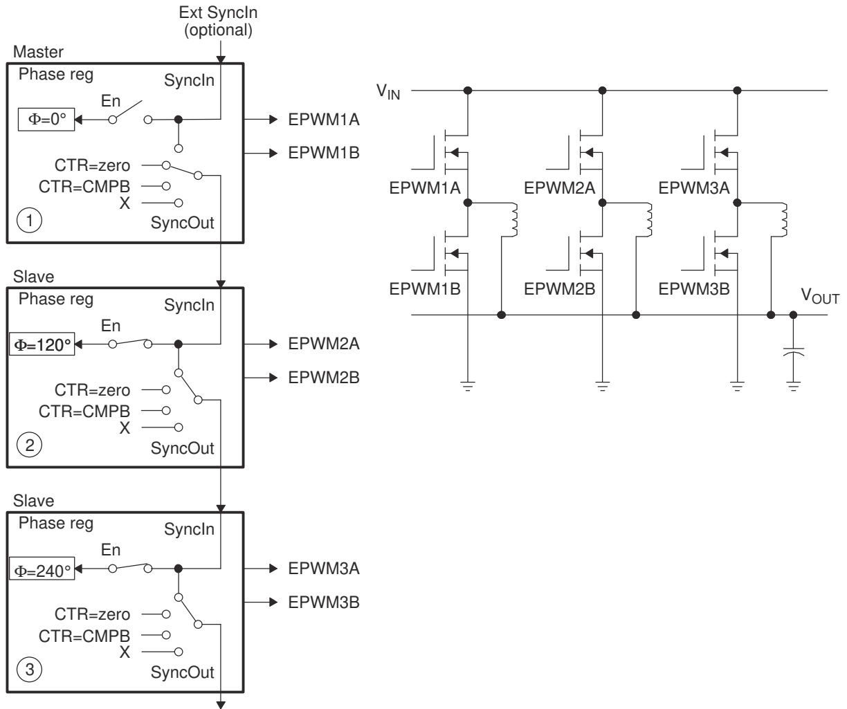
Figure 18-72. Control of a 3-Phase Interleaved DC/DC Converter
