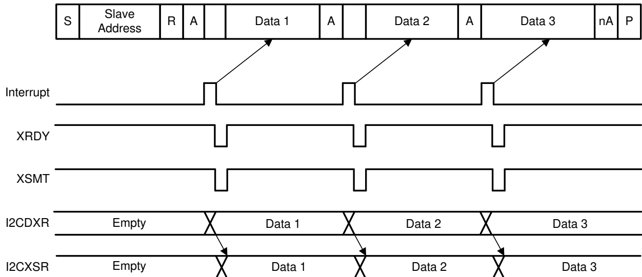
Figure 24-16. Backwards Compatibility Mode Bit, Slave Transmitter
