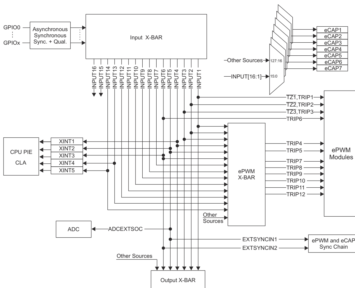
Figure 9-1. Input X-BAR
