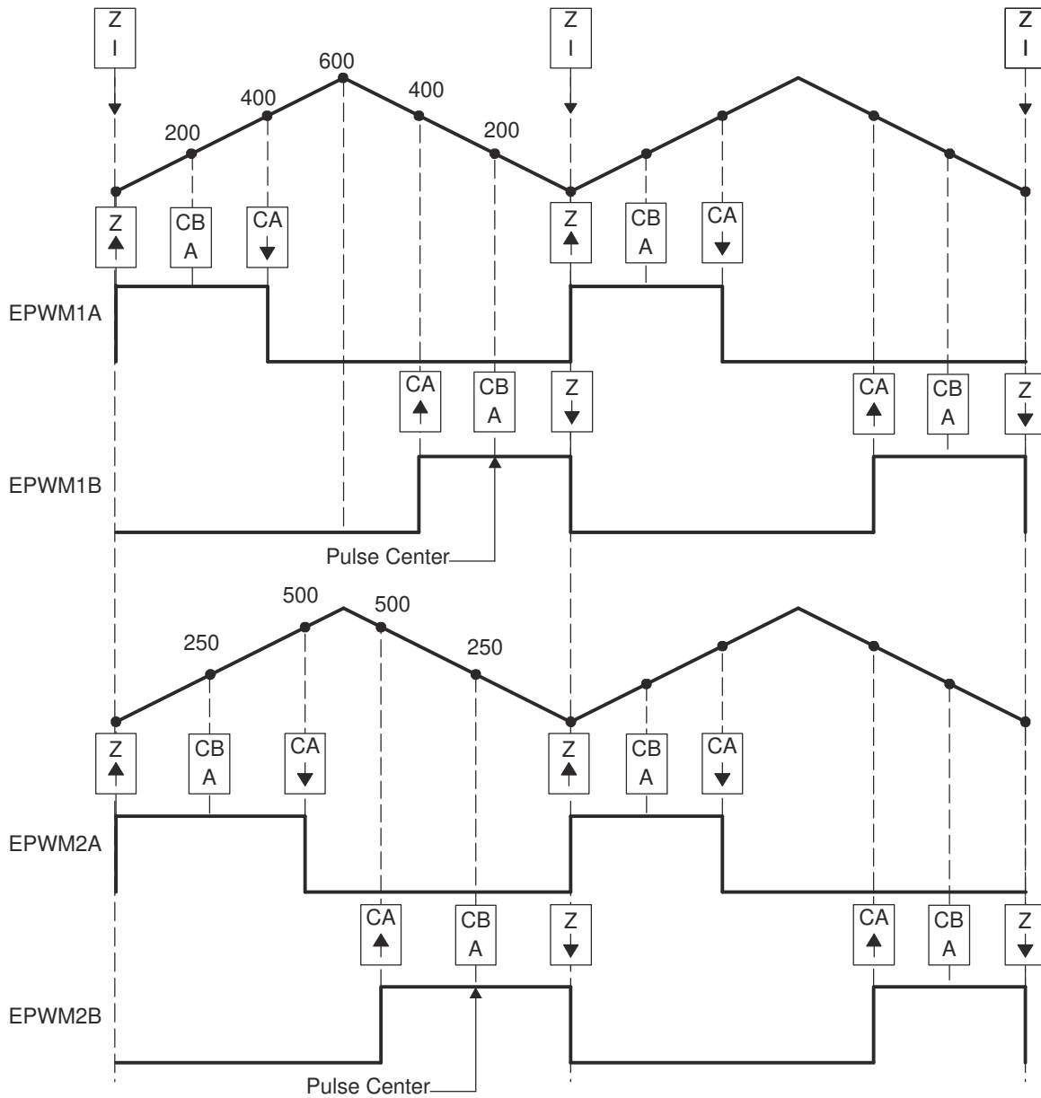
Figure 18-67. Half-H Bridge Waveforms for Figure 18-66 (Note: Here F_{PWM2} = F_{PWM1} )
