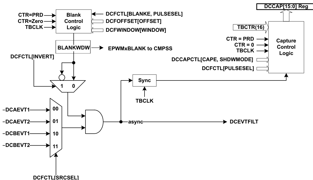
Figure 18-55. Event Filtering
