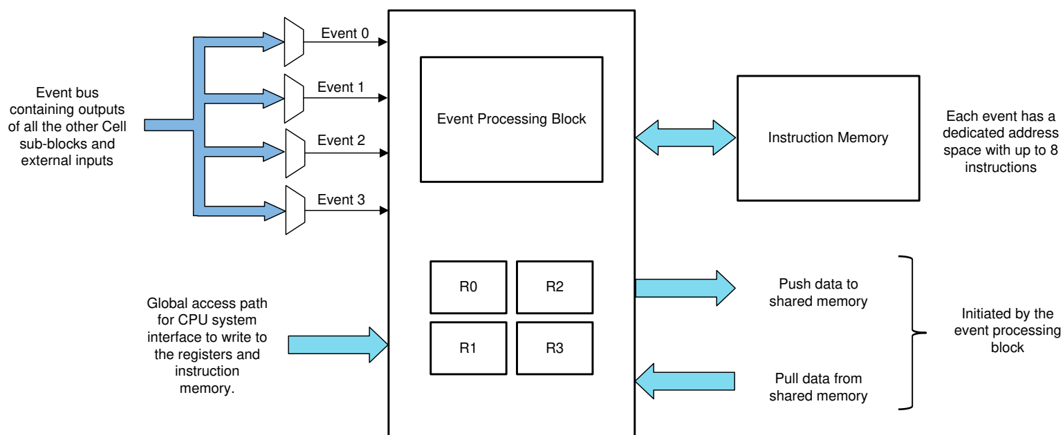
Figure 29-17. High Level Controller Block
