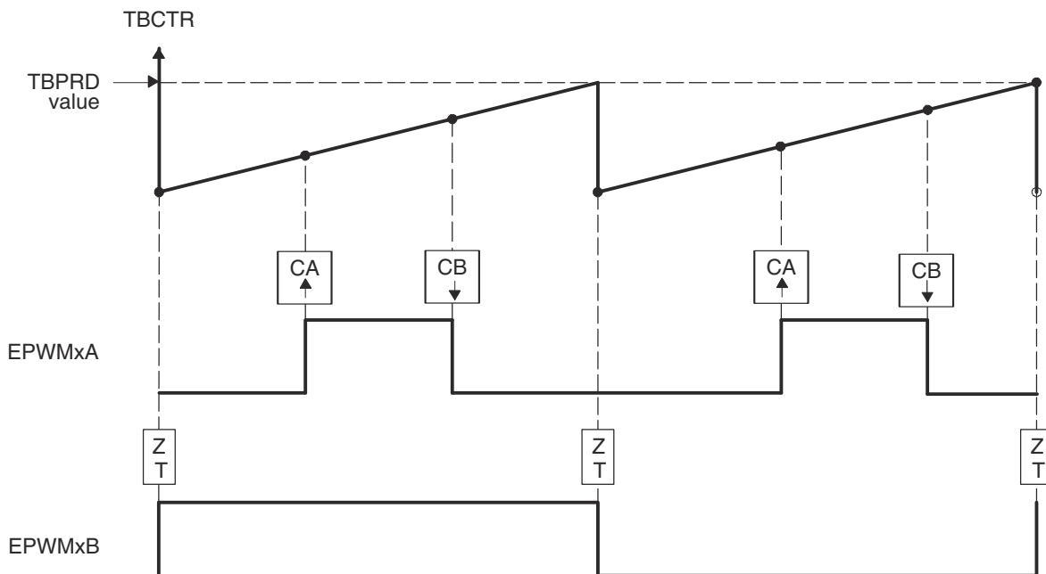
Figure 18-27. Up, Single Edge Asymmetric Waveform With Independent Modulation on EPWMxA and EPWMxB—Active Low
