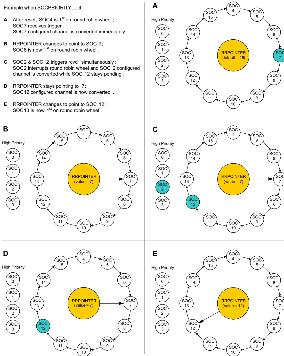
Figure 13-5. High Priority Example
