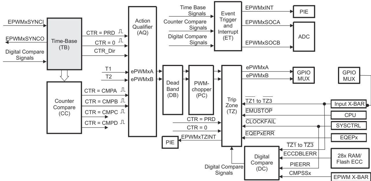
Figure 18-4. Time-Base Submodule
