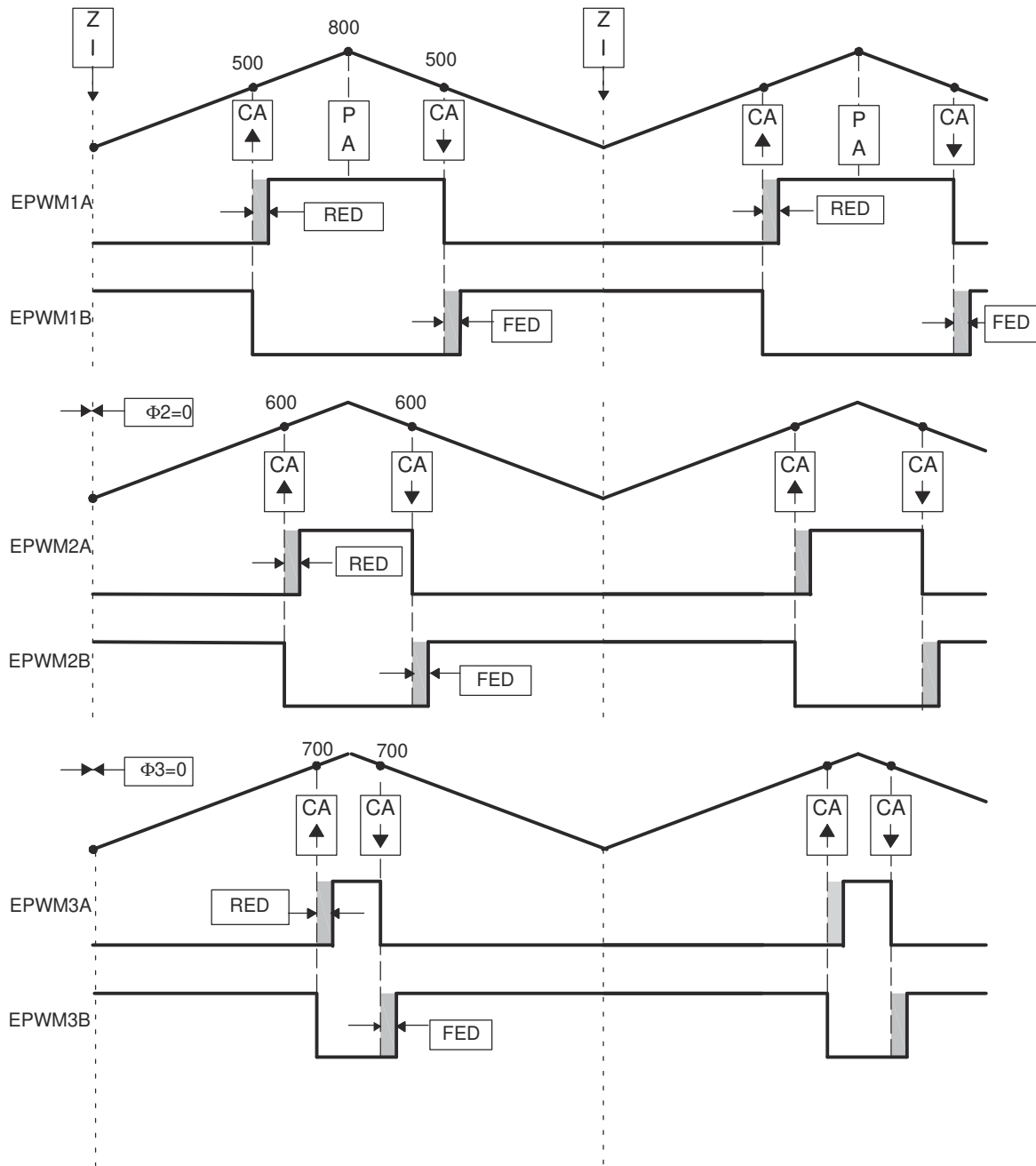
Figure 18-69. 3-Phase Inverter Waveforms for Figure 18-68 (Only One Inverter Shown)
