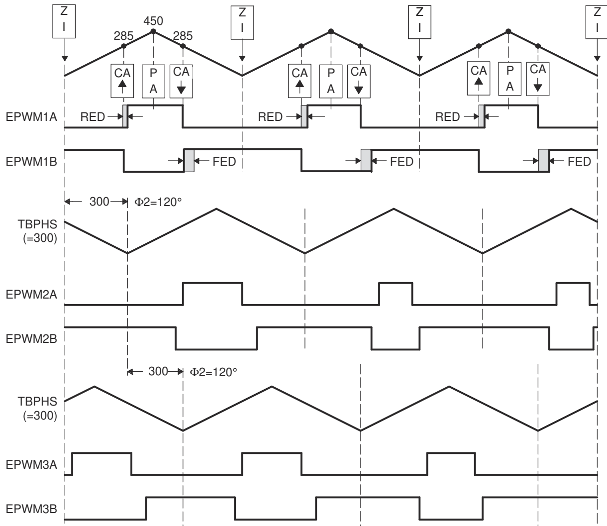
Figure 18-73. 3-Phase Interleaved DC/DC Converter Waveforms for Figure 18-72
