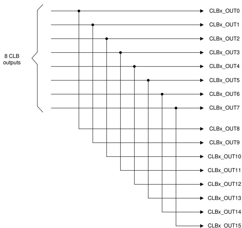
Figure 29-6. CLB Outputs
