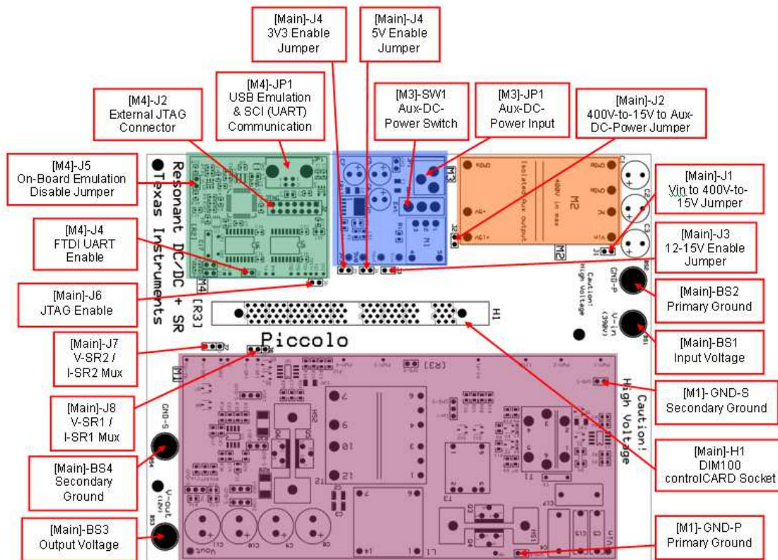
Figure 3. Hardware Features
