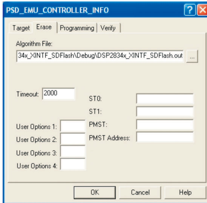
Figure 4. Erase Tab
