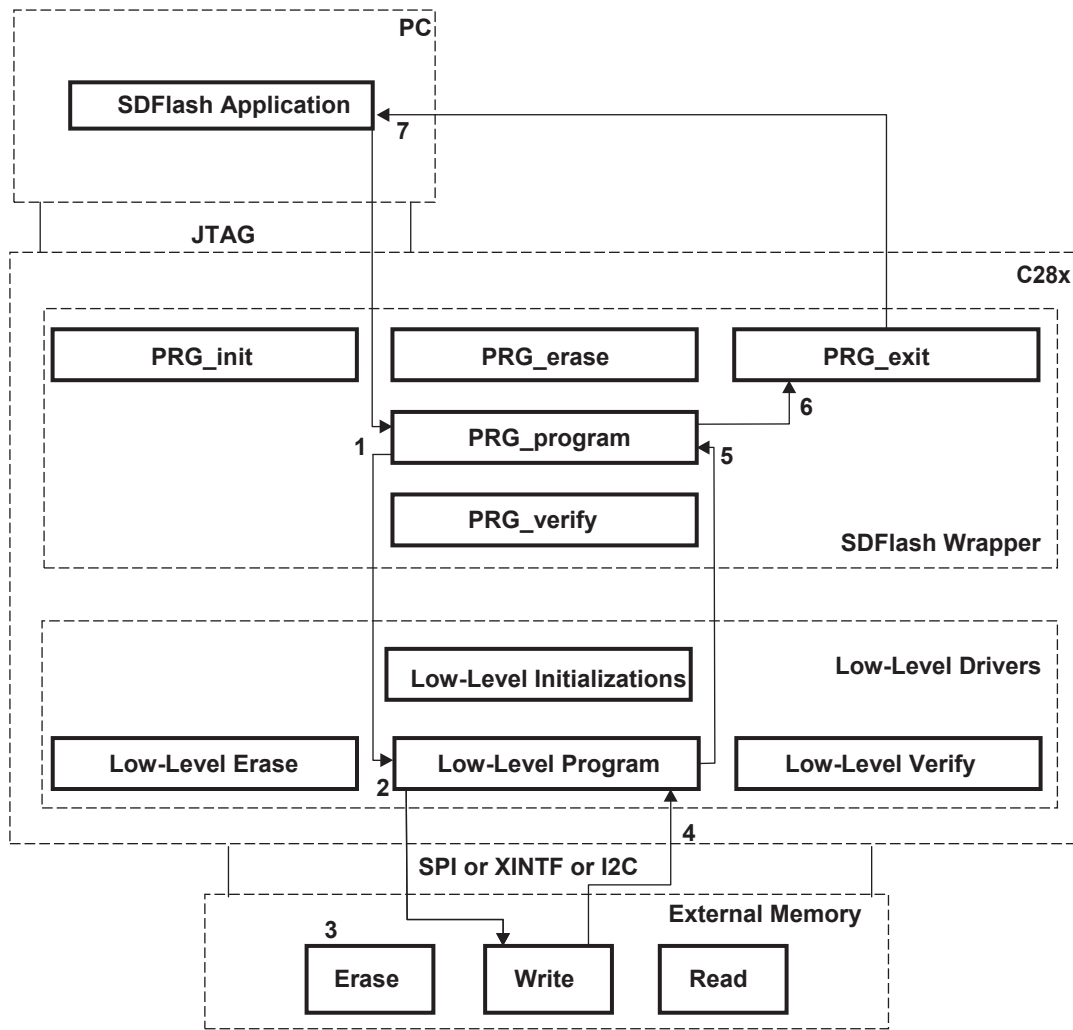
Figure 9. Program Flow
