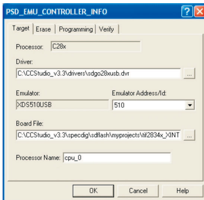
Figure 3. Target Tab
