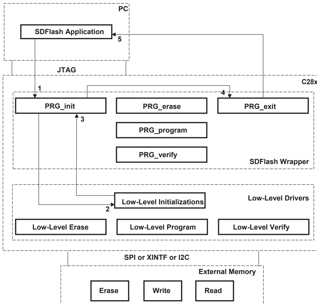
Figure 7. Initializations
