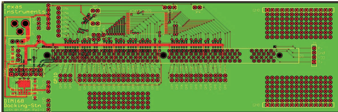
Figure 12. Layout Illustration of Board
