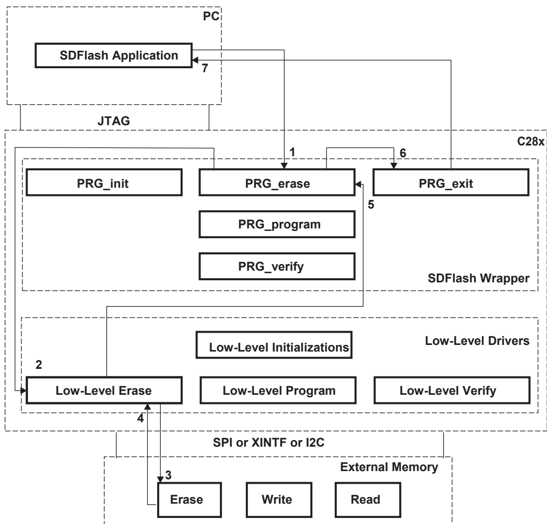
Figure 8. Erase
