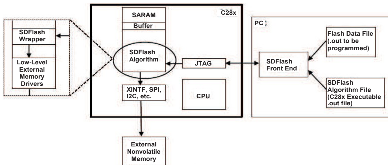
Figure 1. SDFlash Overview
