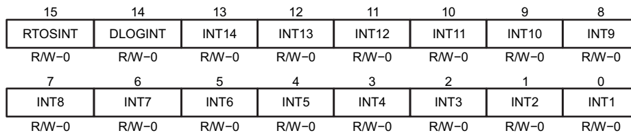
Figure 3-3. Debug Interrupt Enable Register (DBGIER)
