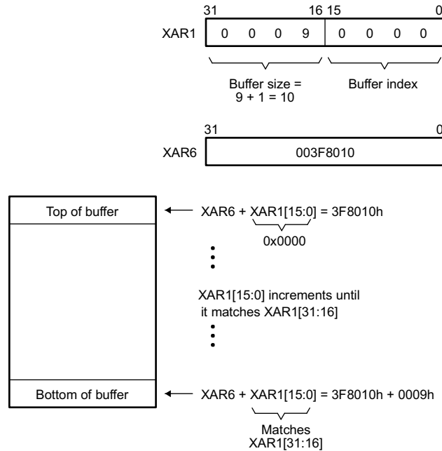
Figure 5-2. Circular Buffer with AMODE = 1
