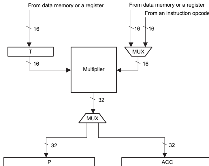
Figure 2-10. Conceptual Diagram of Components Involved in 16 X16-Bit Multiplication
