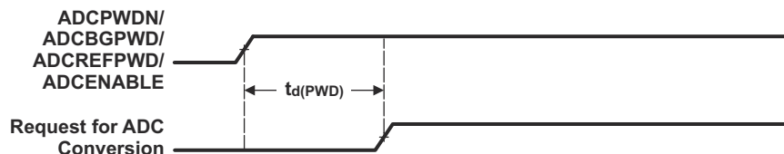
Figure 8-23. ADC Conversion Timing
