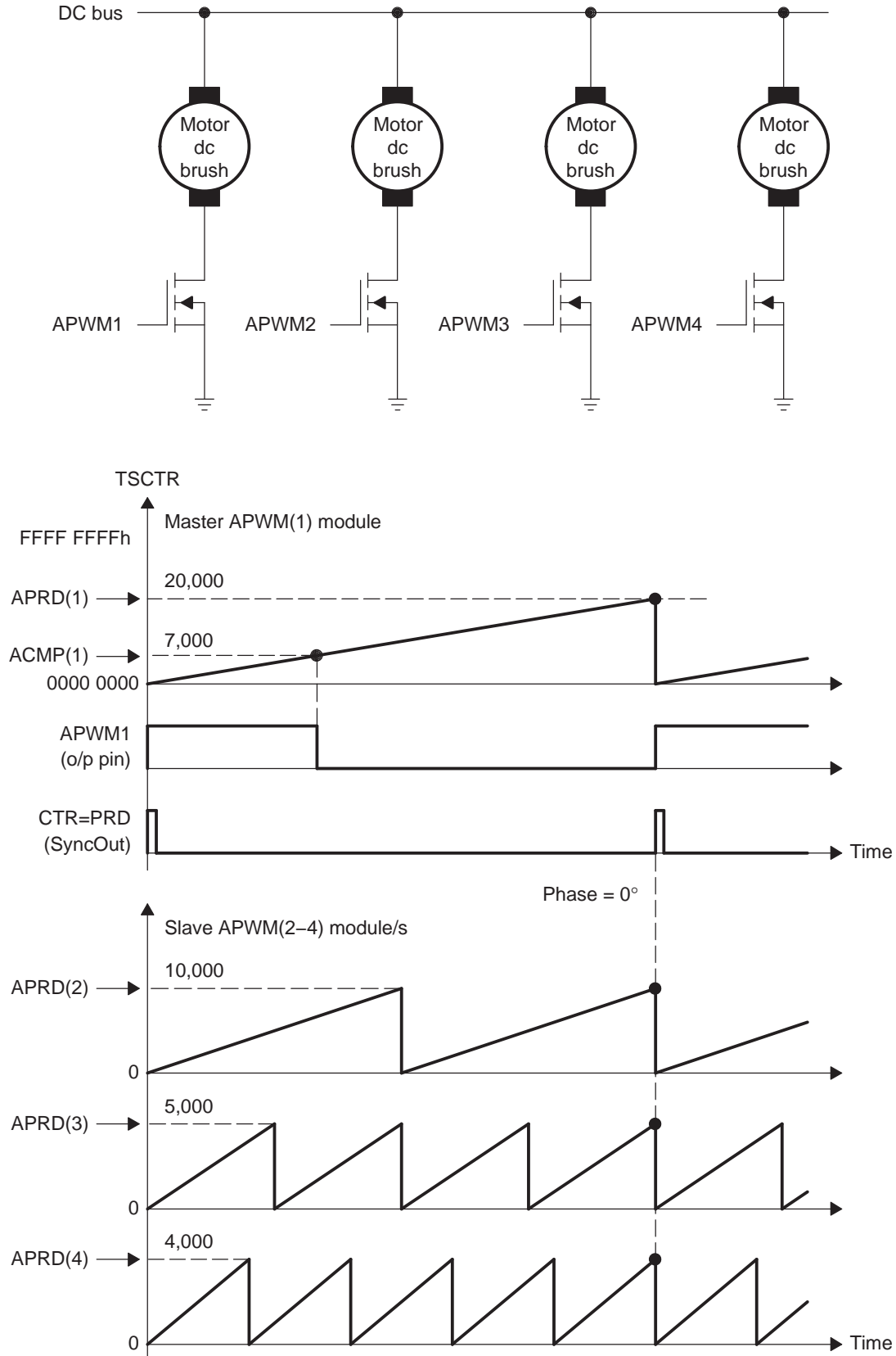
Figure 27. Multichannel PWM Example Using 4 eCAP Modules
