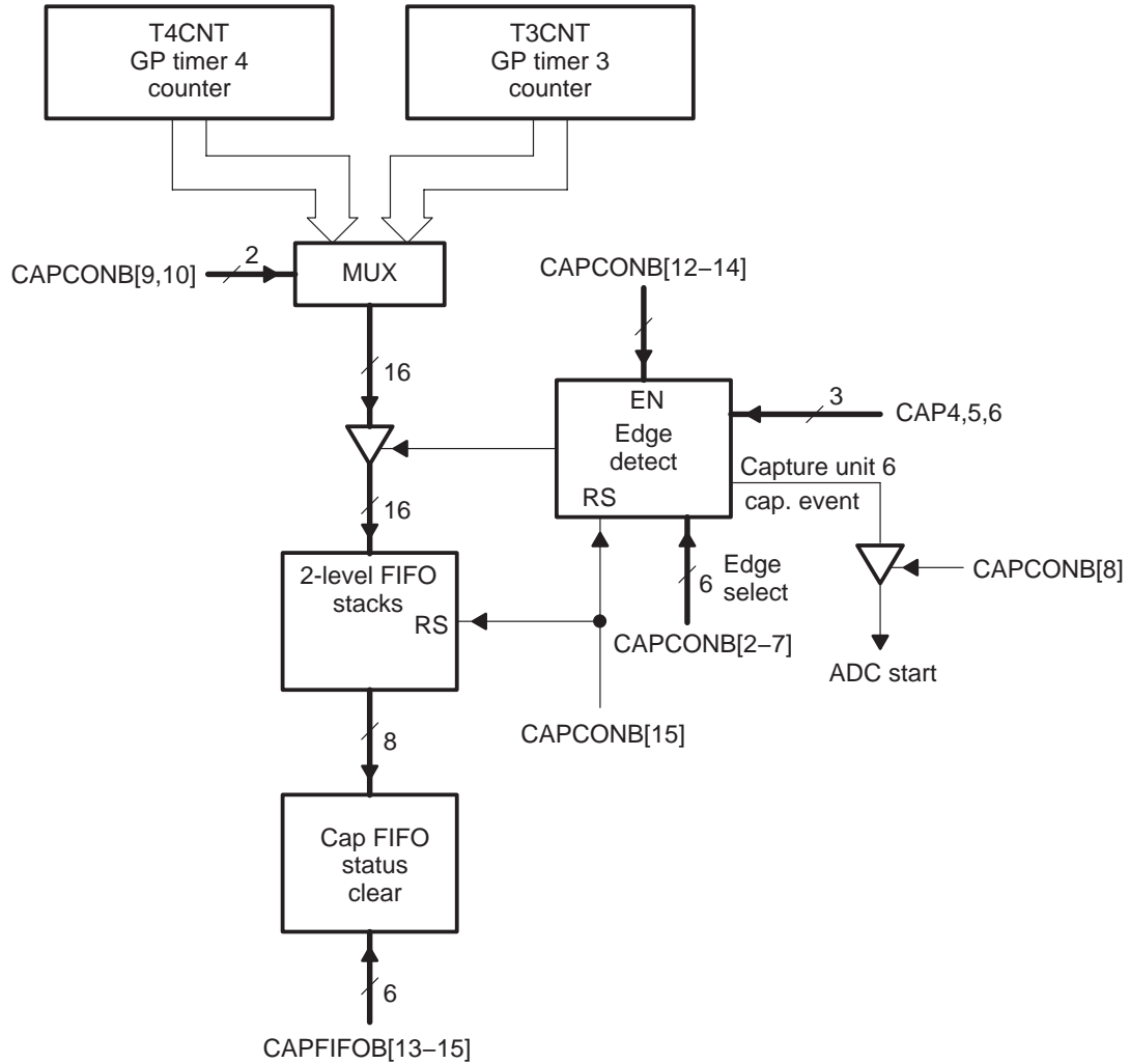
Figure 3–2. Capture Units Block Diagram (EVB)
