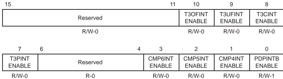
Figure B-26. EVB Interrupt Mask Register A (EVBIMRA) — Address 752Ch
