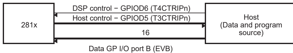
Figure 15. Overview of Parallel GPIO Boot Loader Operation
