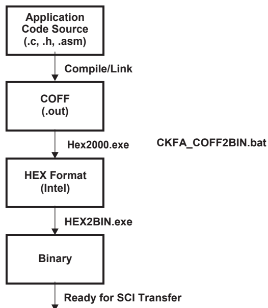
Figure 13. Overview of CKFA File Processing
