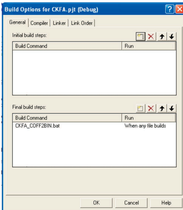
Figure 15. CKFA Project Build Options – Final Build Steps
