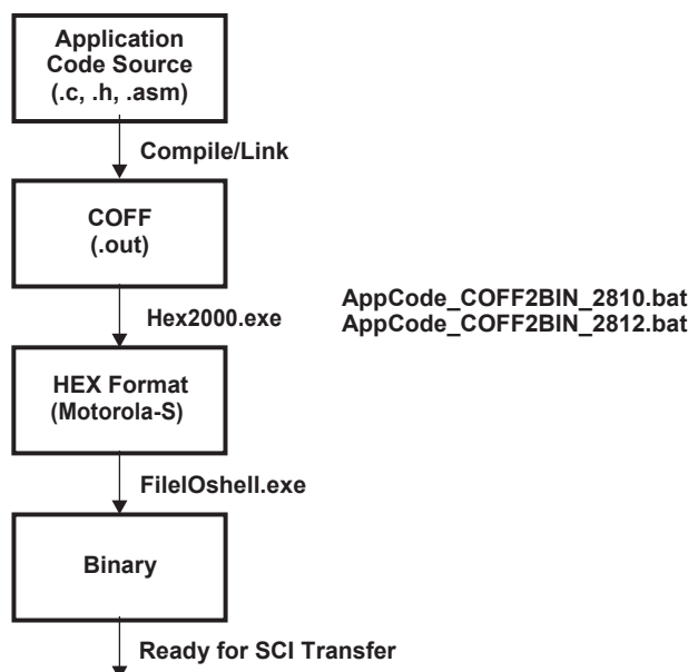
Figure 7. Overview of AppCode File Processing
