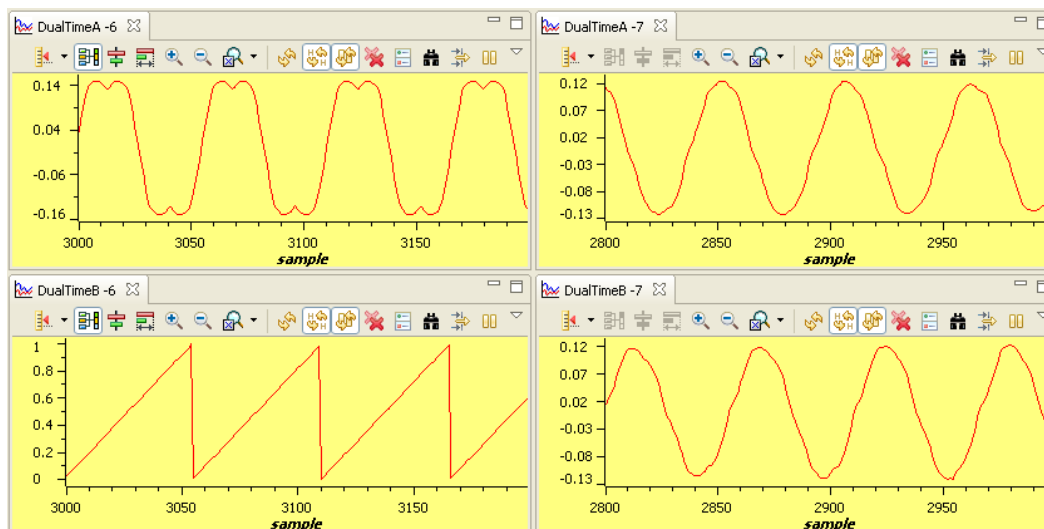
Figure 19. The Waveforms of Svgen_dq1.Ta, rg1.Out, and Phase A and B Currents
