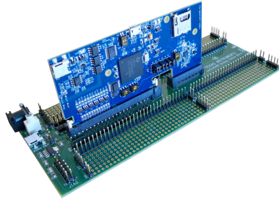
Figure 15: Delfino F28379D Experimenter's Kit (TMDSDOCK28379D) – U.S. $219
