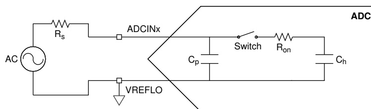
Figure 7-34. Single-Ended Input Model
