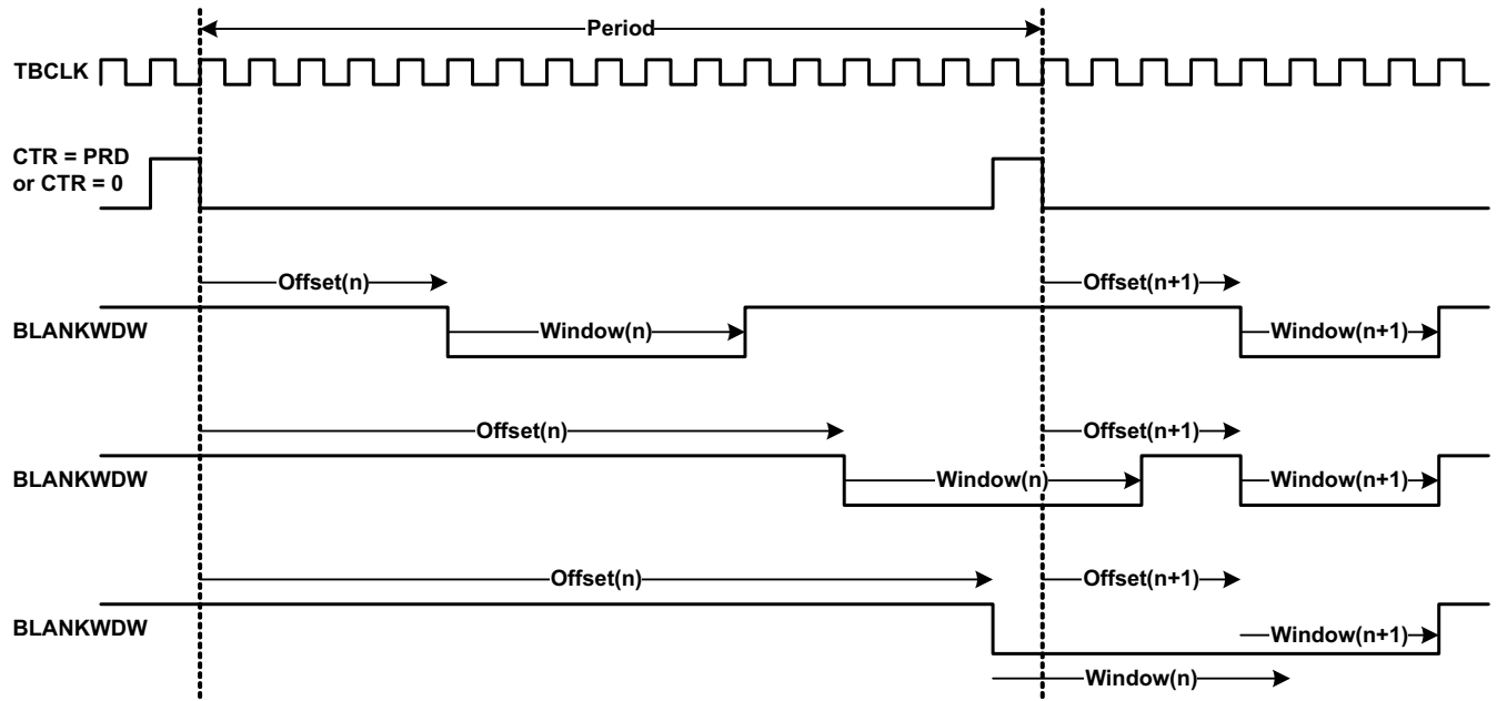
Figure 26-55. Blanking Window Timing Diagram
