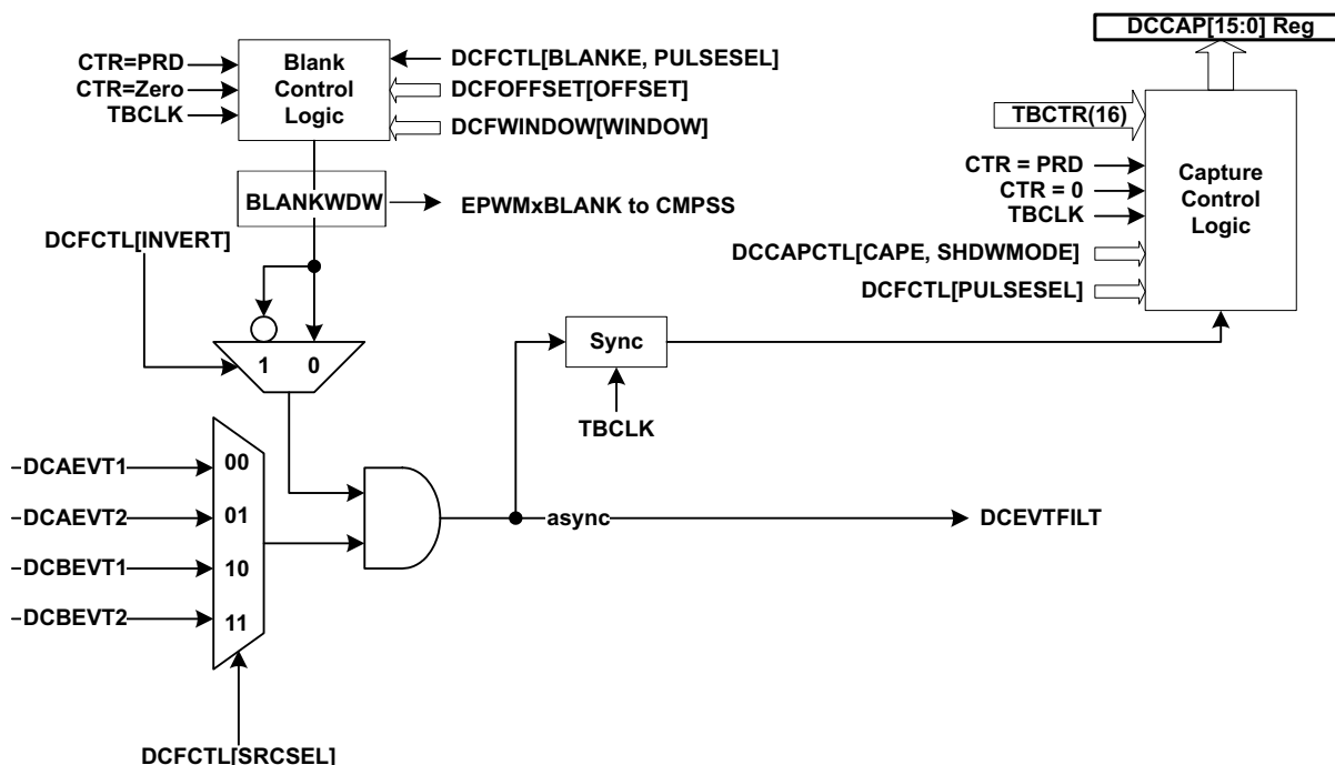
Figure 26-54. Event Filtering
