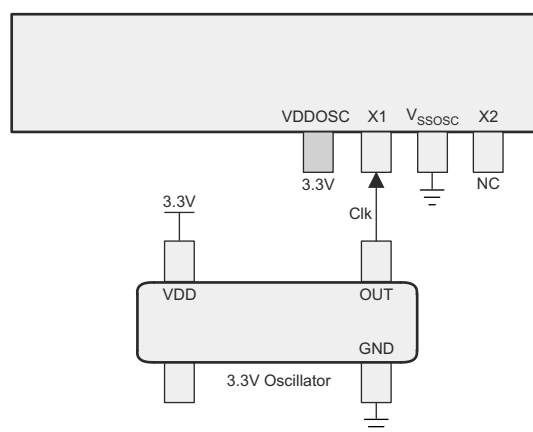
Figure 3-7. Single-ended 3.3V External Clock
