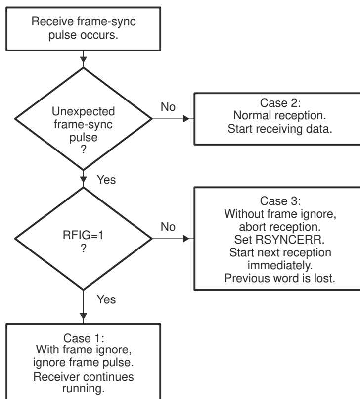
Figure 34-23. Possible Responses to Receive Frame-Synchronization Pulses
