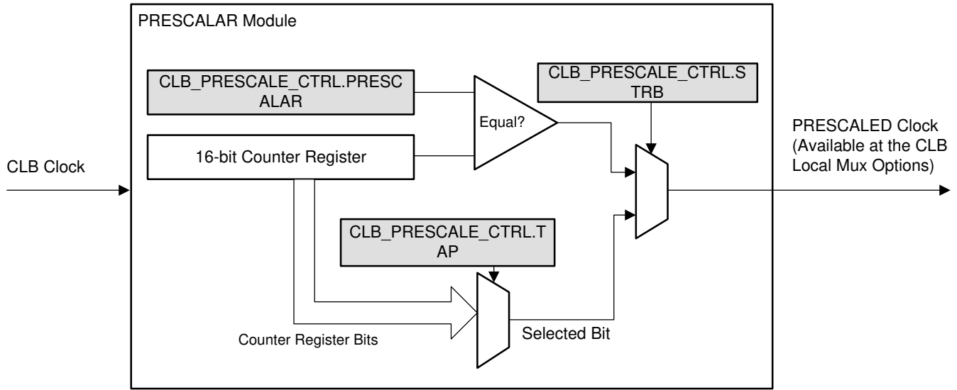
Figure 9-4. CLB Clock Prescalar
