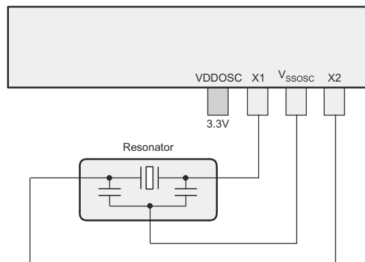
Figure 3-9. External Resonator
