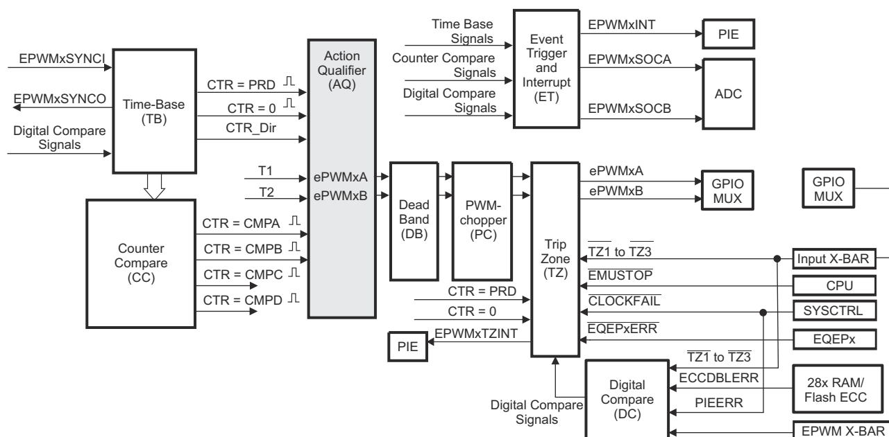
Figure 26-21. Action-Qualifier Submodule
