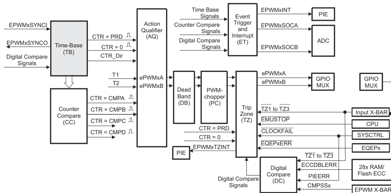
Figure 26-4. Time-Base Submodule
