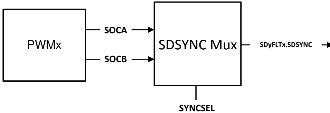
Figure 28-10. SDSYNC Event
