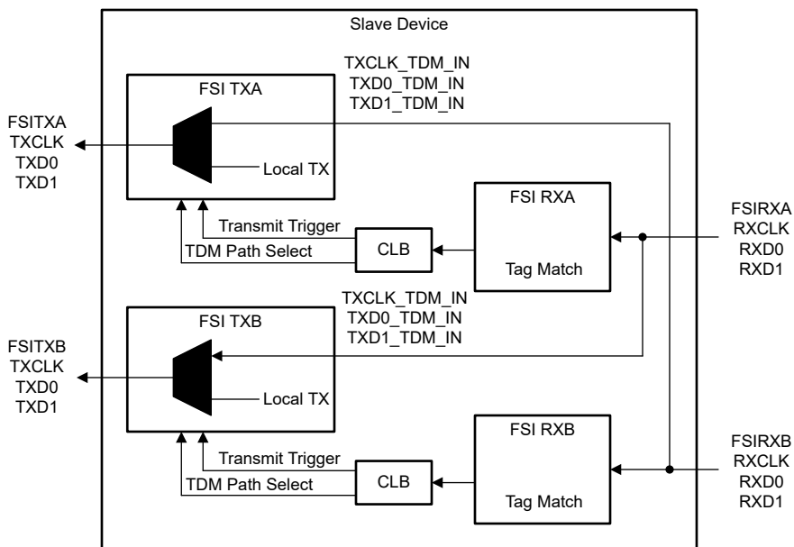
Figure 32-13. FSI and CLB Multi-node TDM Connections
