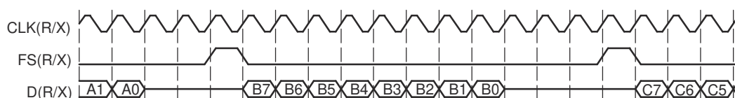
Figure 34-9. Single-Phase Frame for a McBSP Data Transfer
