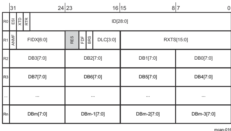
Figure 45-19. Rx Buffer/Rx FIFO Element Structure
