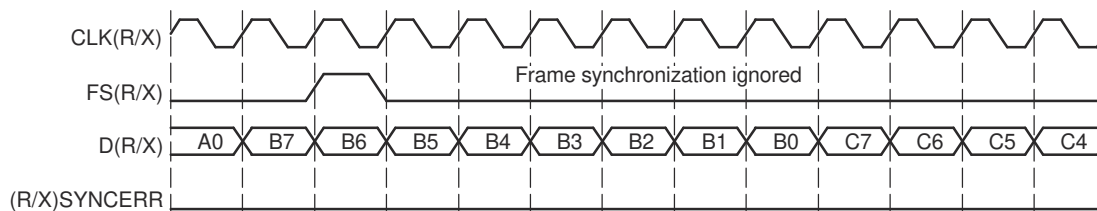
Figure 34-44. Unexpected Frame-Synchronization Pulse With (R/X)FIG = 1
