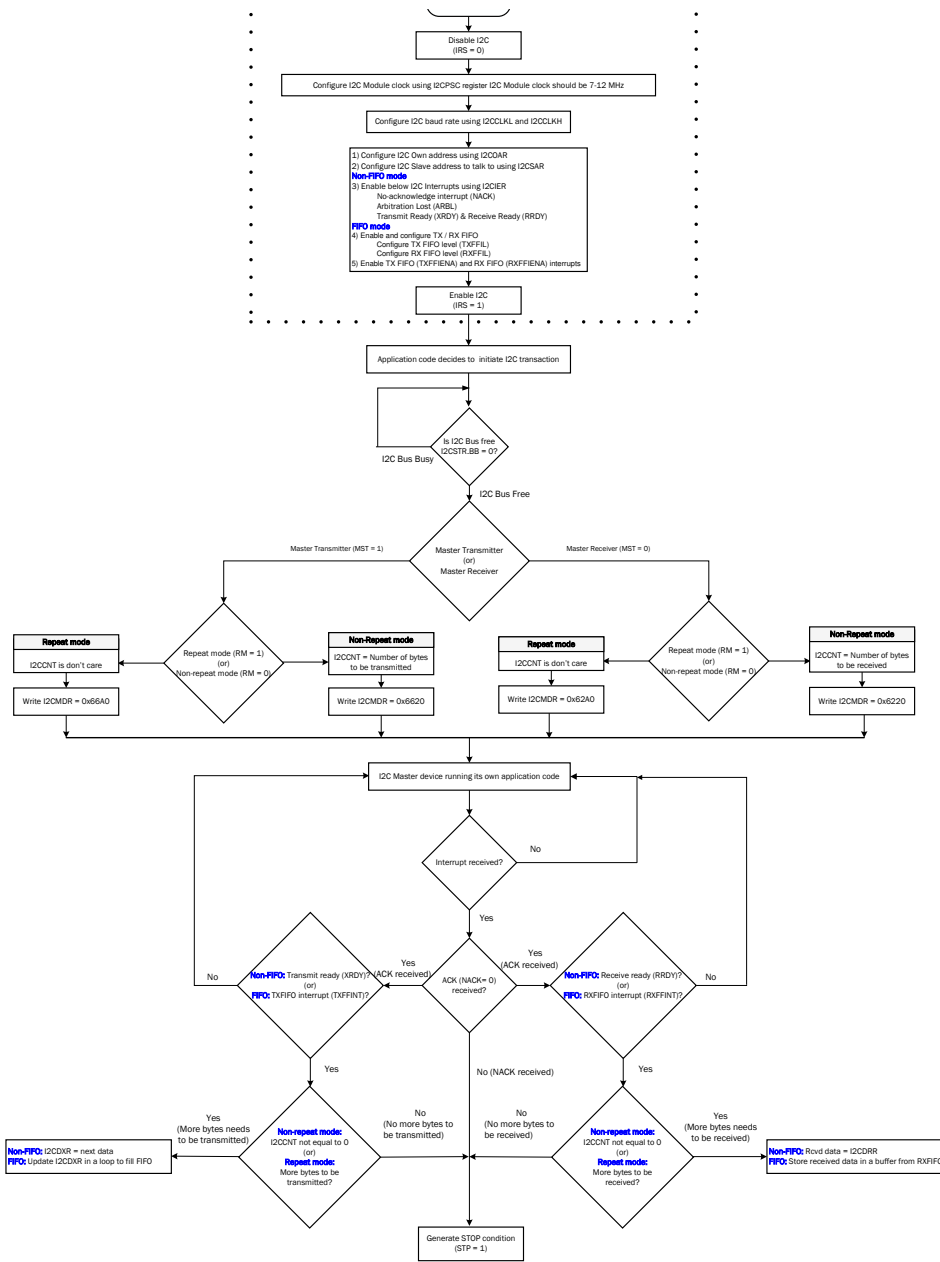
Figure 33-7. I2C Master TX / RX Flowchart
