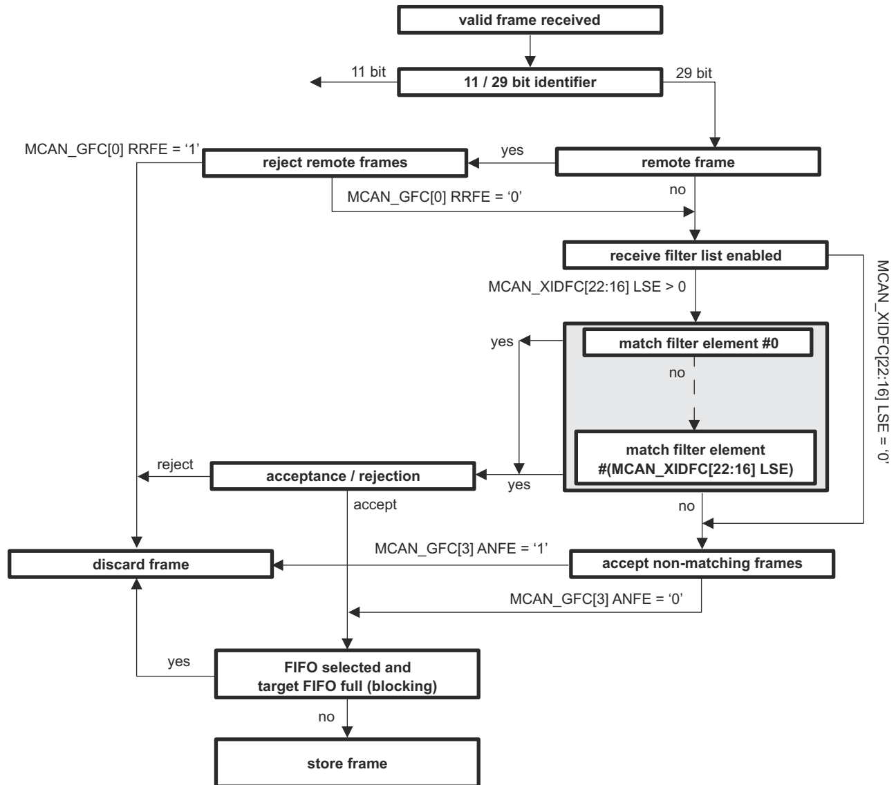
Figure 45-13. Extended Message ID Filter Path
