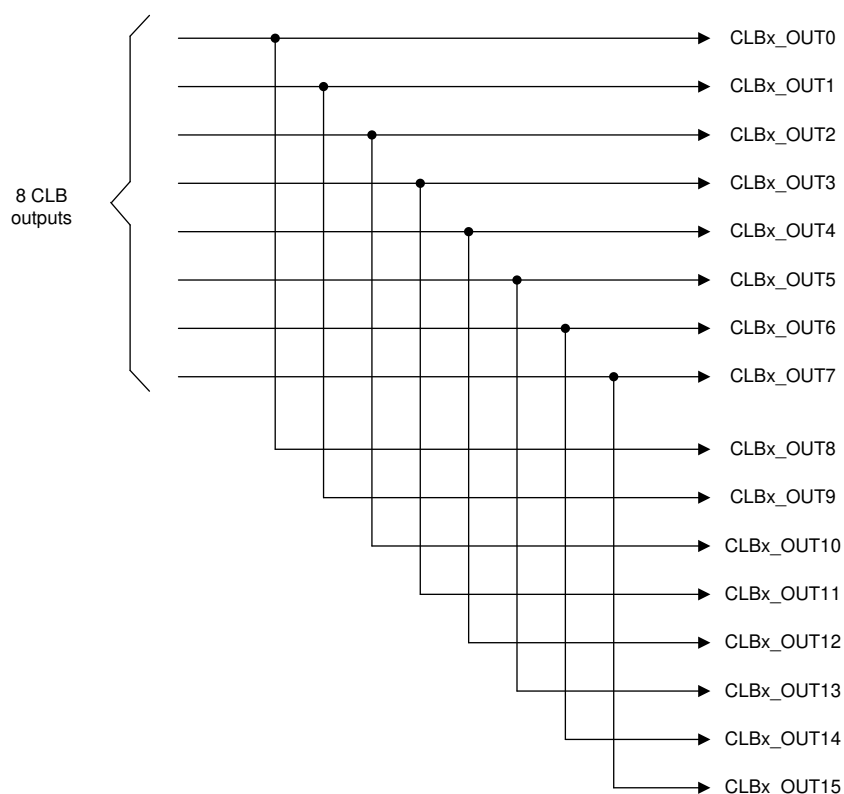
Figure 9-7. CLB Outputs
