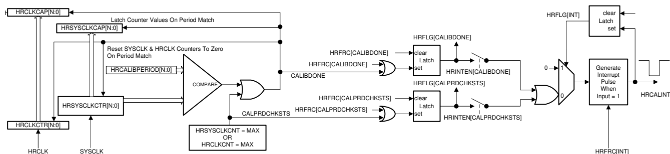
Figure 25-2. HRCAP Calibration
