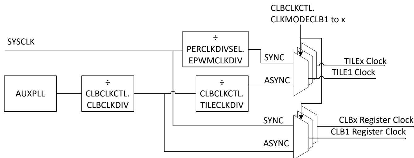
Figure 9-3. CLB Clocking
