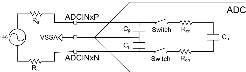
Figure 20-4. Differential Input Model
