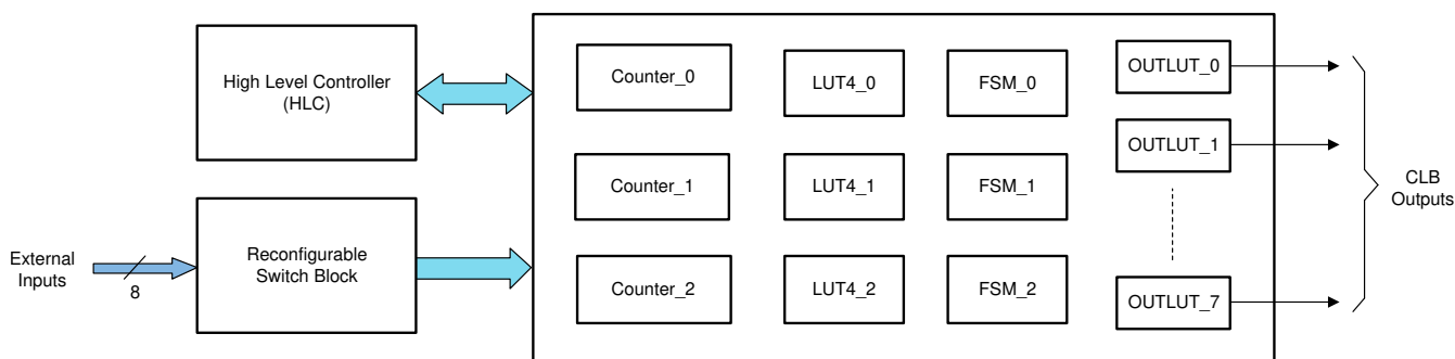
Figure 9-9. CLB Tile Submodules
