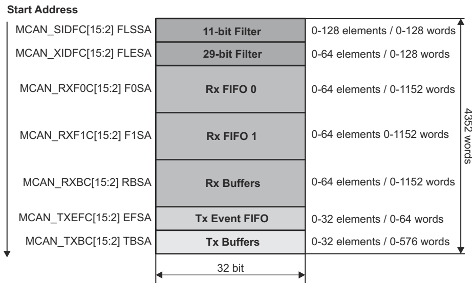
Figure 45-18. Message RAM Configuration
