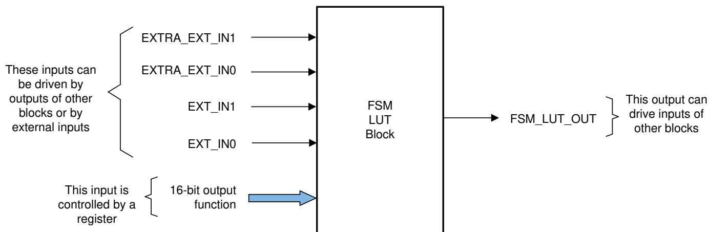
Figure 9-13. FSM LUT Block
