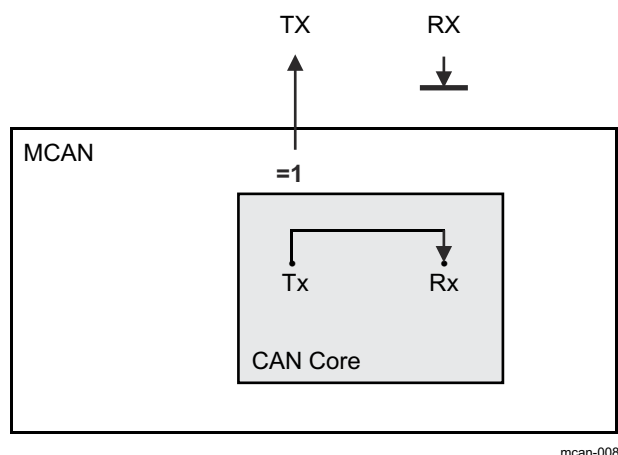
Figure 45-10. Internal Loop Back Mode
