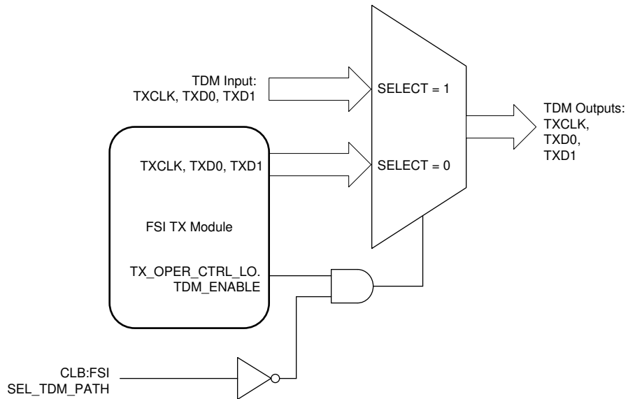
Figure 32-11. FSI Transmitter Multi-node TDM Multiplexing
