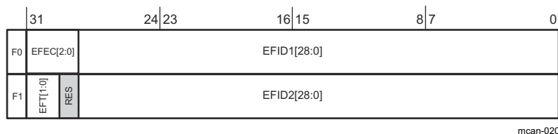
Figure 45-23. Extended Message ID Filter Element Structure
