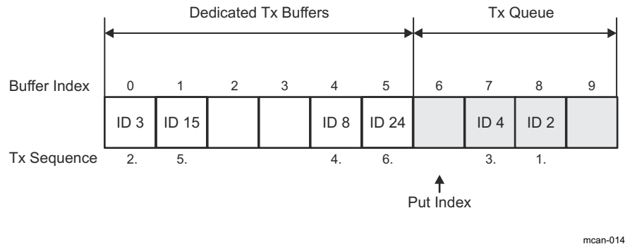
Figure 45-17. Mixed Dedicated Tx Buffers /Tx Queue (example)
