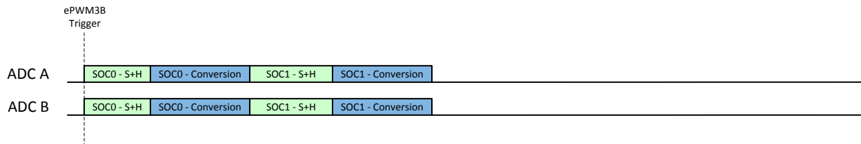
Figure 20-17. Example: Basic Synchronous Operation
