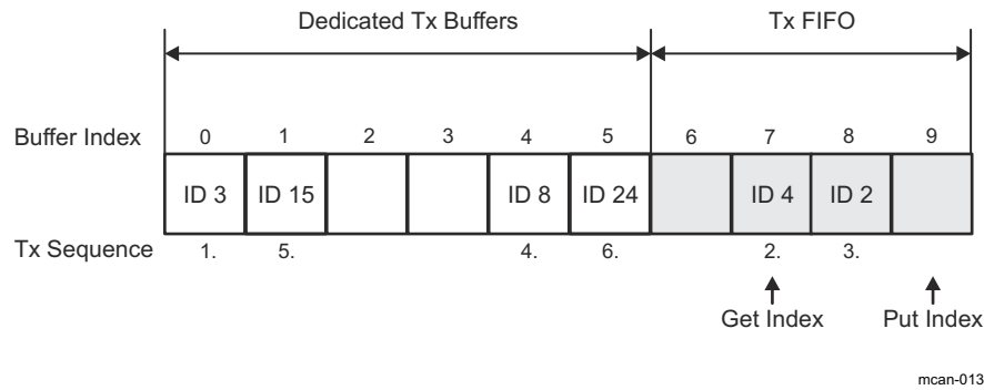
Figure 45-16. Mixed Dedicated Tx Buffers /Tx FIFO (example)
