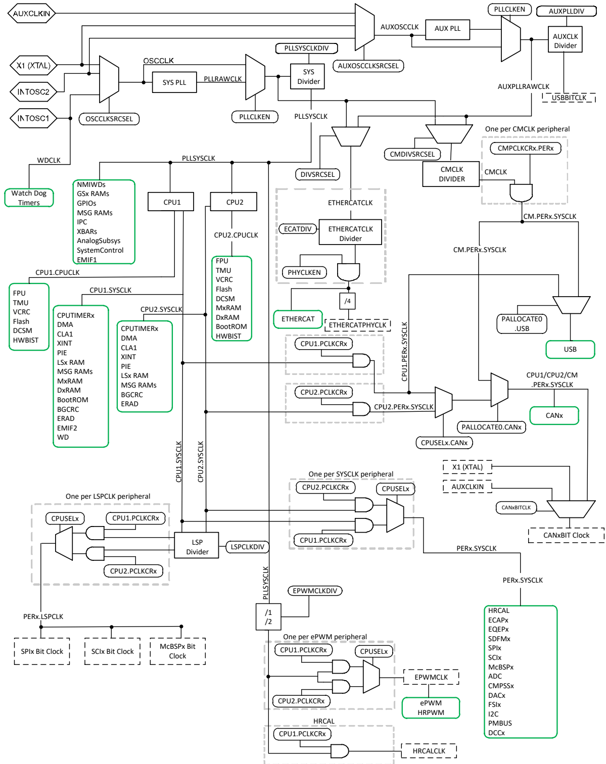
Figure 3-6. Clocking System
