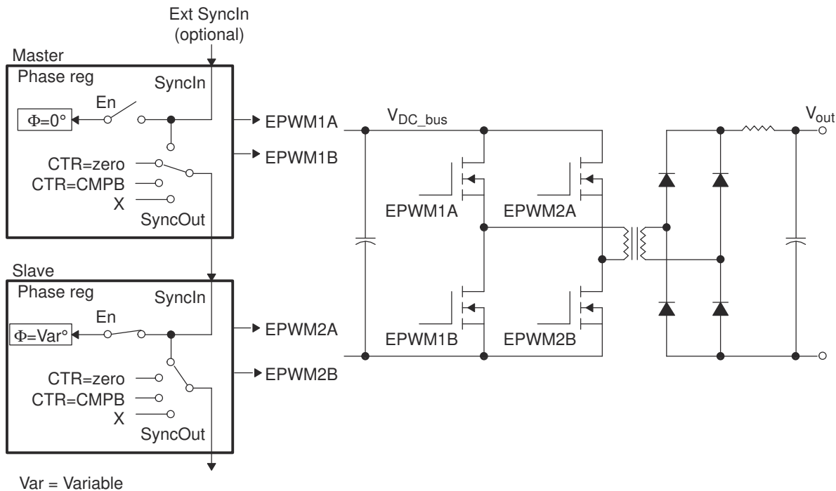
Figure 26-72. Controlling a Full-H Bridge Stage ( F_{PWM2} = F_{PWM1} )
