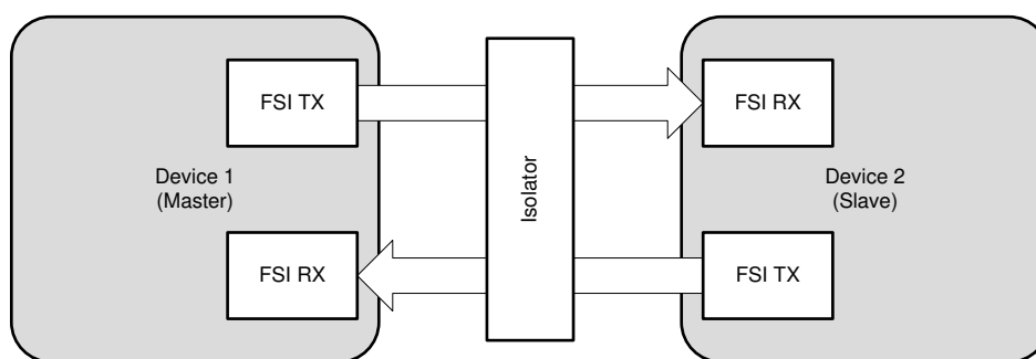
Figure 32-17. Point to Point Connection
