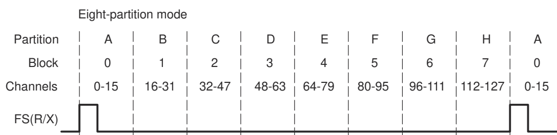
Figure 34-34. McBSP Data Transfer in the 8-Partition Mode
