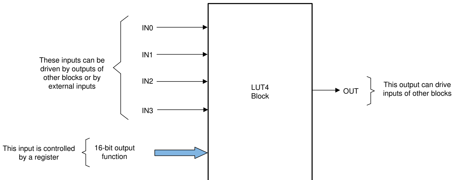
Figure 9-14. LUT4 Block
