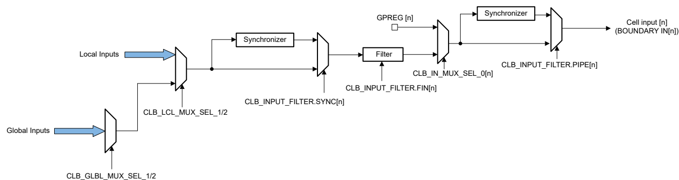
Figure 9-5. CLB Input Mux and Filter
