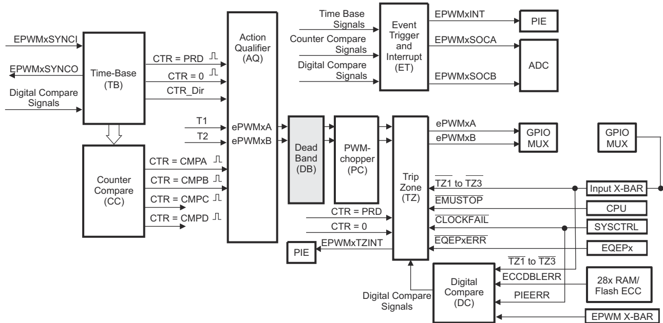
Figure 26-34. Dead_Band Submodule
