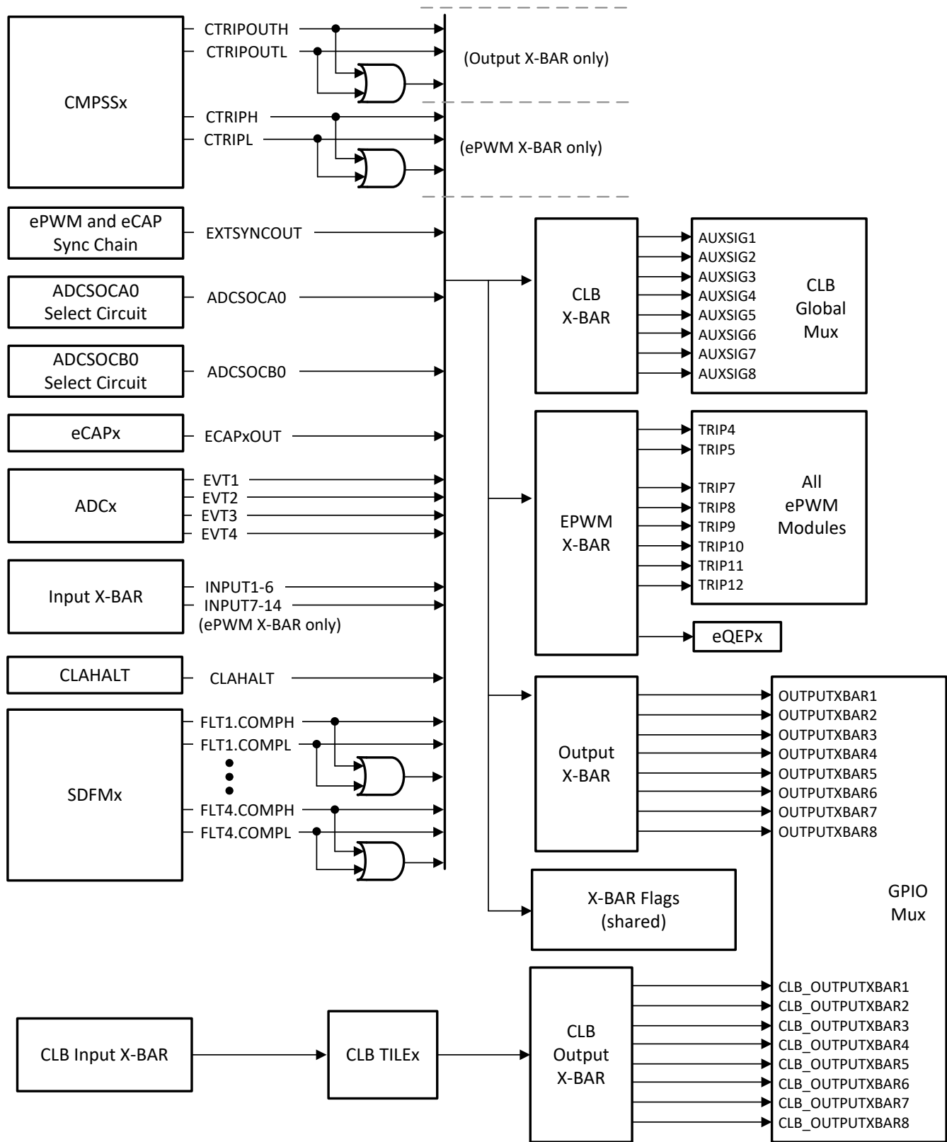
Figure 17-5. ePWM and Output X-BARs Sources
