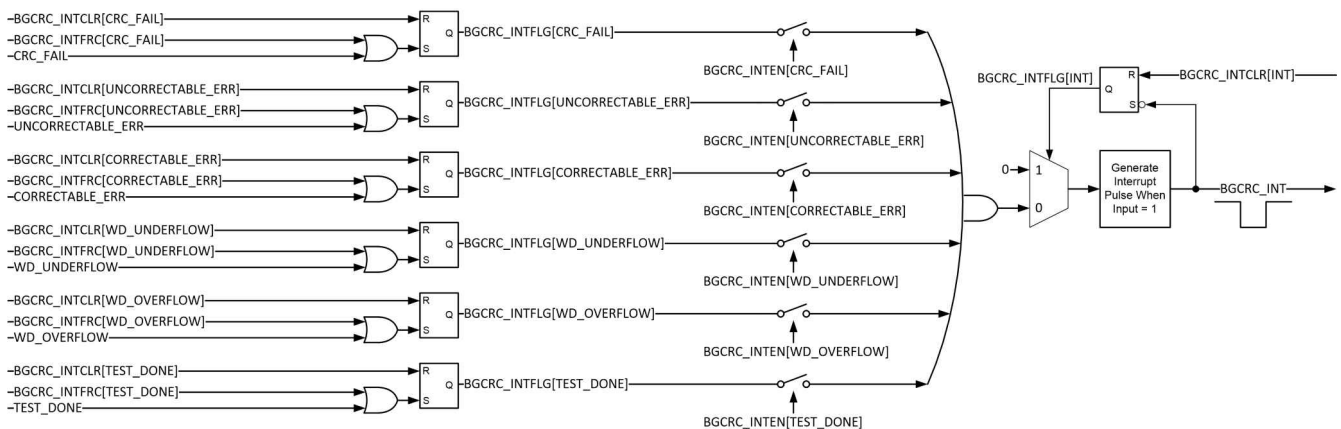
Figure 7-4. BGCR_C Interrupt
