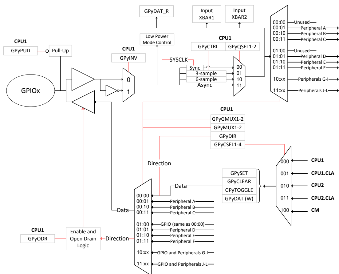
Figure 15-1. GPIO Logic for a Single Pin
