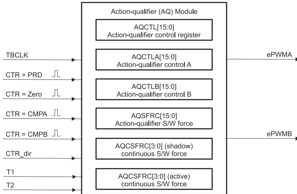
Figure 26-22. Action-Qualifier Submodule Inputs and Outputs
