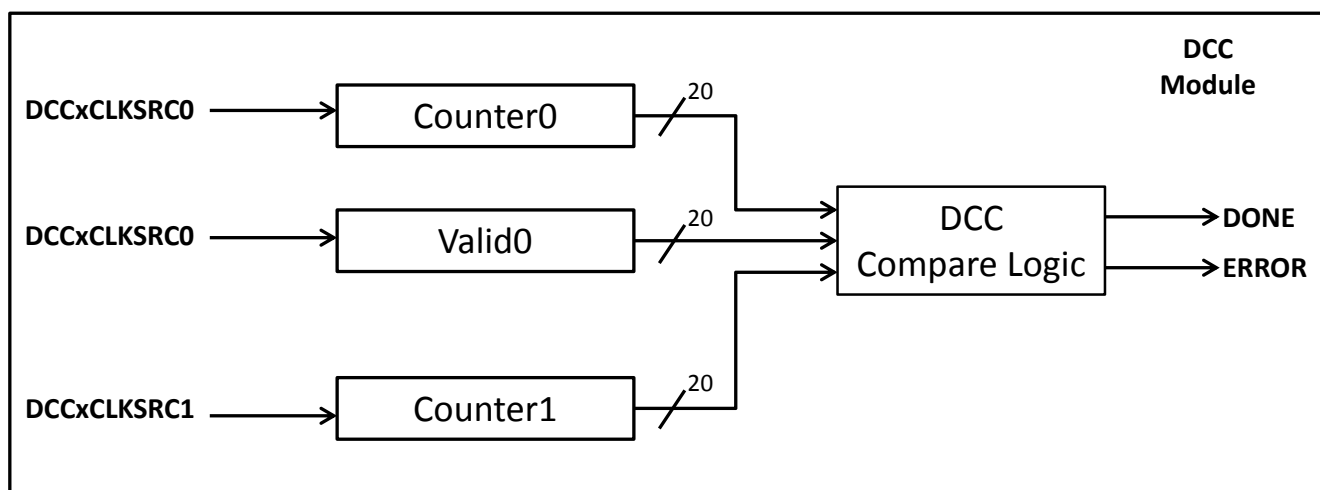
Figure 10-1. DCC Operation
