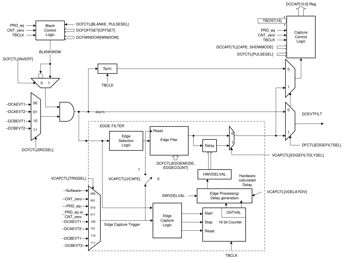
Figure 26-56. Valley Switching
