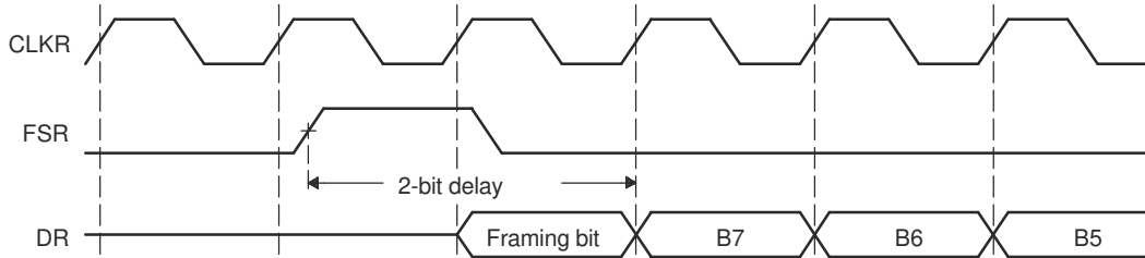
Figure 34-57. 2-Bit Data Delay Used to Skip a Framing Bit
