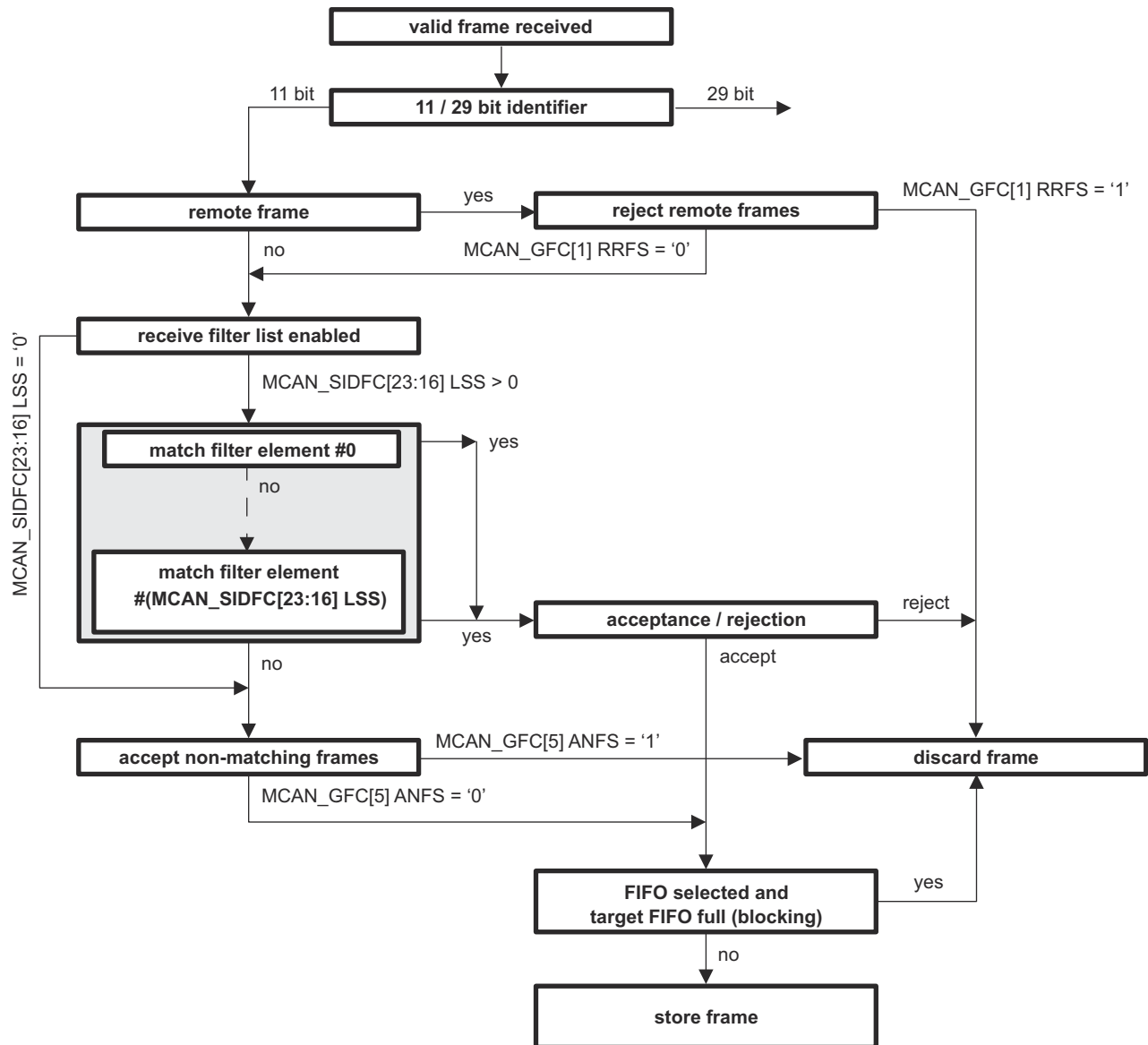
Figure 45-12. Standard Message ID Filter Path
