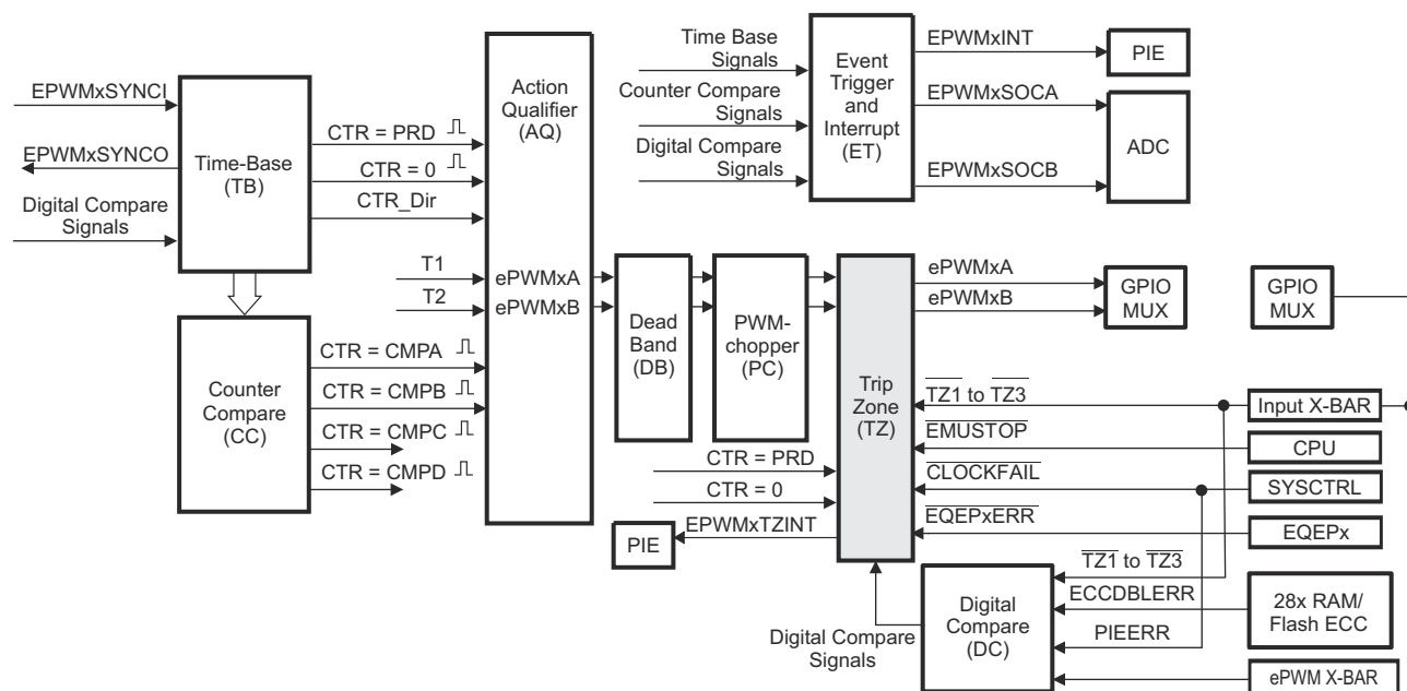
Figure 26-42. Trip-Zone Submodule
