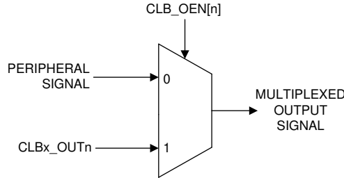
Figure 9-8. Peripheral Signal Multiplexer
