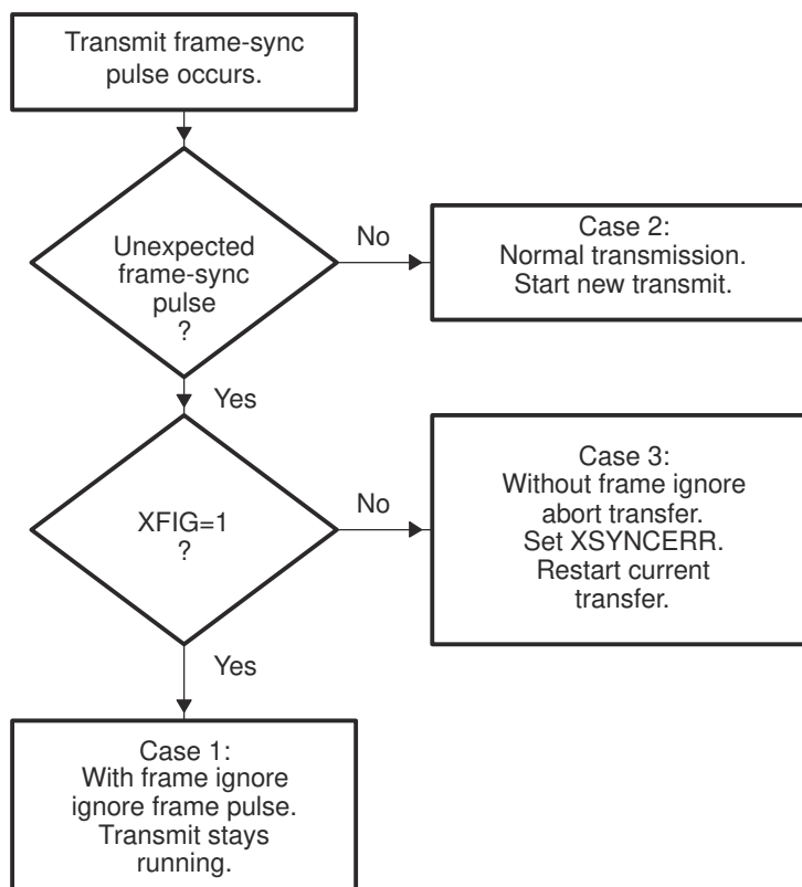
Figure 34-29. Possible Responses to Transmit Frame-Synchronization Pulses
