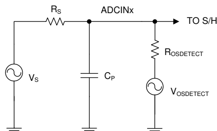
Figure 20-12. Input Circuit Equivalent with OSDETECT Enabled
