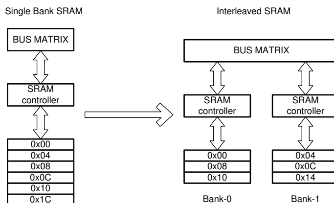
Figure 41-7. Interleaving
