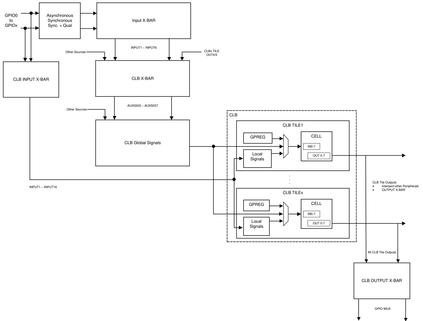
Figure 9-6. GPIO to CLB Tile Connections
