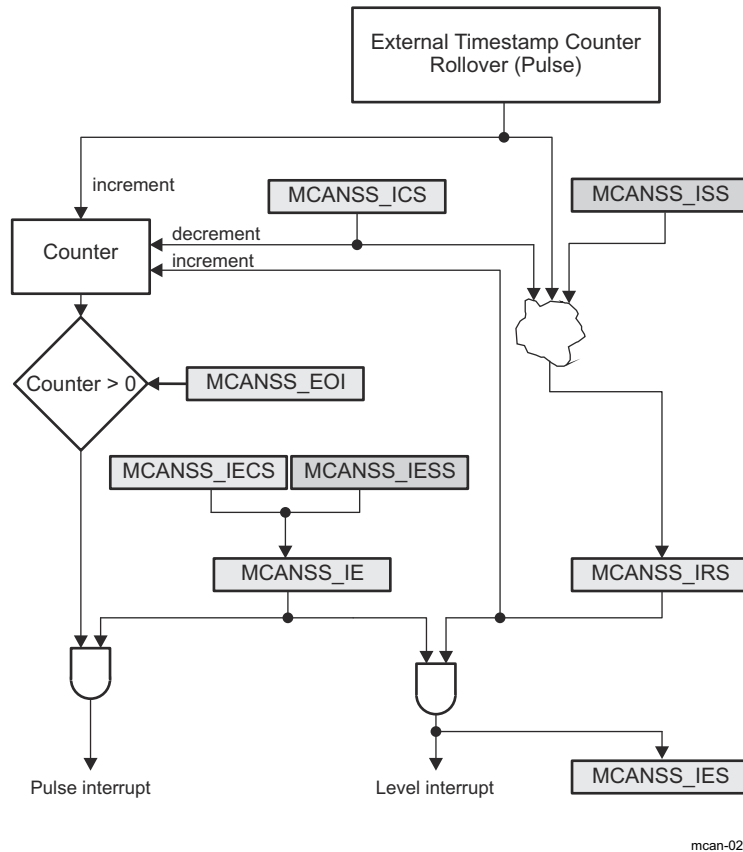
Figure 45-11. External Timestamp Counter Interrupt
