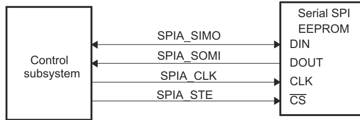
Figure 5-8. SPI Loader
