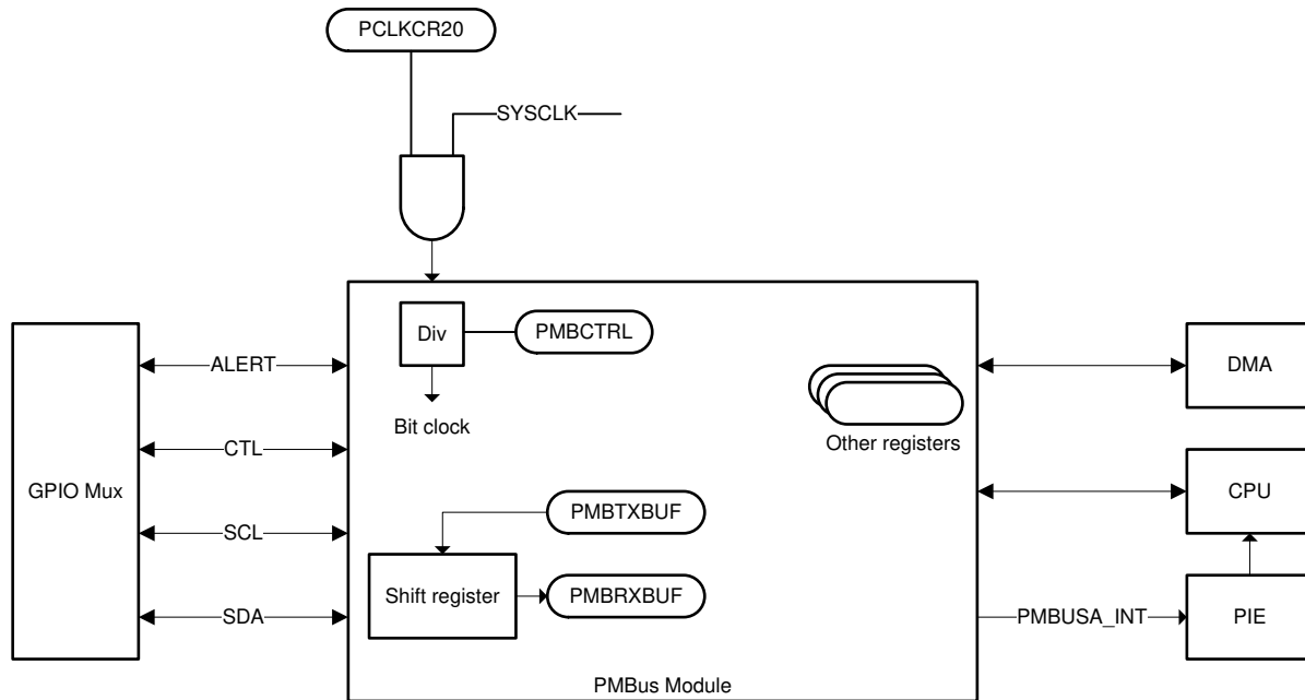
Figure 35-1. PMBus Module Block Diagram
