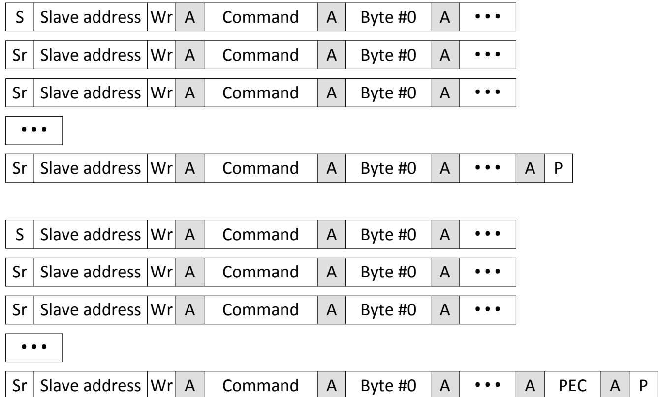
Figure 35-27. Group Command Message With and Without PEC
