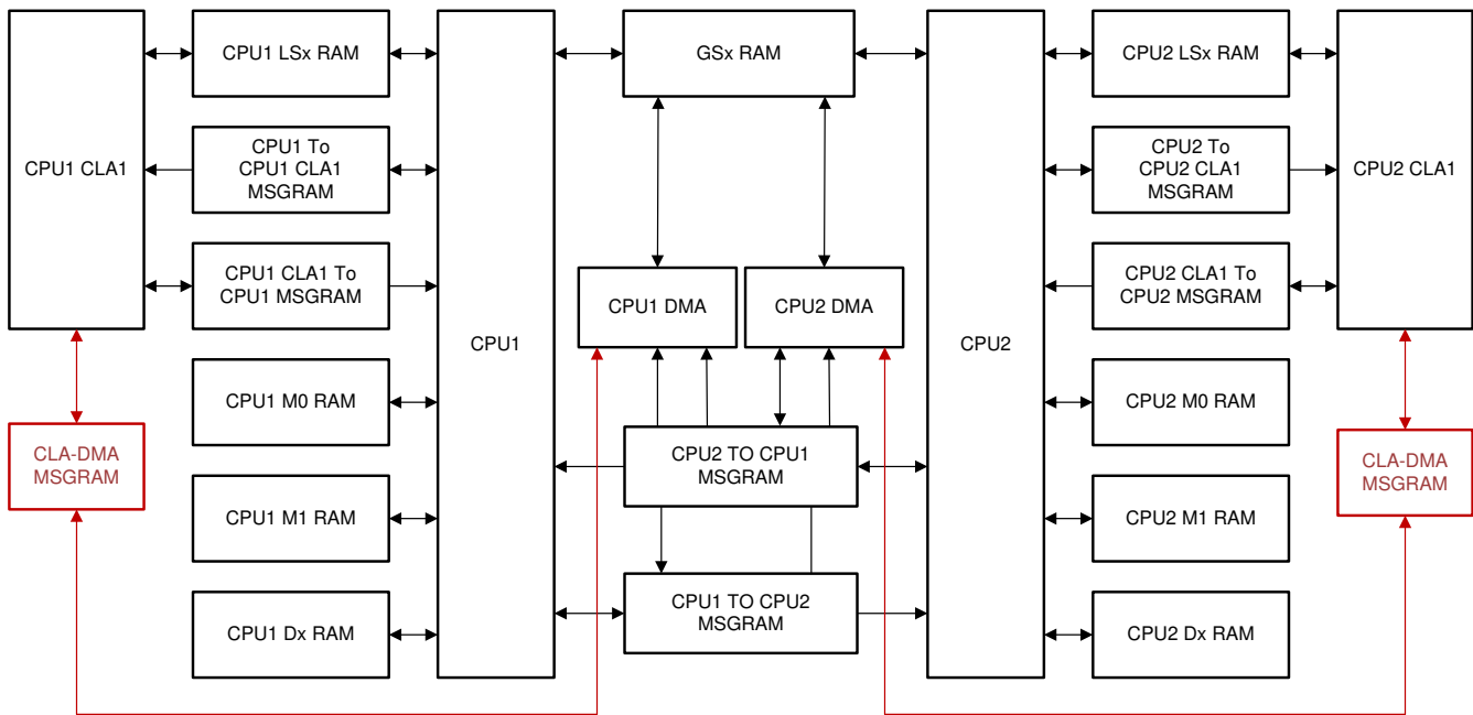
Figure 3-16. Memory Architecture
