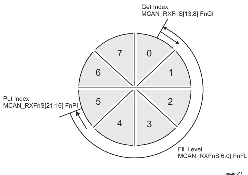
Figure 45-14. Rx FIFO Status
