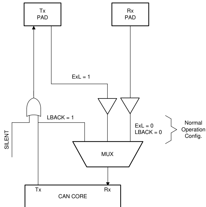
Figure 30-2. CAN_MUX
